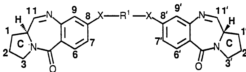
(I)
