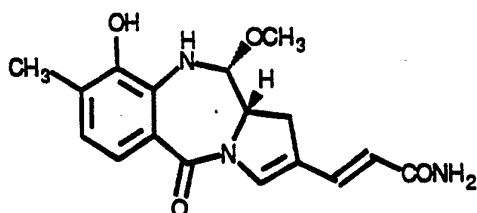
ANTHRAMYCIN
