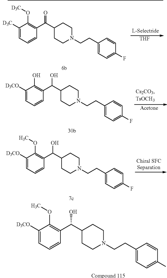
Scheme 7. Preparation of (R)-(1-(4-fluorophenethyl)piperidin-4-yl)(2-methoxy-3-(methoxy-d 3 )phenyl)methanol (Compound 115).
