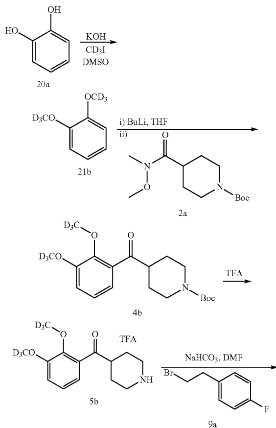
Scheme 6. Preparation of (R)-(2,3-bis(methoxy-d 3 )phenyl)(1-(4-fluorophenethyl)piperidin-4-yl)methanol (Compound 147).
