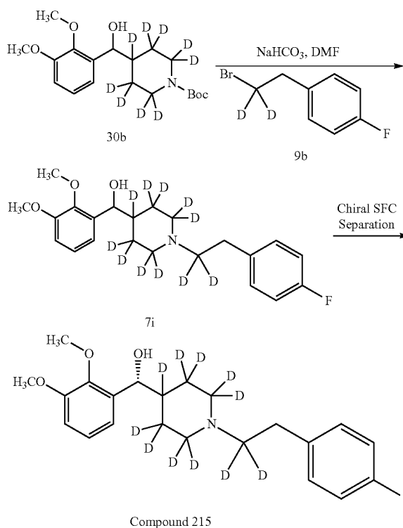
Scheme 16. Preparation of (R)-(2,3-dimethoxyphenyl)(1-(2-(4-fluorophenyl)ethyl-1,1- \text{d}_2 )piperidin-4-yl-2,2,3,3,4,5,5,6,6- \text{d}_9 )methanol (Compound 215).
