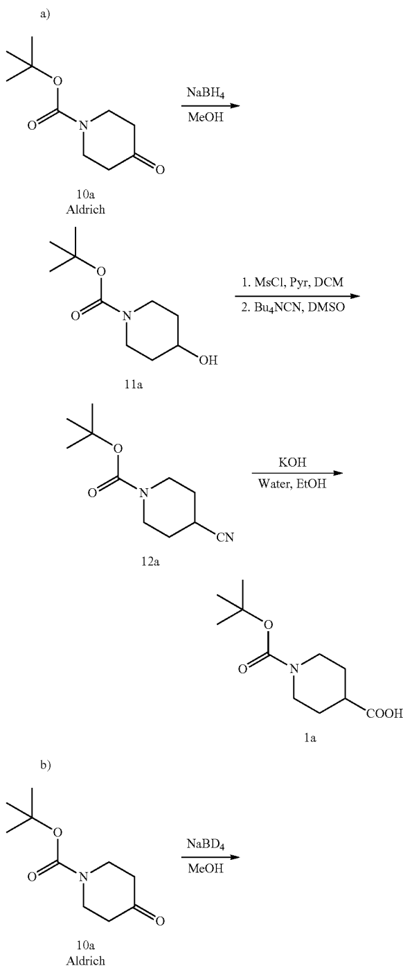
Scheme 2. Synthesis of Intermediates 1a-1h
