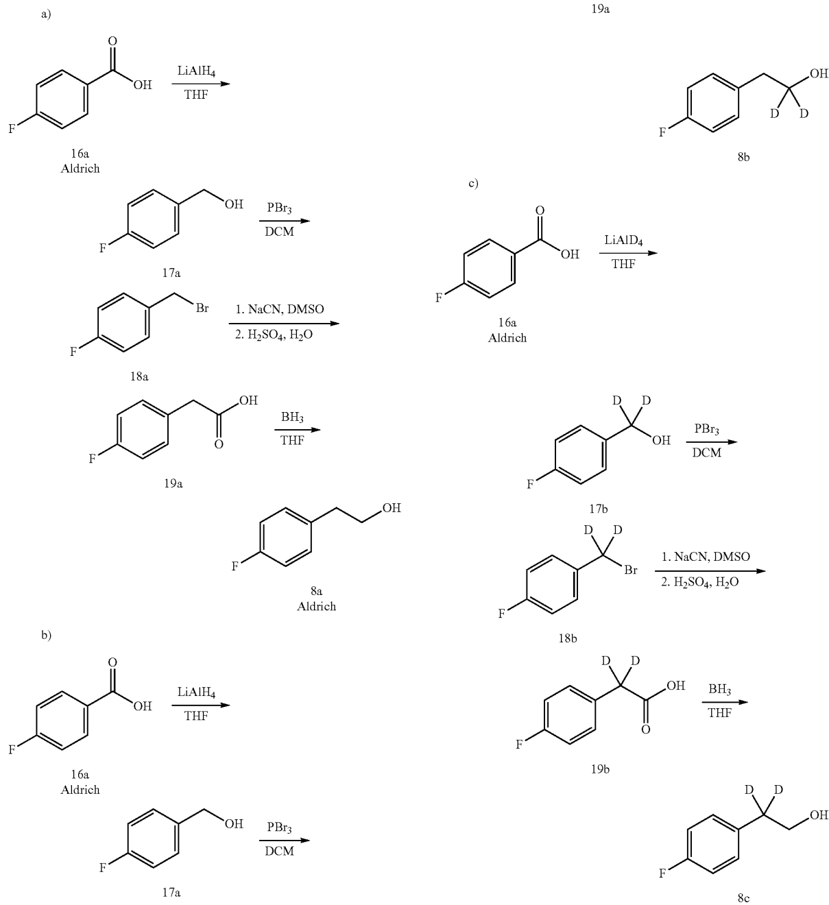
Scheme 4. Synthesis of Intermediates 8a-8h
