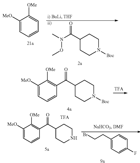
Scheme 9. Preparation of (R)-(1-(4-fluorophenethyl)piperidin-4-yl)(3-methoxy-2-(methoxy-d 3 )phenyl)methanol (Compound 131).
