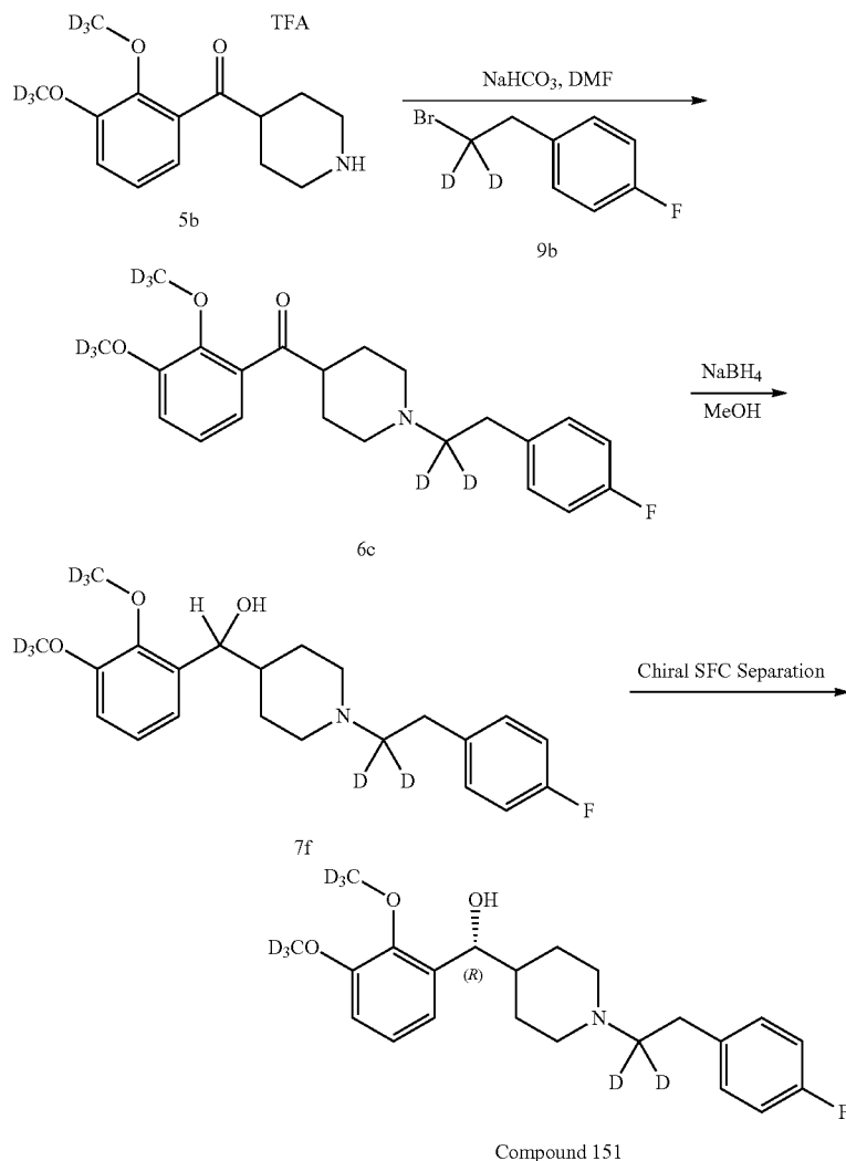
Scheme 11. Preparation of (R)-(2,3-bis(methoxy-d 3 )phenyl)(1-(2-(4-fluorophenyl)ethyl)-1,1-d 2 )piperidin-4-yl)methanol (Compound 151).
