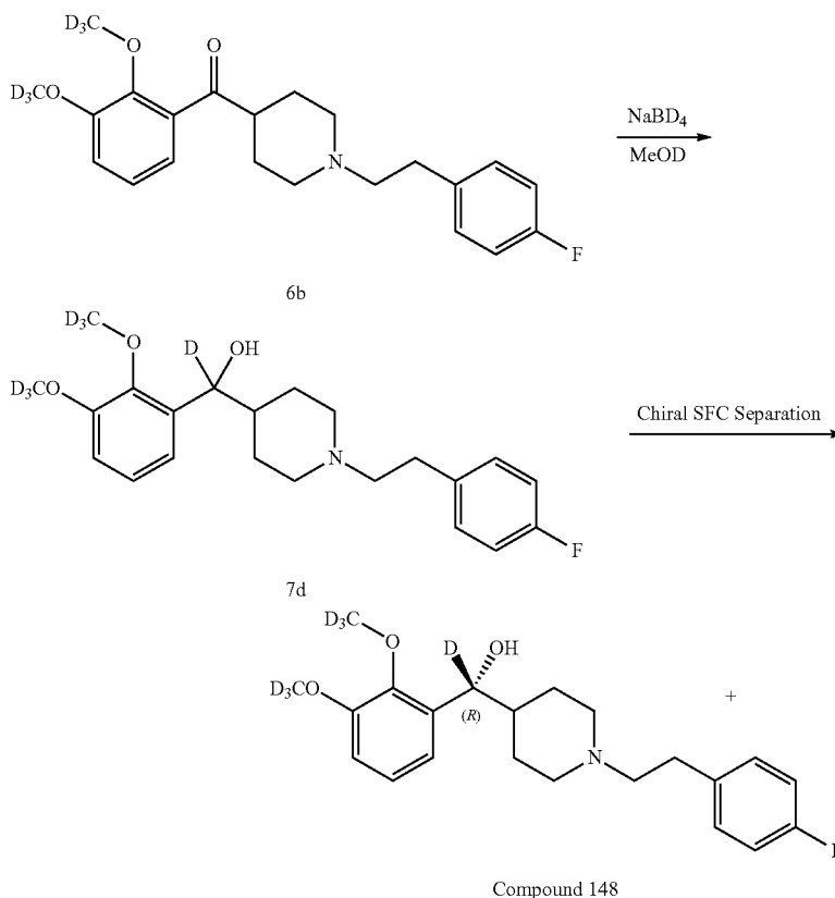
Scheme 8. Preparation of (R)-(2,3-bis(methoxy- \text{d}_3 )phenyl)(1-(4-fluorophenethyl)piperidin-4-yl)methan-d-ol (Compound 148).
