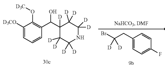
Scheme 18. Preparation of (R)-(2,3-bis(methoxy-d 3 )phenyl)(1-(2-(4-fluorophenyl)ethyl)-1,1-d 2 )piperidin-4-yl-2,2,3,3,4,5,5,6,6-d 9 )methanol (Compound 359).
