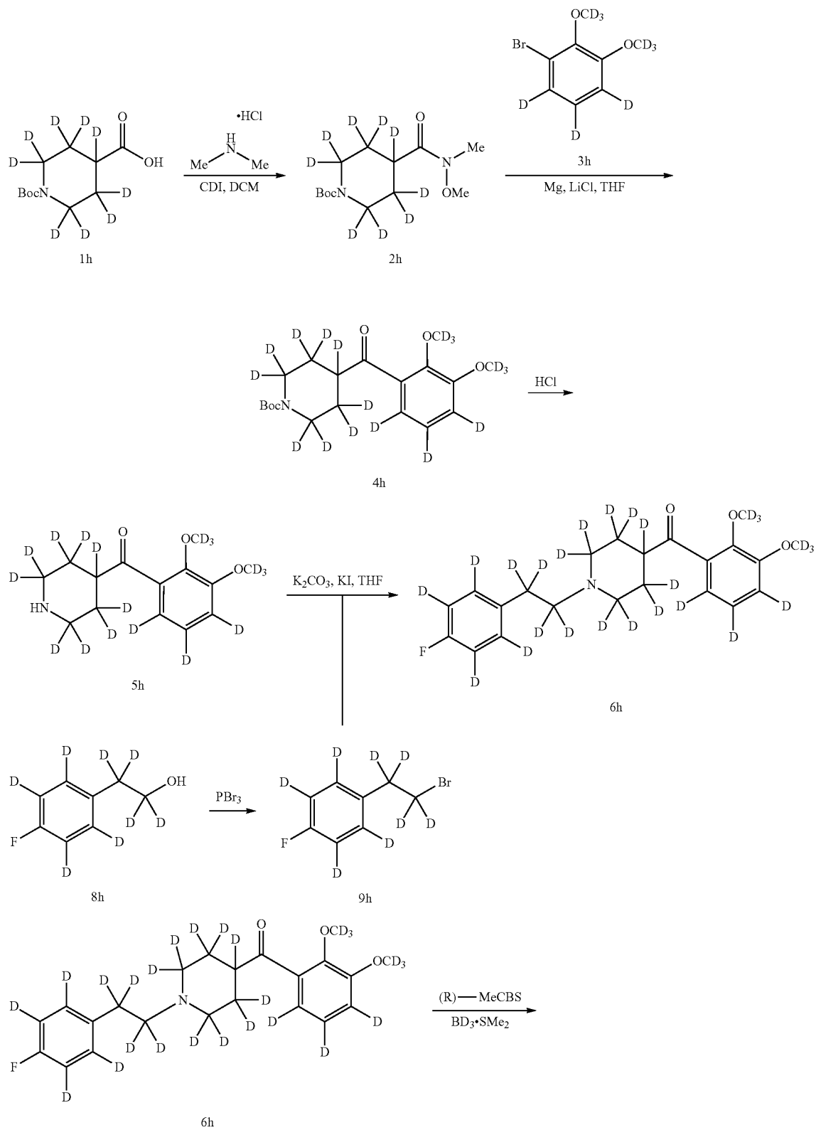
Scheme 5. Representative Synthesis of d 27 -Volinanserin (7h)
