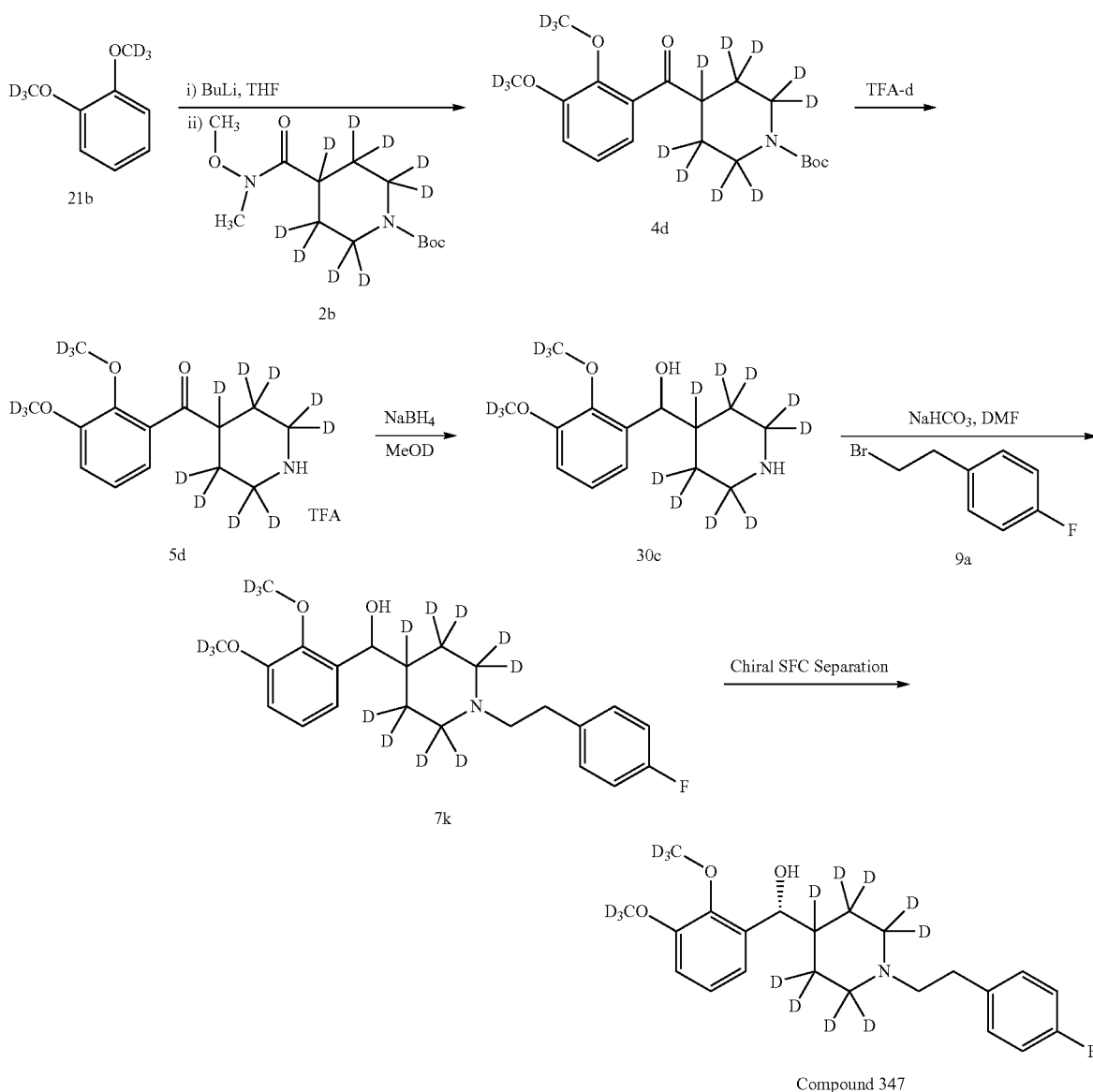
Scheme 17. Preparation of (R)-(2,3-bis(methoxy-d 3 )phenyl)(1-(4-fluorophenethyl)piperidin-4-yl-2,2,3,3,4,5,5,6,6-d 9 )methanol (Compound 347).
