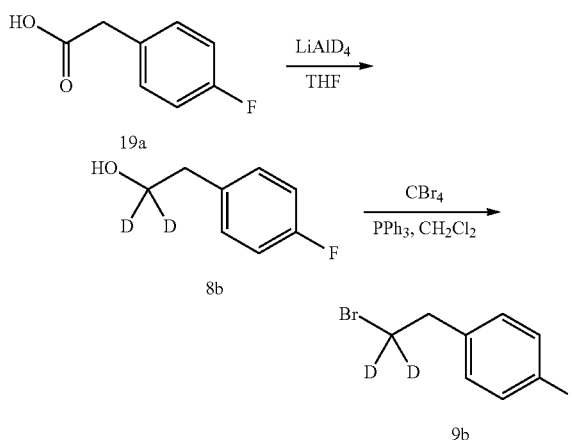
Scheme 10. Preparation of 1-(2-bromoethyl-2,2-d 2 )-4-fluorobenzene (9b)
