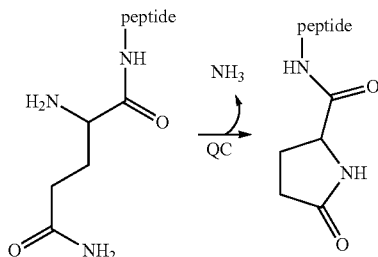
Scheme 1: Cyclization of glutamine by QC
