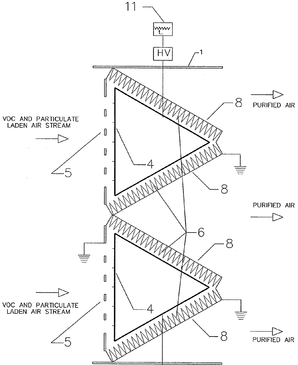
FIG. 6 TOP VIEW OF V-CELL FILTER
