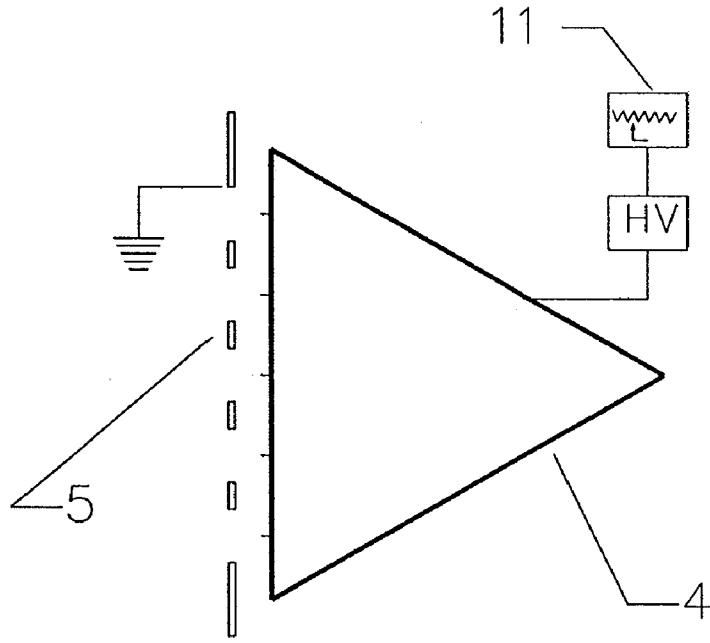
FIG. 7A: TOP VIEW OF ENERGIZING ELECTRODE
