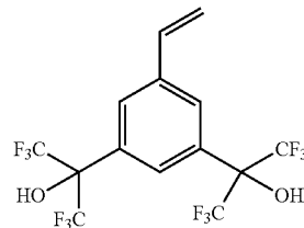
3,5-HFA-St
