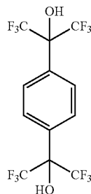
1,4-HFAB
