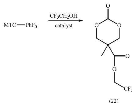
Scheme 3.
