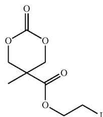
(MTCOEtl)
