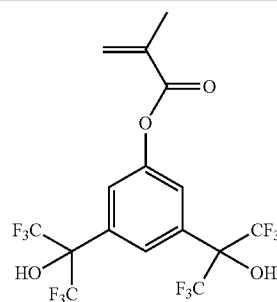
3,5-HFA-MA
