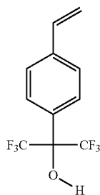
4-HFA-St
