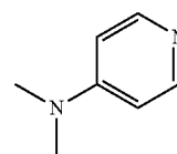
4-N,N-Dimethylaminopyridine (DMAP)
