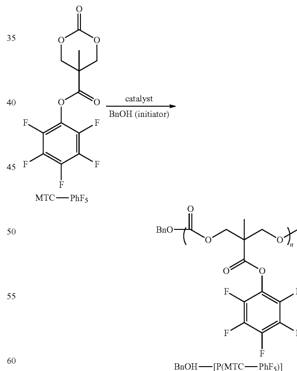
Scheme C.
