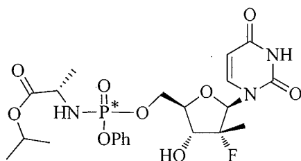
PSI-7977 (Sp-diastereomer) PSI-7976 (Rp-diastereomer)
