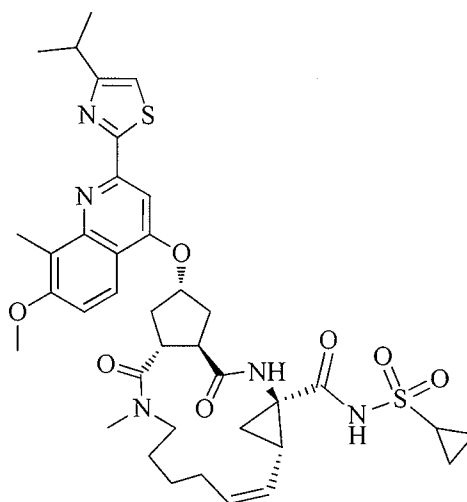
TMC435
