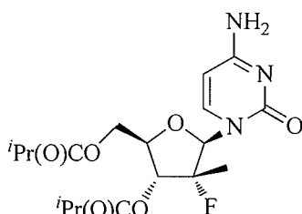
RG7128
