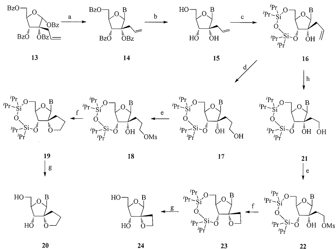
Scheme 2. General Synthesis of 2'-Spiro-ribo-nucleosides
