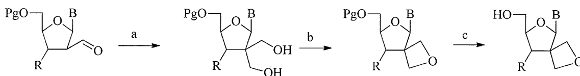
Scheme 4: Reagents: a) 1. \text{HCHO}/\text{NaOH} , 2. \text{NaBH}_4 ; b) Mitsunobu reagents; c) deprotection.
