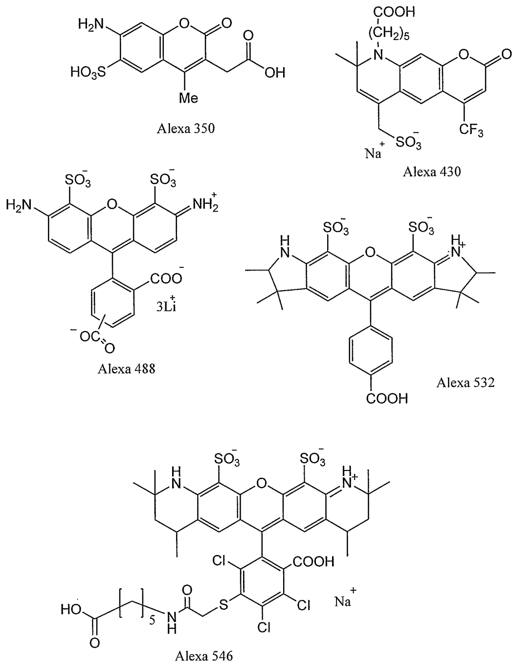
Figure 1. Alexa Fluor® 350, 430, 488, 532 and 546 dyes. (Prior Art)
