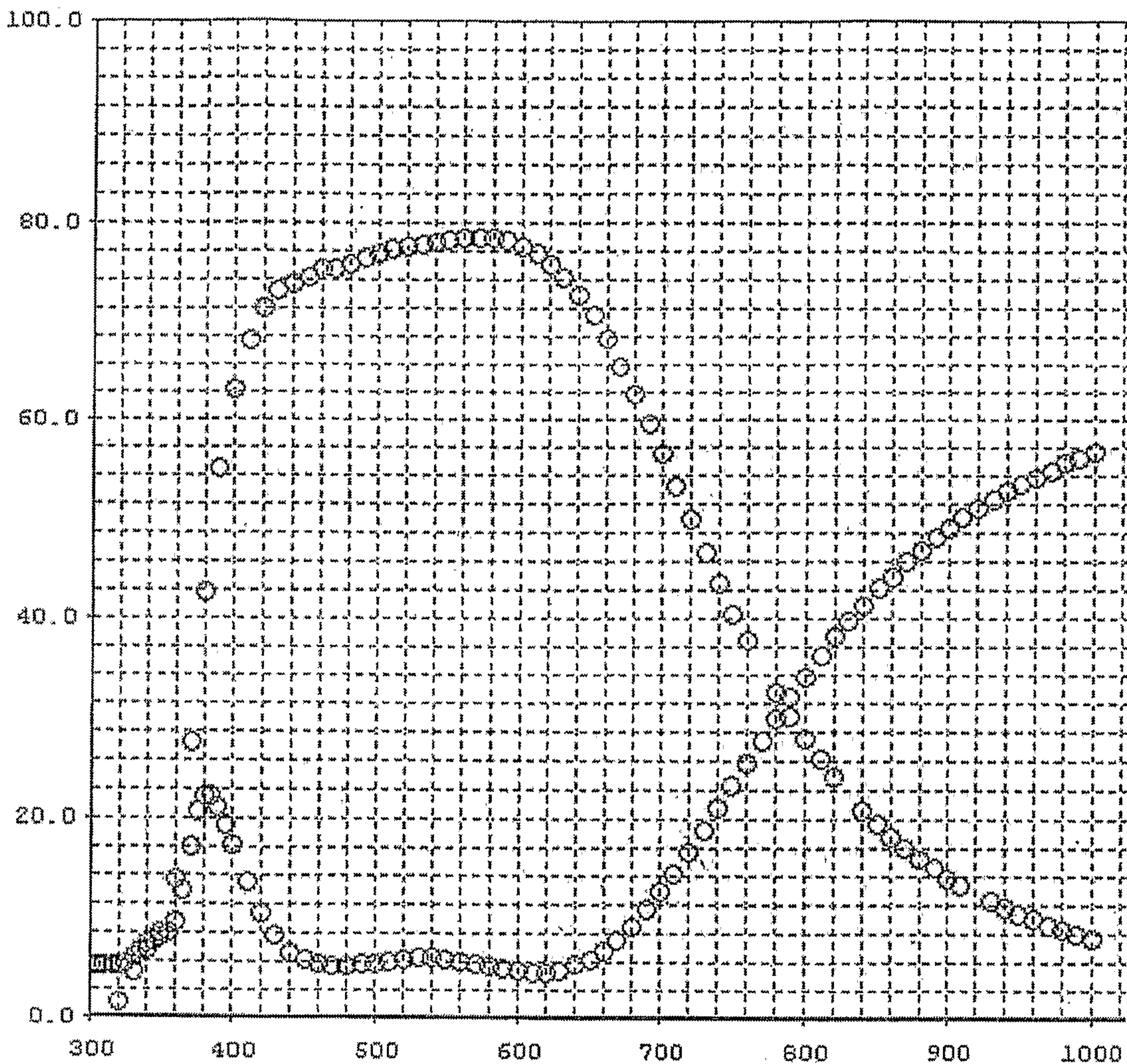
Reflectance (%) and Transmittance (%) vs Wavelength
