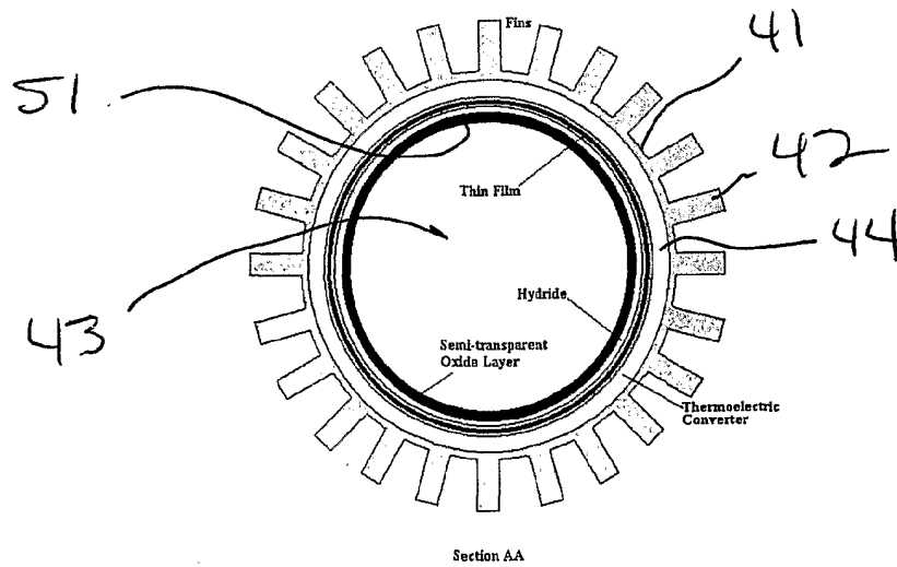
Figure 1. Schematic of Proton-Reaction Palm Power Cell
