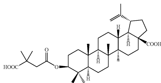
Structure of 3-O-(3',3'-dimethylsuccinyl) betulinic acid (DSB)
