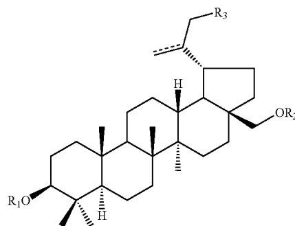
Betulin and Dihydrobetulin Derivatives
