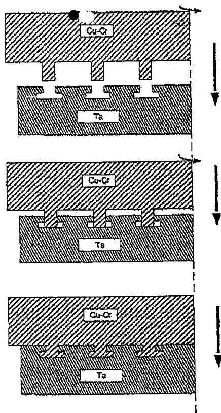
Friction weld interlocking target assembly method.
