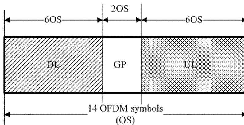
Configuration 1 of Type 1 enhanced subframe DL=UL
