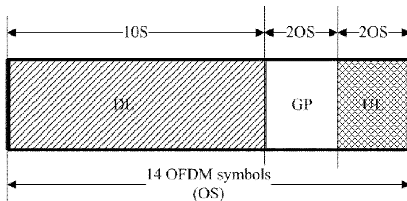
Configuration 2 of Type 1 enhanced subframe DL > UL
