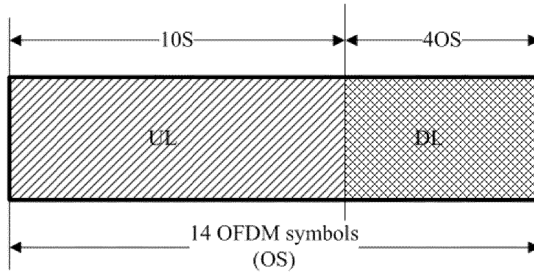
Configuration 2 of Type 2 enhanced subframe UL>DL
