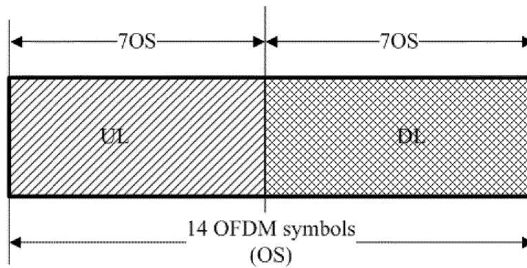
Configuration 1 of Type 2 enhanced subframe DL = UL
