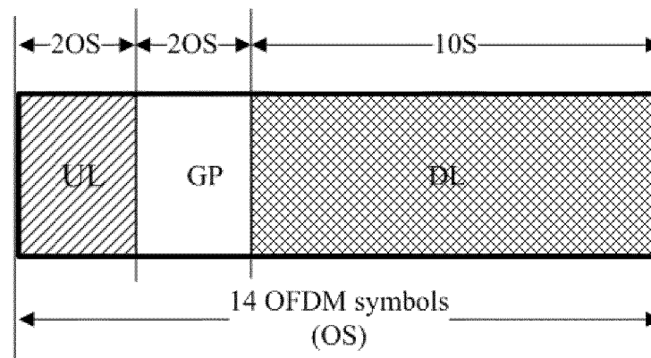
Configuration 3 of Type 2 enhanced subframe UL < DL
