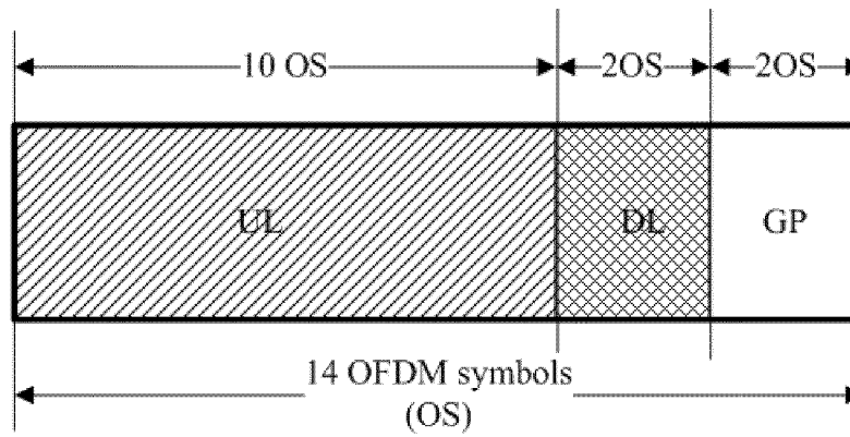
Configuration 2 of Type 2 enhanced subframe UL>UL
