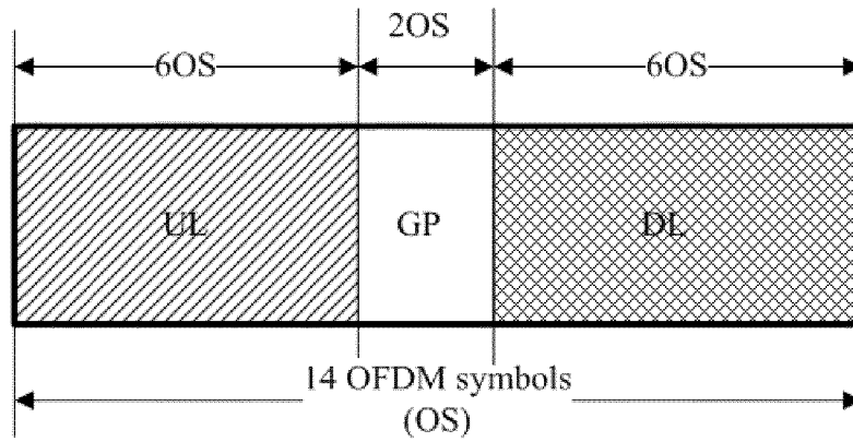
Configuration 1 of Type 2 enhanced subframe DL=UL
