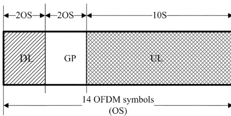
Configuration 3 of Type 1 enhanced subframe DL < UL
