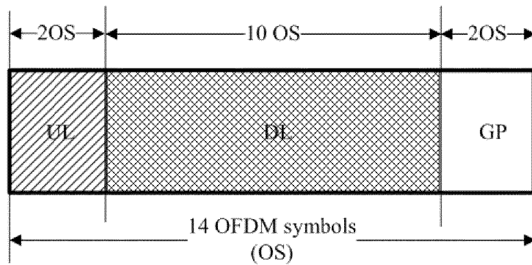
Configuration 3 of Type 2 enhanced subframe UL<DL
