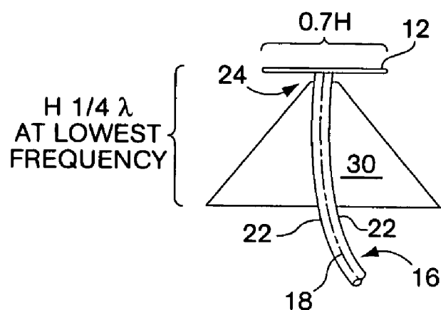
Fig. 1 (PRIOR ART)
