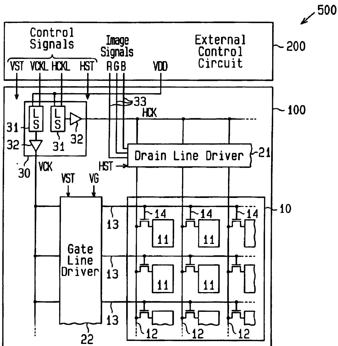
Fig.1 (Prior Art)
