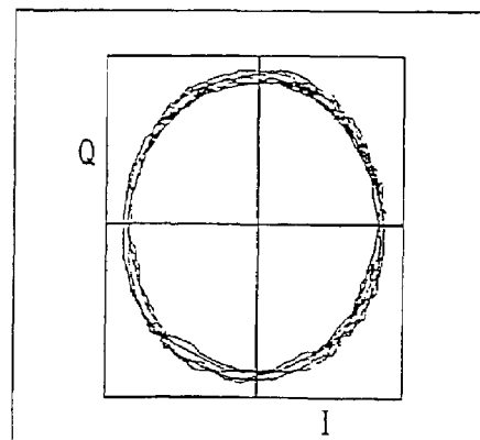
FQPSK-B. VECTOR CONSTELLATION
