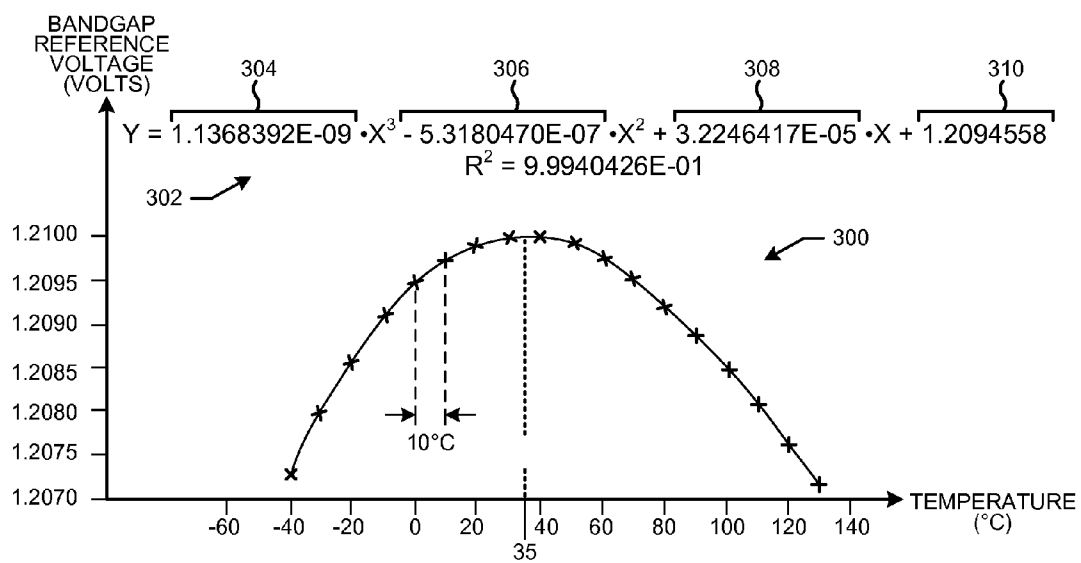
BANDGAP REFERENCE VOLTAGE FIG. 3A
