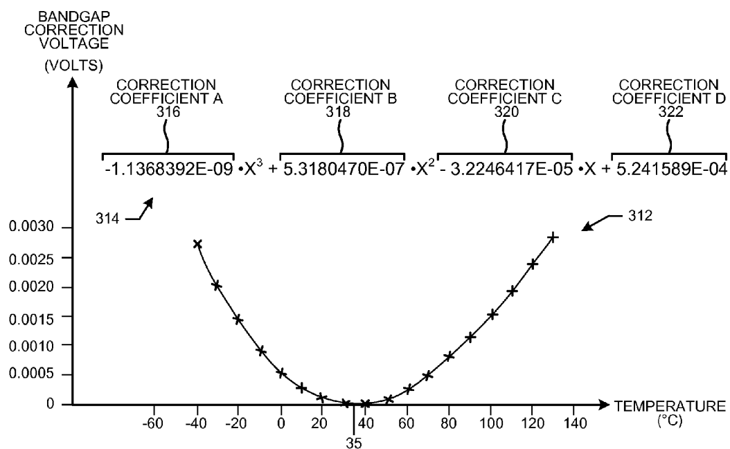
BANDGAP CORRECTION VOLTAGE FIG. 3B
