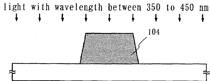
Fig. 1C light irradiation processing
