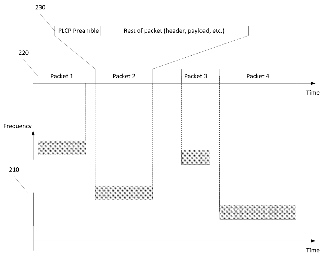
Spectral and temporal characteristics for TF-WB packets.
