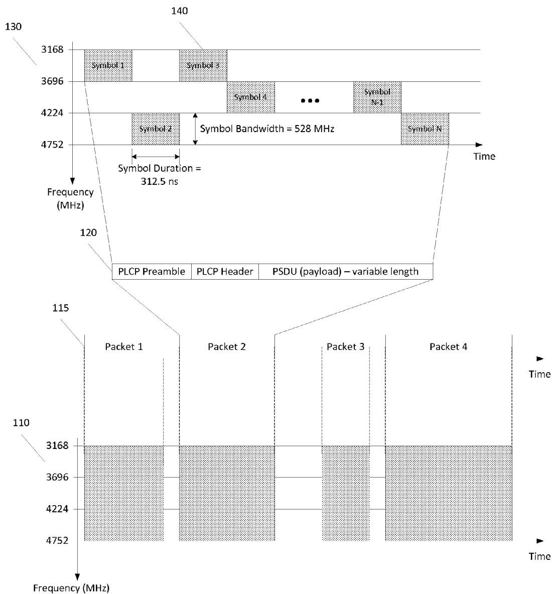
Spectral and temporal characteristics for ECMA-368/MB-OFDM packets.
