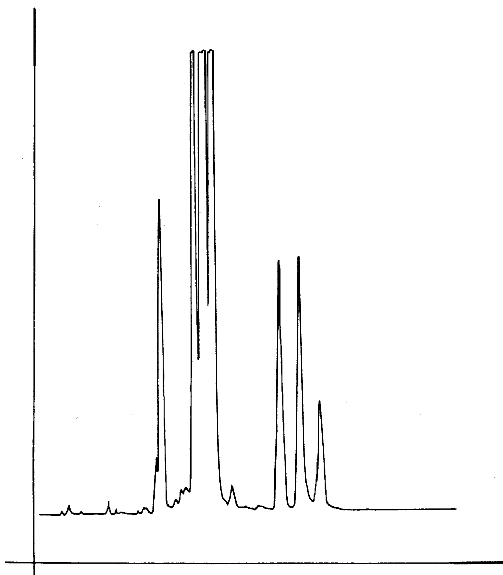
GLC PROFILE FOR EXAMPLE I .
