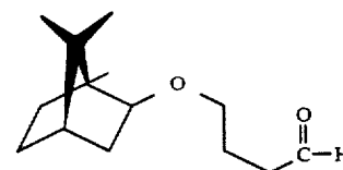
FIG. 15 is the infra-red spectrum for fraction 5 of the distillation product of the reaction product of this example which is for the compound having the structure:
