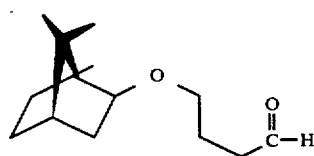
FIG. 12 is the GLC profile for fraction 6 of the distillation product of the reaction product of this example containing the compound having the structure:
