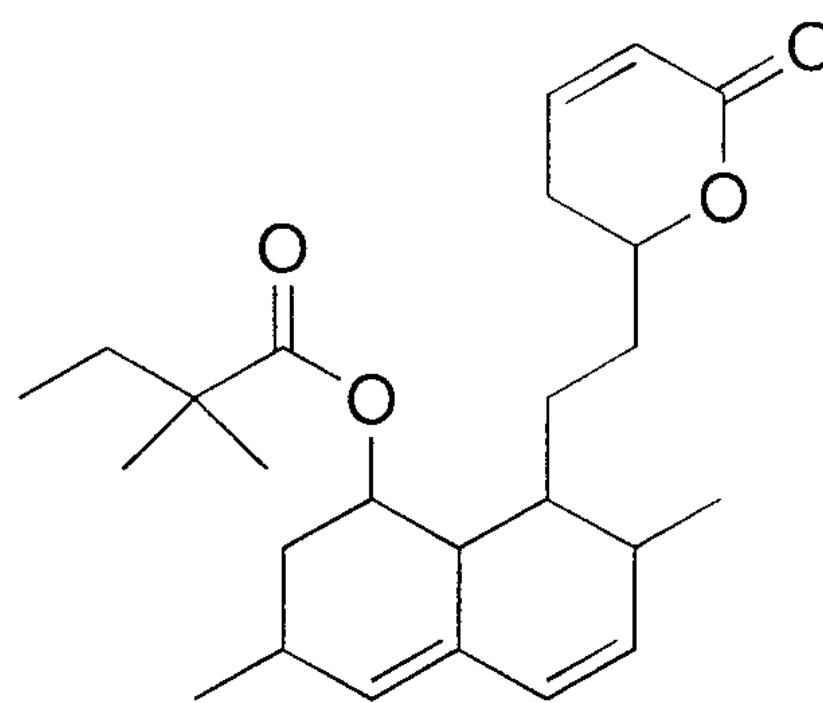
Dehydrosimvastatin (RRT 2.669)
