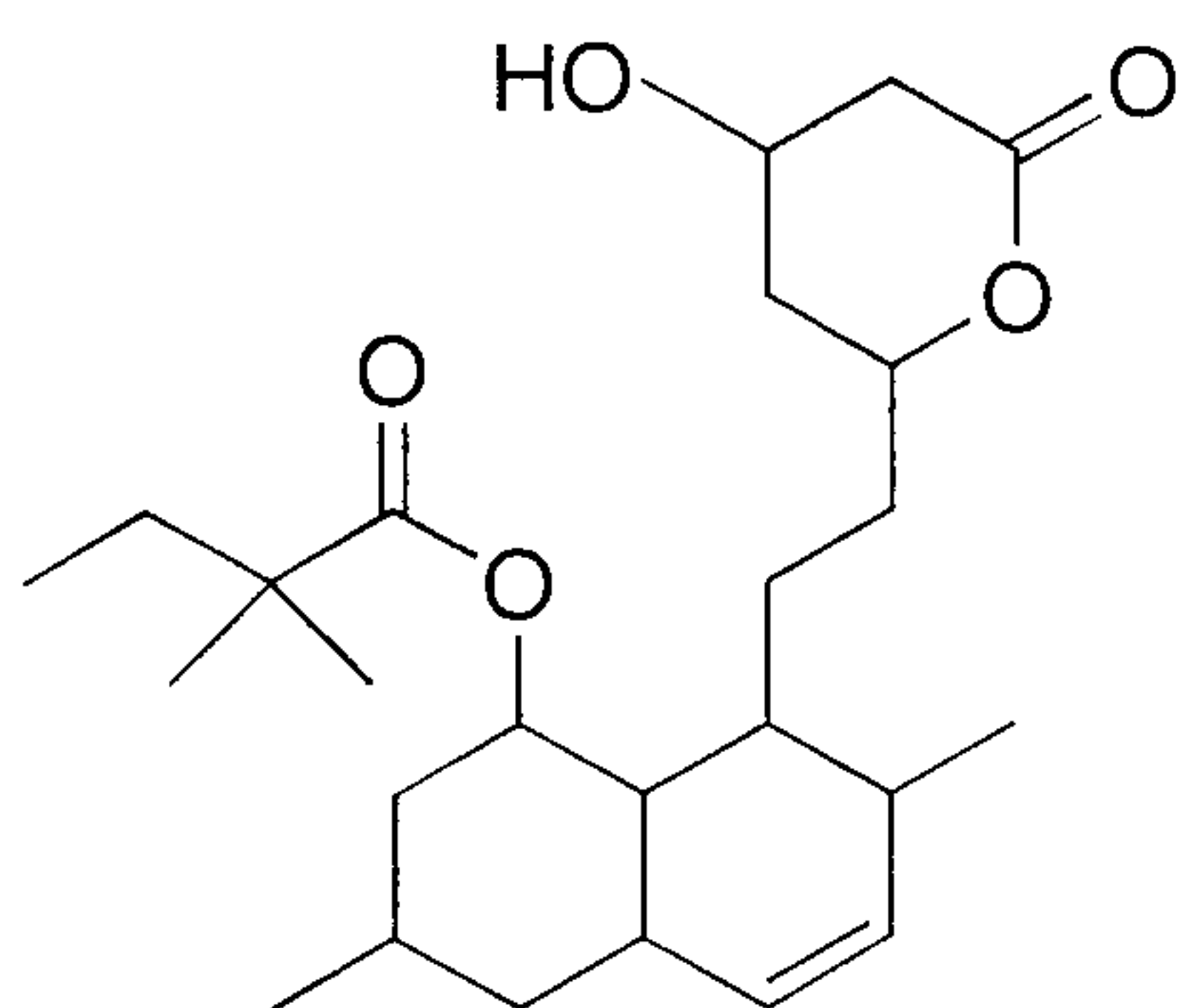
Dihydrosimvastatin (RRT 1.260)
