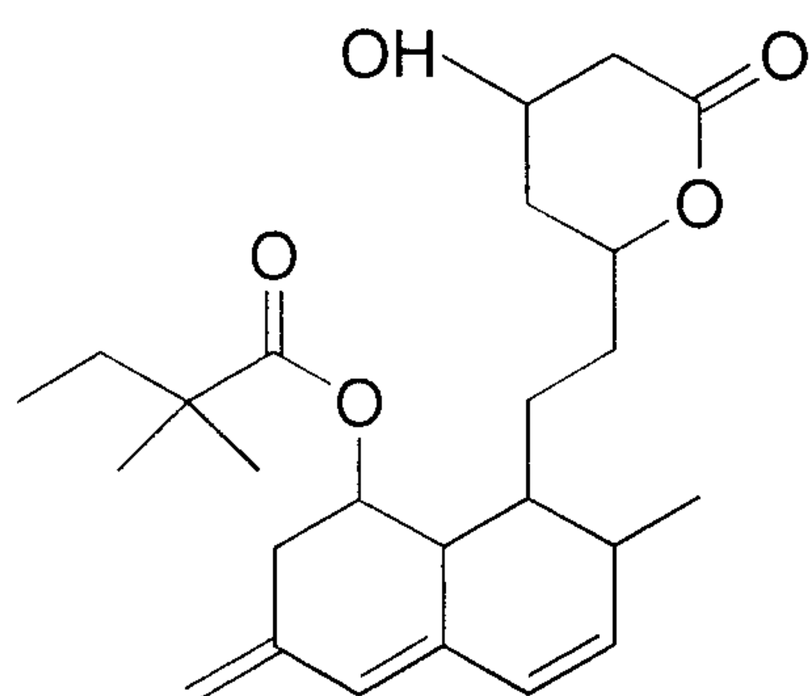
3-Exomethylene Simvastatin (RRT 0.810)
