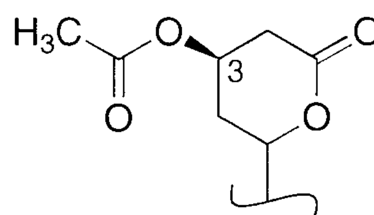
3-O-Acetyl Lactone
