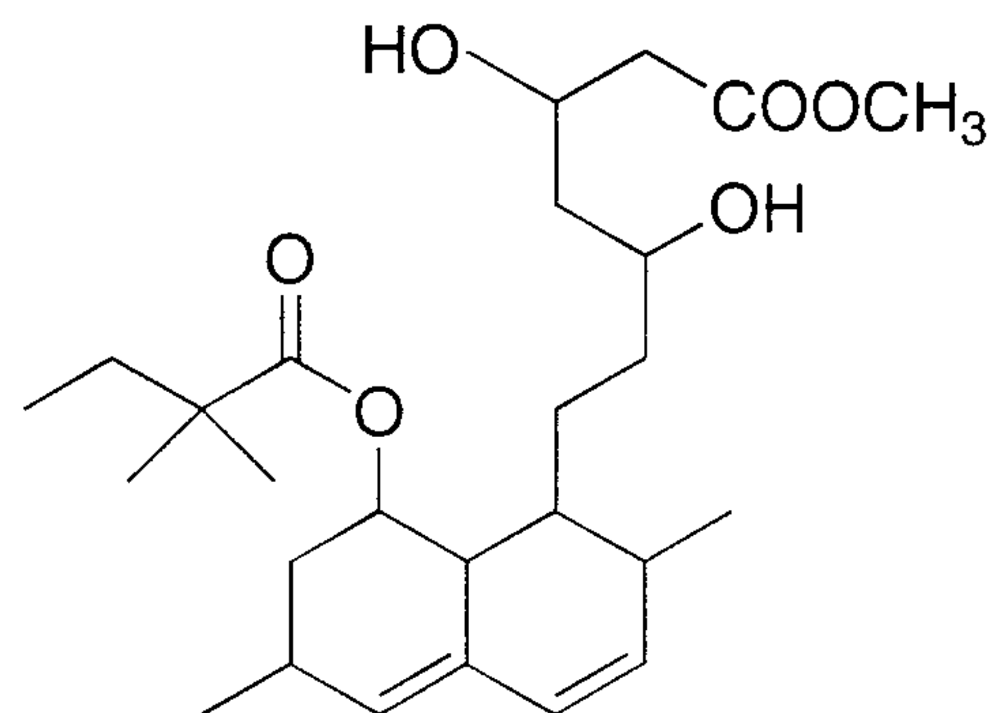
Simvastatin Methyl Ester (RRT 1.100)
