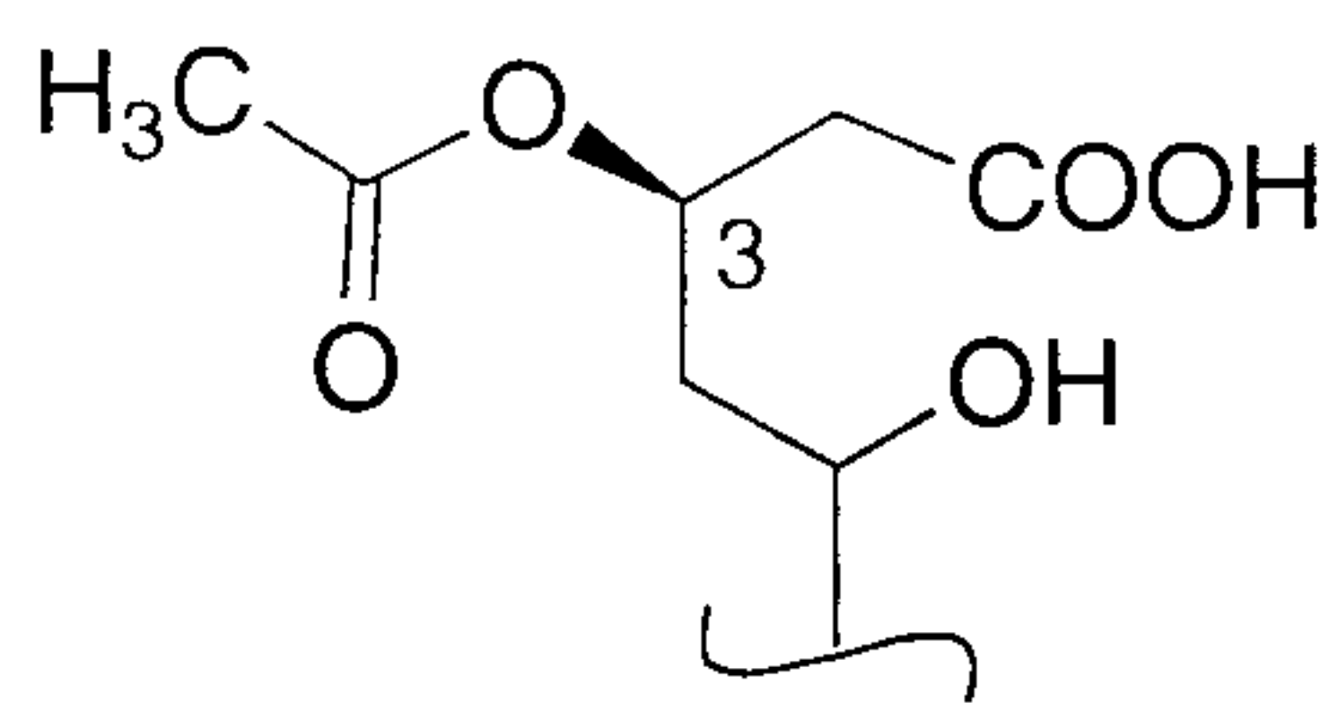
3-O-Acetyl 5-Hydroxy Acid ("open-ring")
