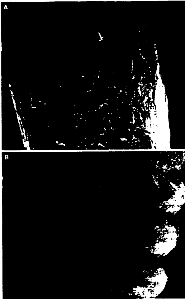
FIGURE 7. Scanning electron micrographs of the surfaces of an ion-implanted, collagen-coated platinum coil (original magnification, \times 200 ) (A) and a standard platinum coil (original magnification, \times 300 ) (B) after 1 hour in swine iliac arteries. Note the intensive blood cellular response on the ion-implanted, protein-coated platinum coil surface.
