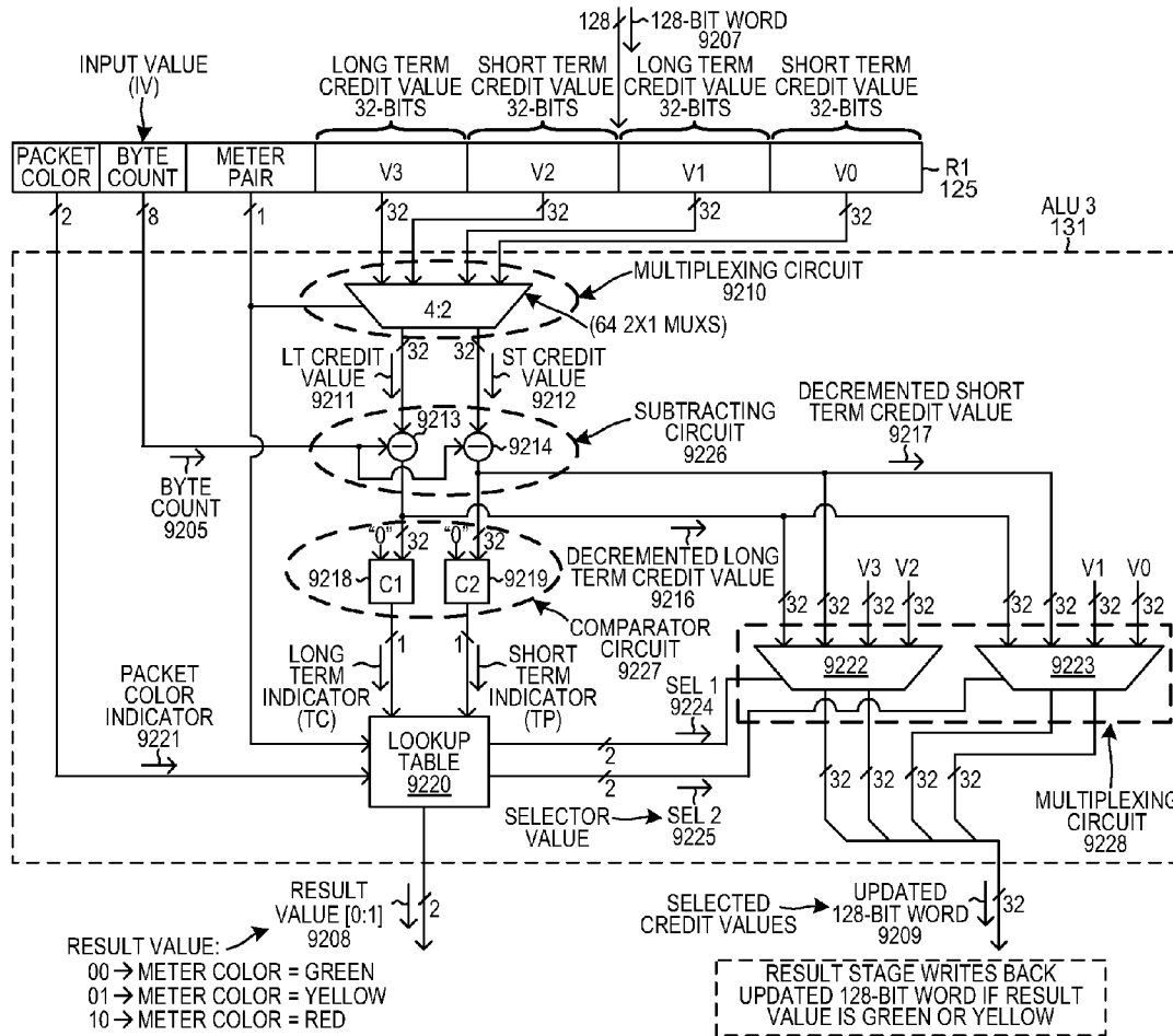
ATOMIC METERING COMMAND LOOKUP STAGE FIG. 59
