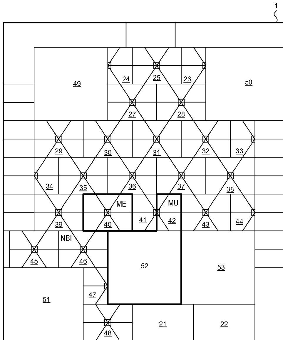
COMMAND-PUSH-PULL (CPP) DATA BUS STRUCTURE
