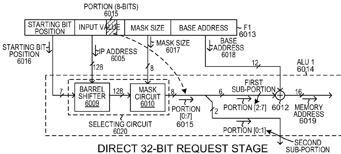
DIRECT 32-BIT MEMORY PACKING SCHEME FIG. 40
