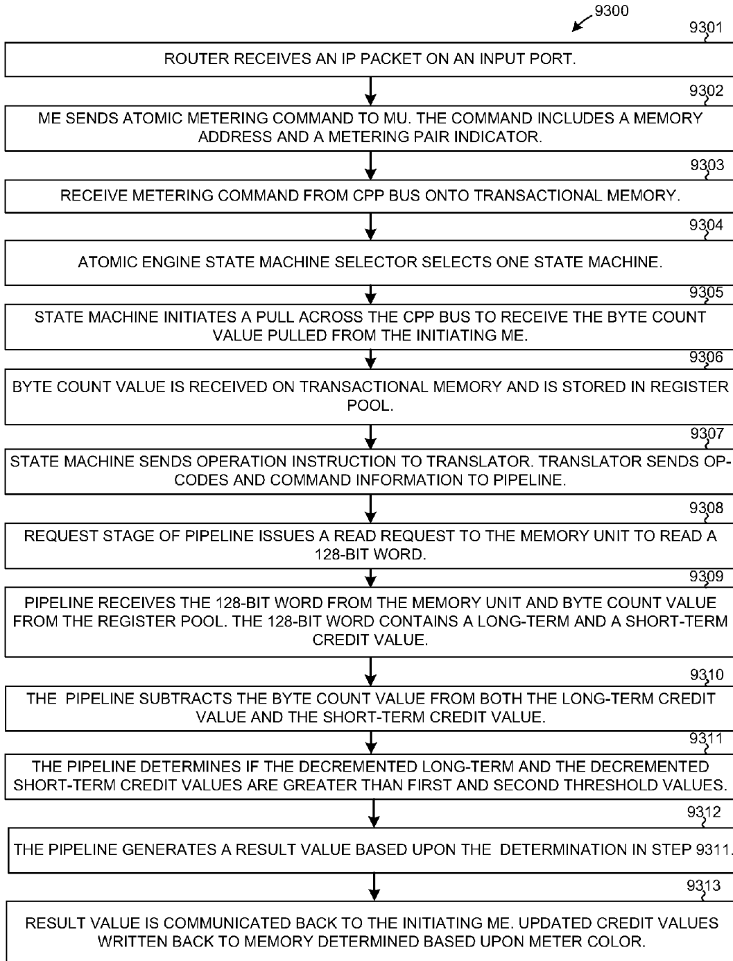
ATOMIC METERING COMMAND FLOWCHART FIG. 62
