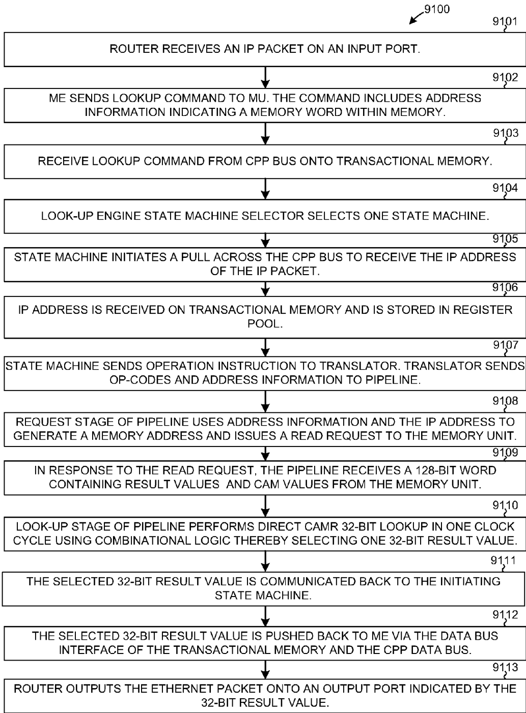
CAMR 32-BIT LOOKUP FLOWCHART FIG. 55
