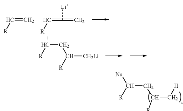
Scheme 4: A hypothetical mechanism for cationic polymerization of [n]2, n = 5-7.
