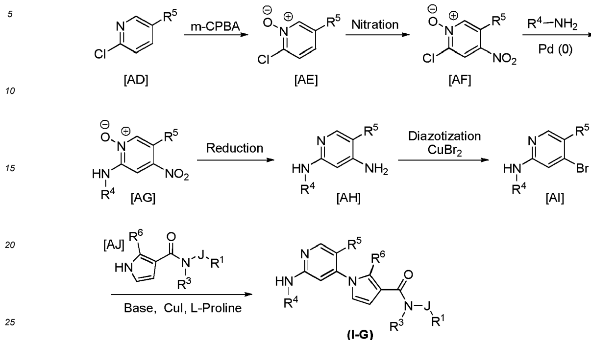
Scheme 8
