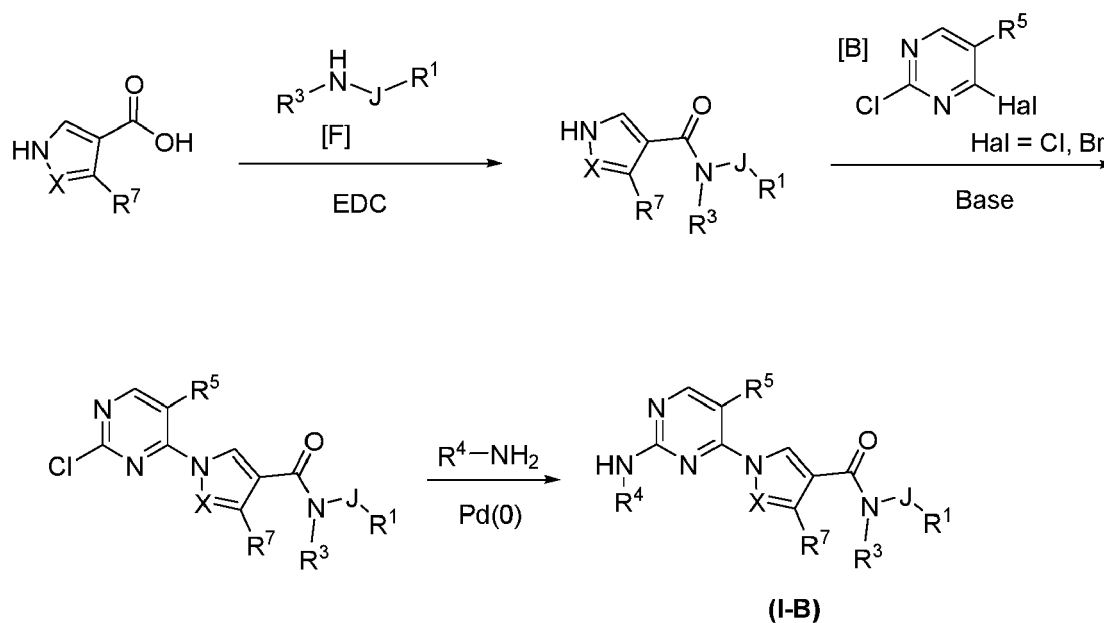
Scheme 3a
