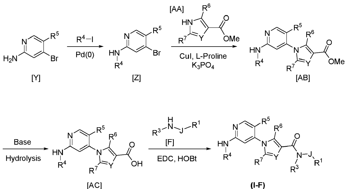
Scheme 7
