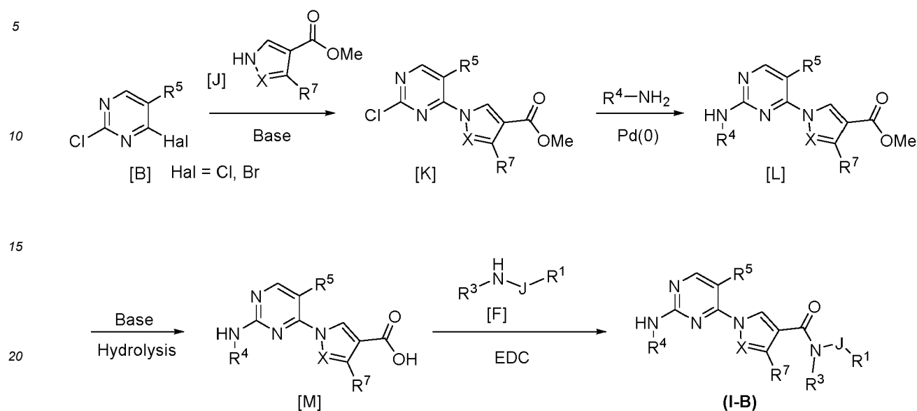
Scheme 3
