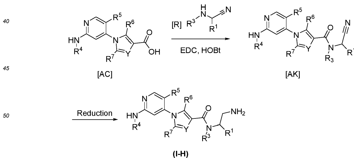
Scheme 9
