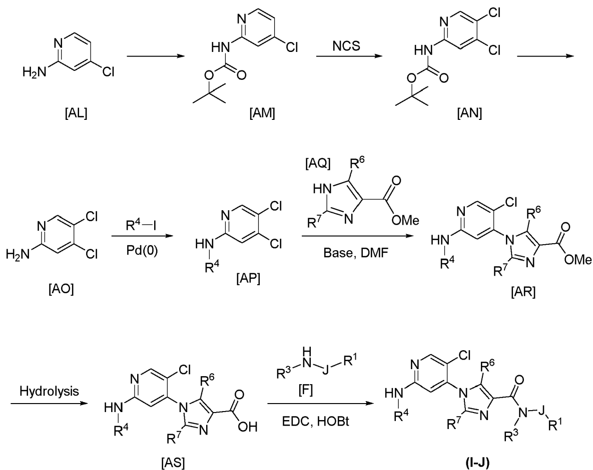
Scheme 10
