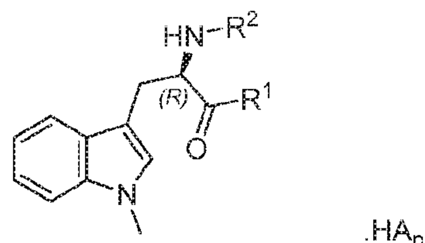
Formula 2
