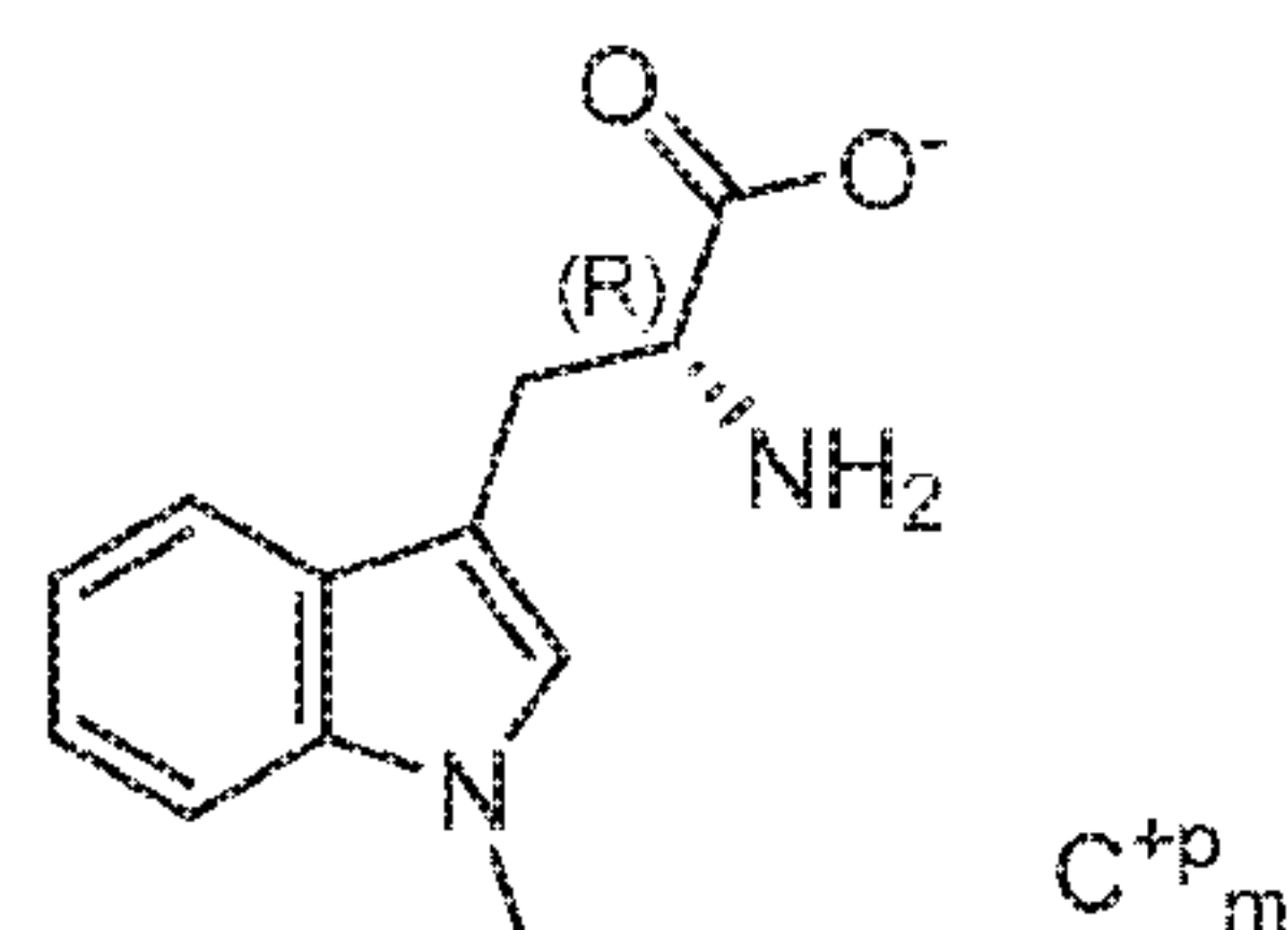
Formula 1b
