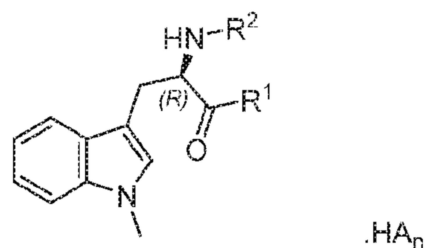
Formula 2
