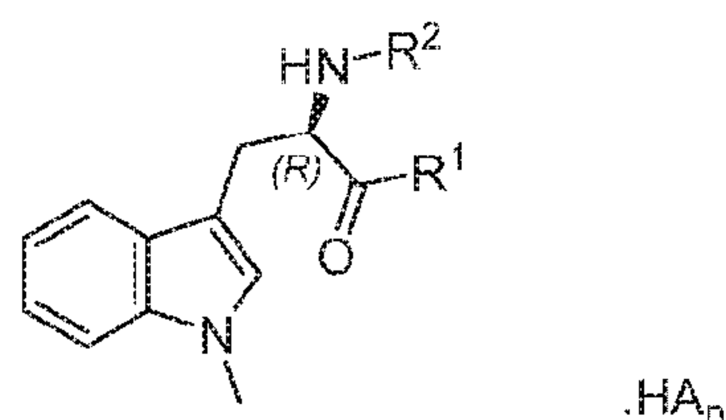
Formula 2
