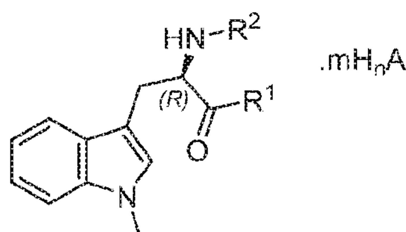
Formula 2
