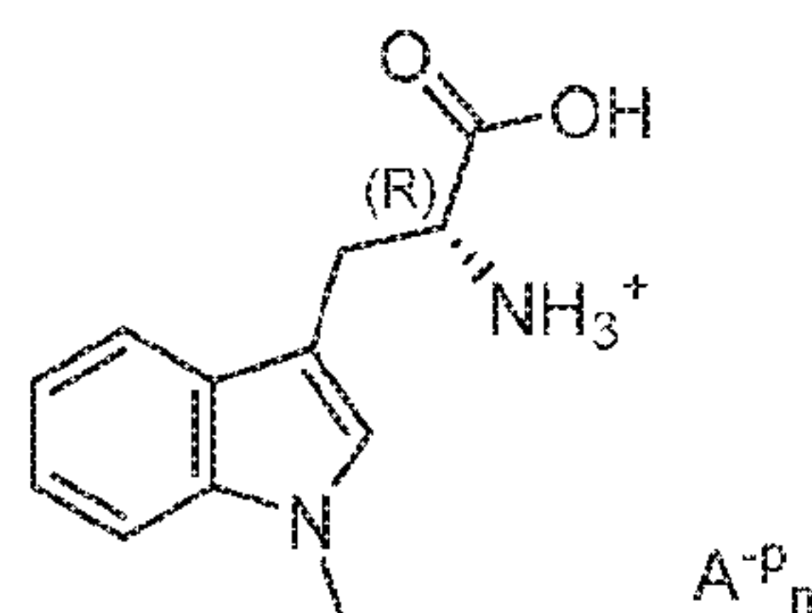
Formula 1a
