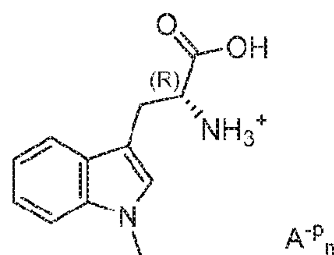
Formula 1a
