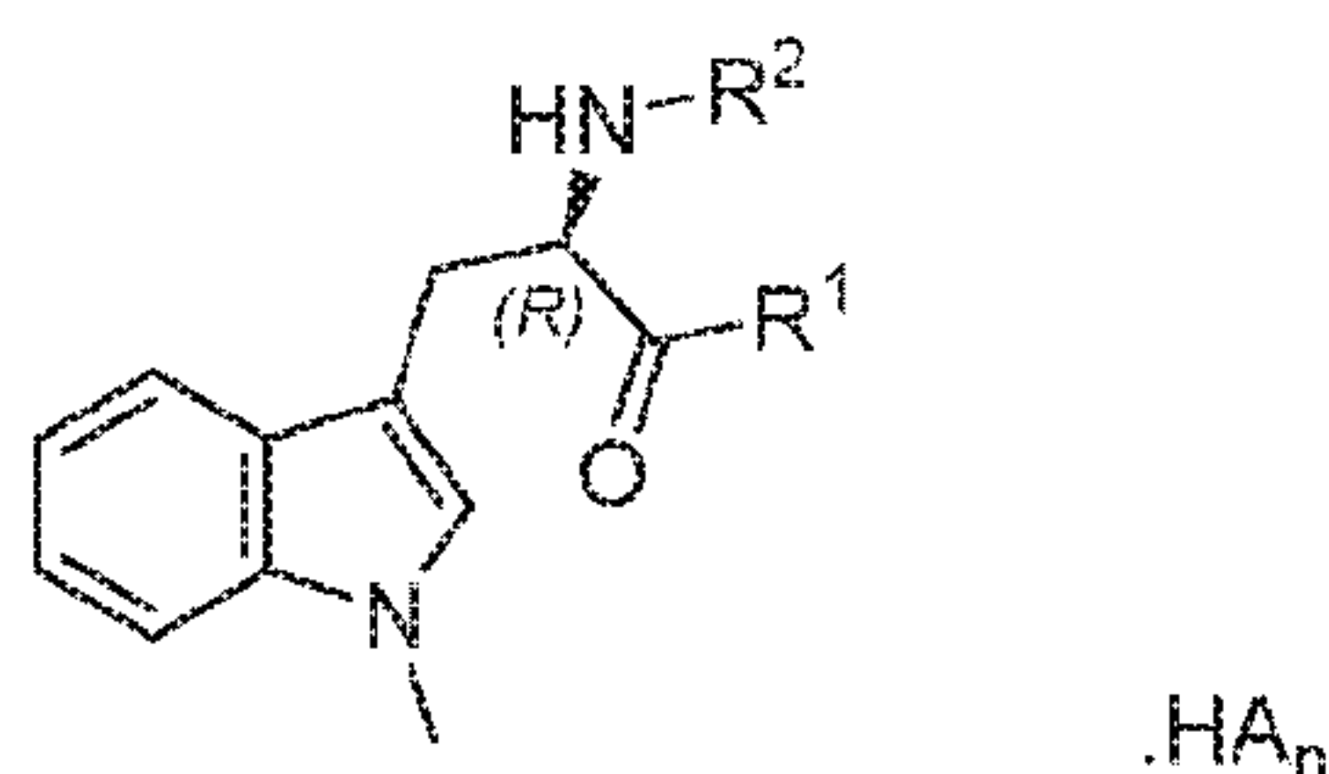
Formula 2
