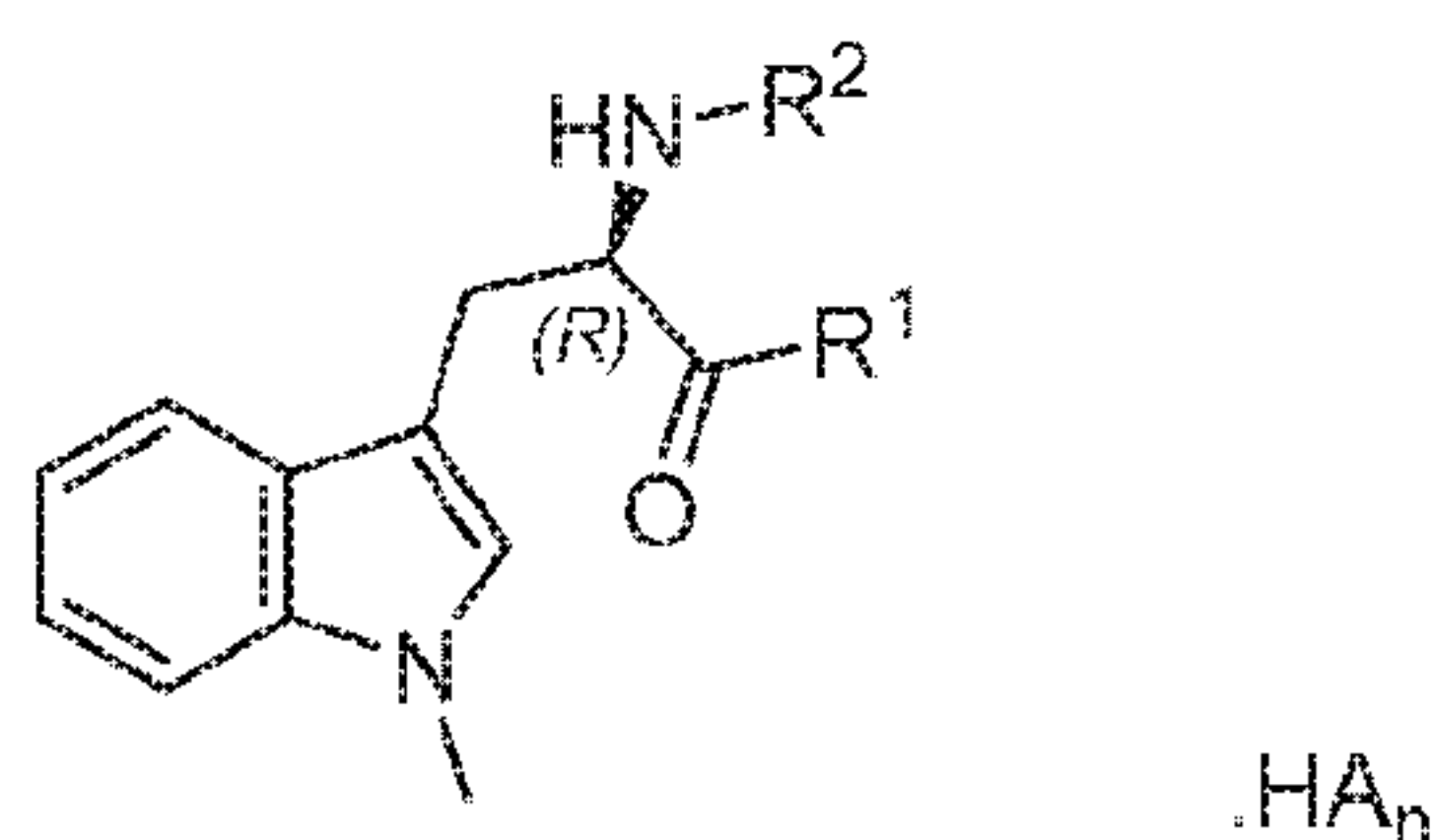
Formula 2
