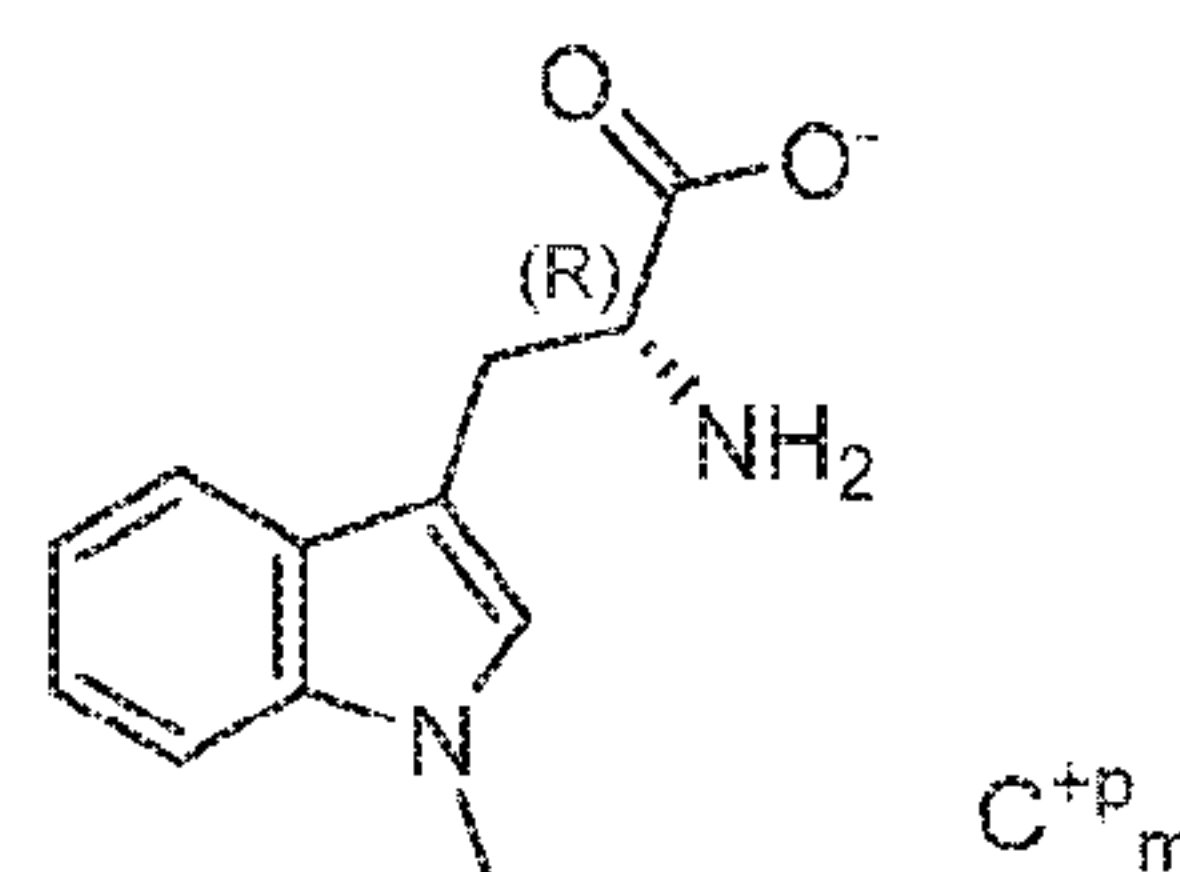
Formula 1b
