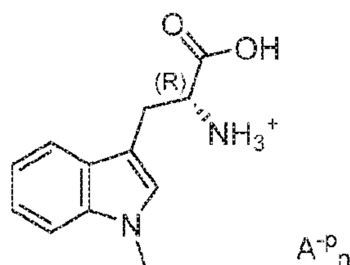
Formula 1a
