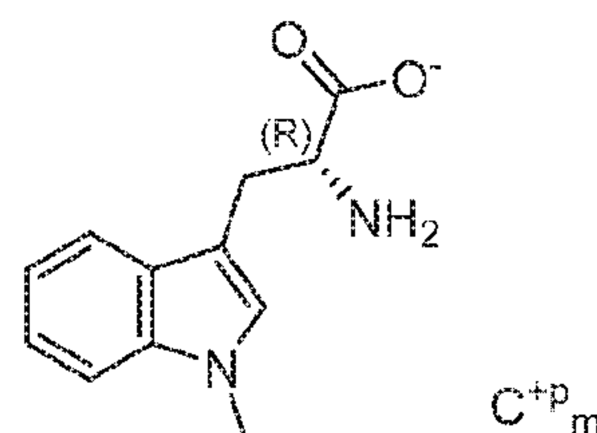
Formula 1b
