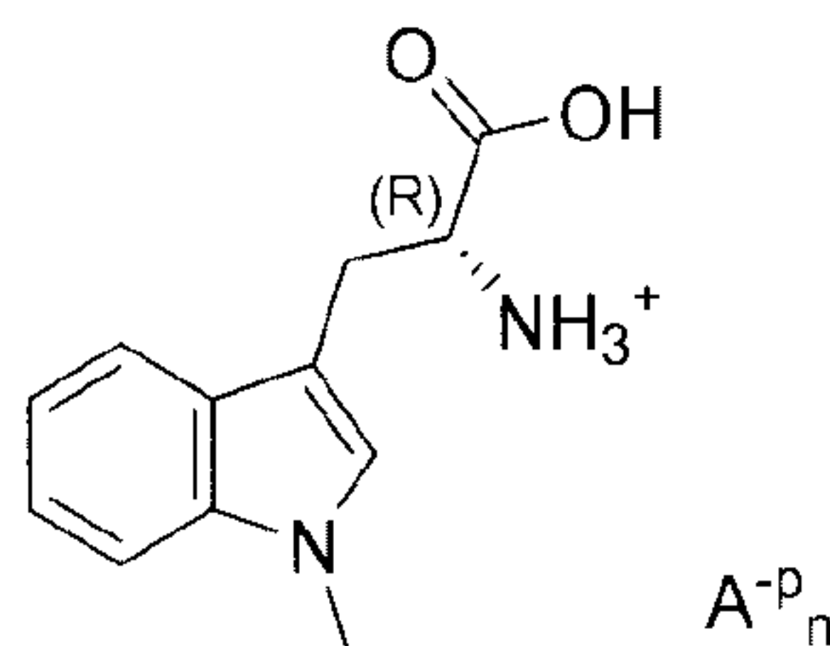
Formula 1a
