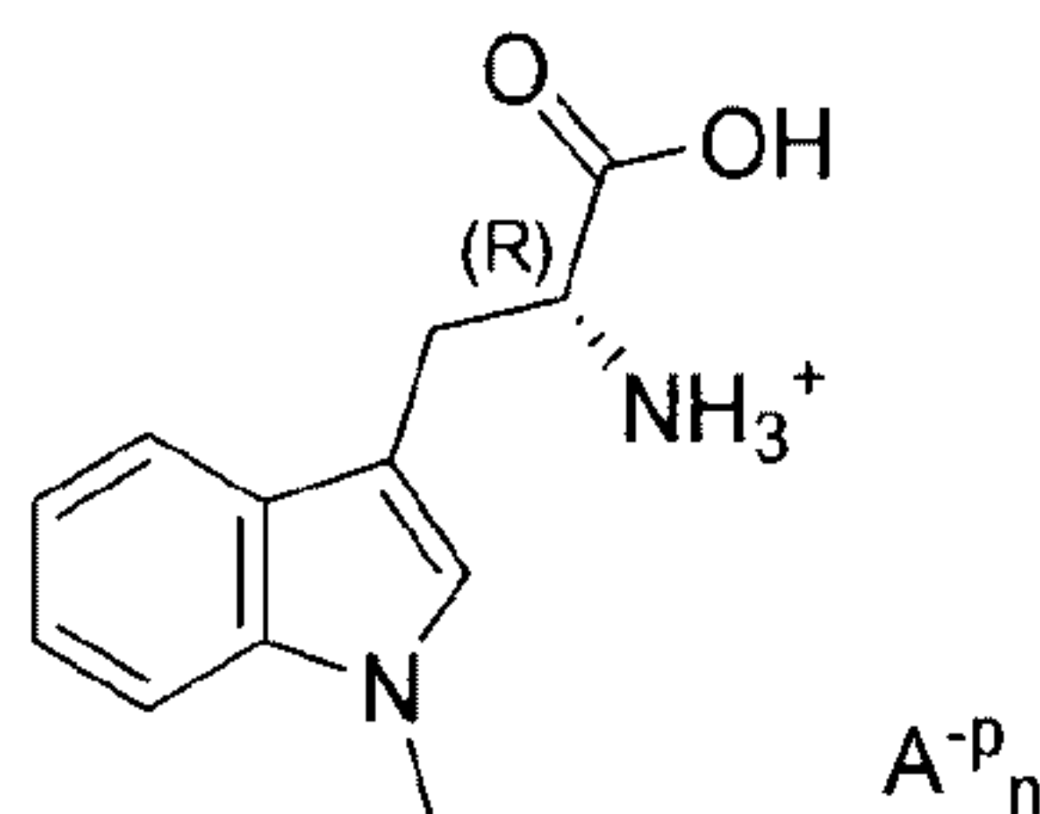
Formula 1a
