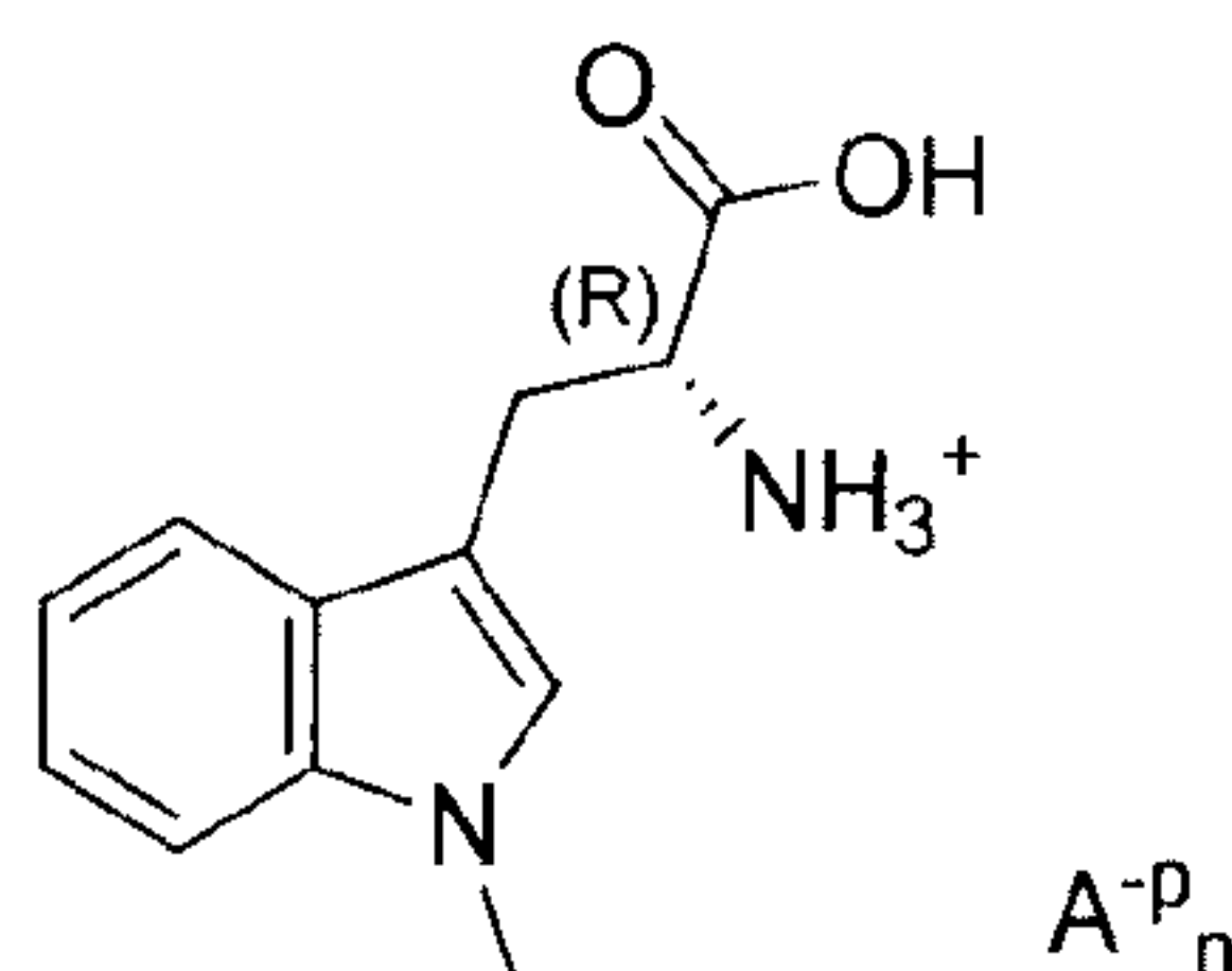
Formula 1a
