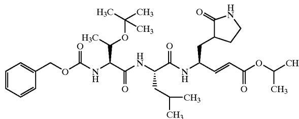
Compound 91
