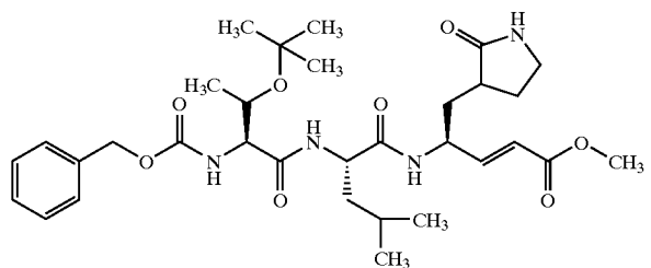
Compound 103
