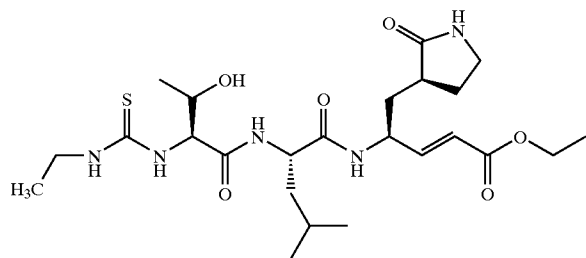
Compound 33
