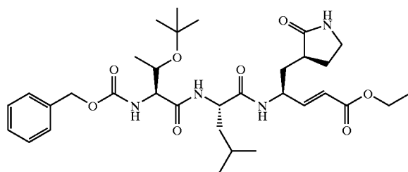
Compound 19
