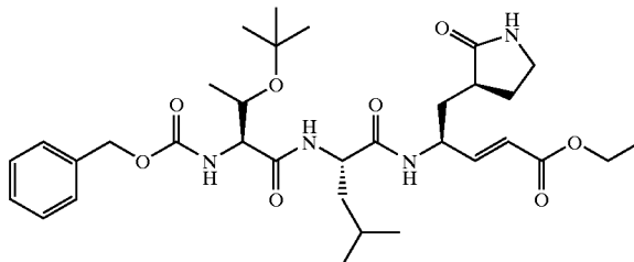
Compound 6
