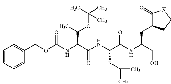
Compound 107
