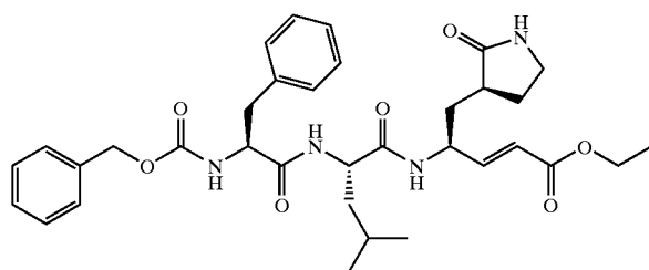
Compound 37
