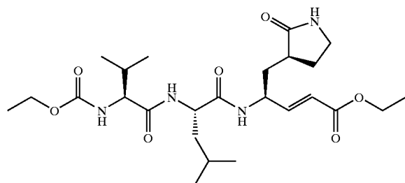
Compound 19
