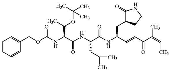
Compound 139
