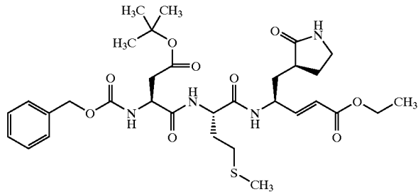
Compound 88
