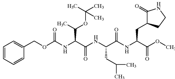
Compound 115
