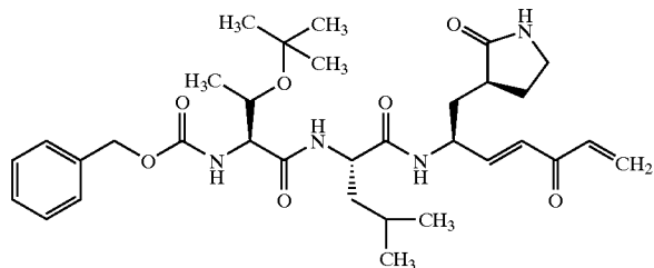
Compound 138
