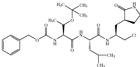
Compound 133
