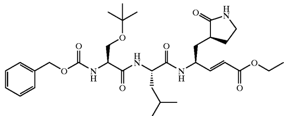
Compound 7
