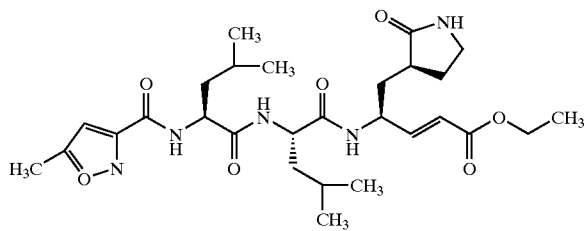
Compound 71
