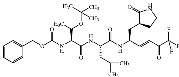
Compound 132
