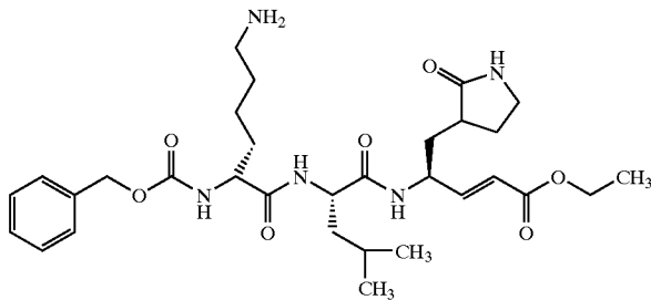
Compound 74
