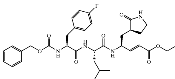
Compound 39
