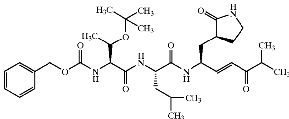
Compound 137
