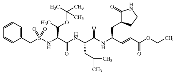
Compound 89
