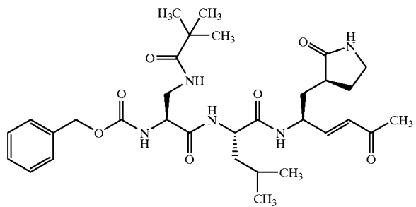
Compound 122
