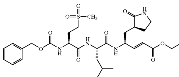
Compound 14
