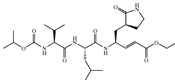
Compound 21
