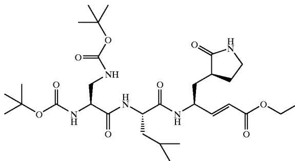
Compound 66
