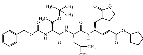
Compound 100
