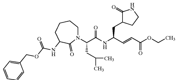
Compound 94
