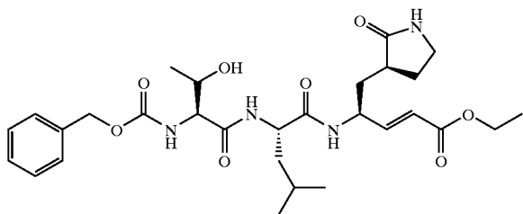
Compound 1
