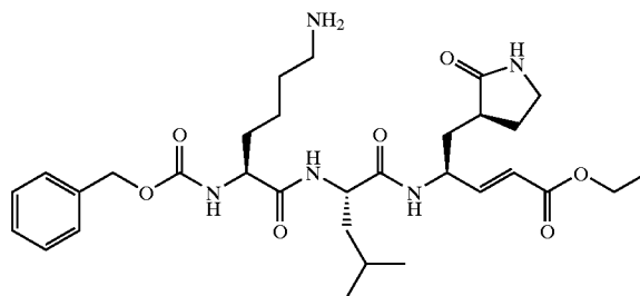
Compound 10
