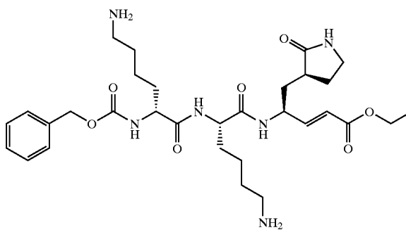
Compound 62
