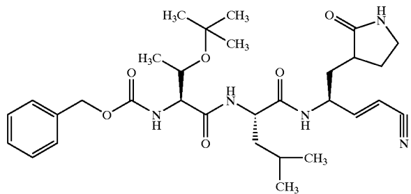
Compound 94
