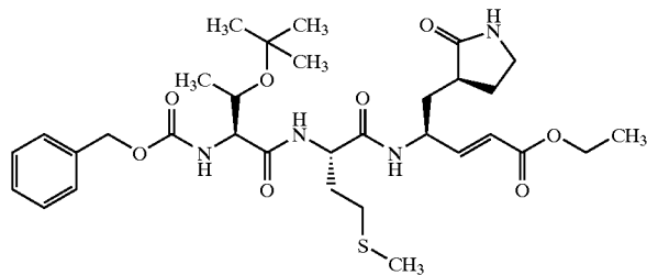
Compound 87
