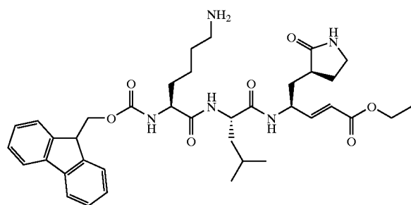
Compound 29
