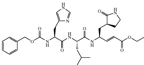
Compound 41
