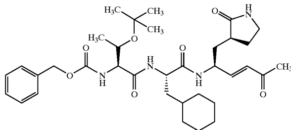
Compound 140
