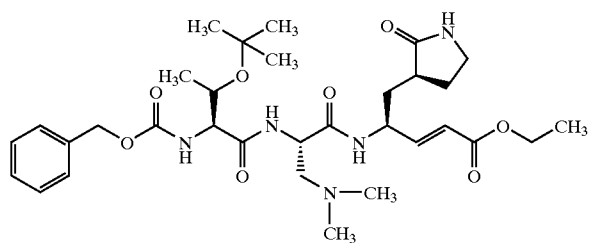
Compound 101
