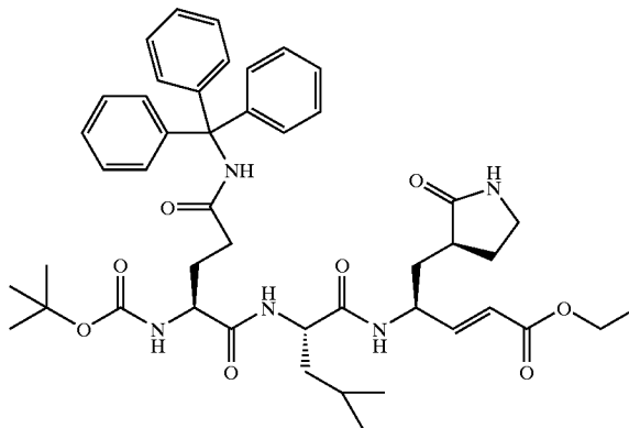
Compound 68
