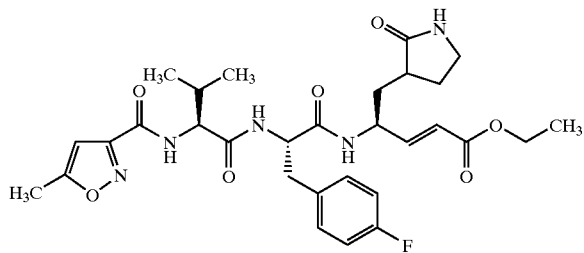
Compound 73
