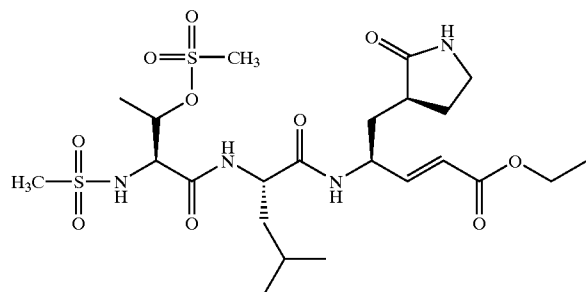
Compound 51
