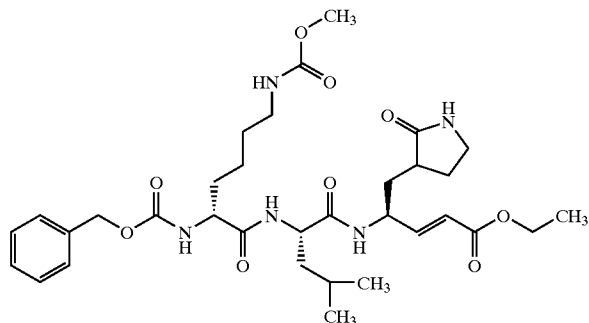
Compound 78
