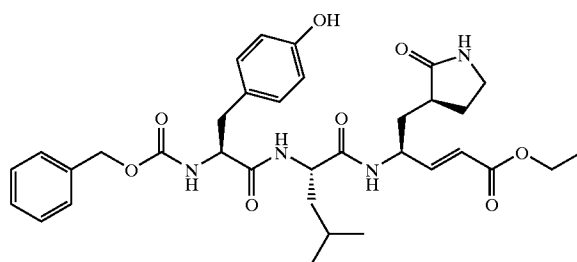
Compound 38
