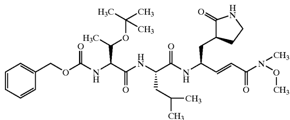
Compound 108
