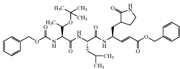
Compound 99
