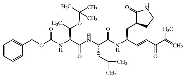
Compound 140
