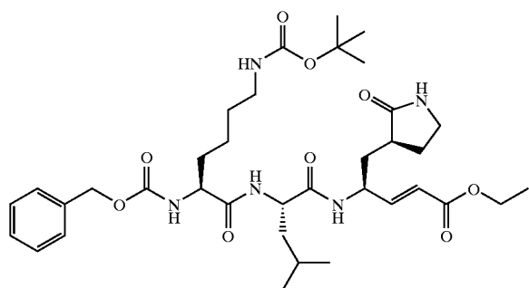
Compound 11
