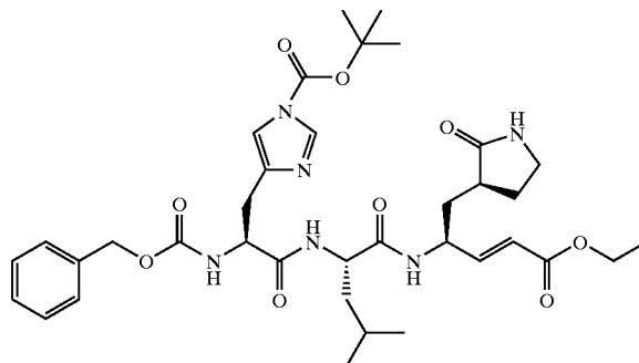
Compound 44
