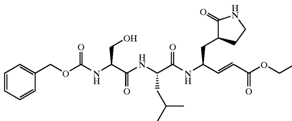
Compound 2
