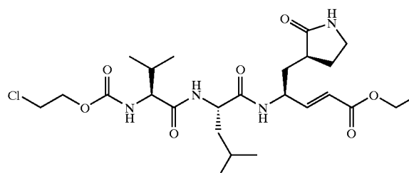
Compound 20
