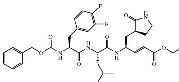
Compound 40
