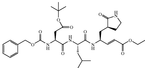
Compound 59
