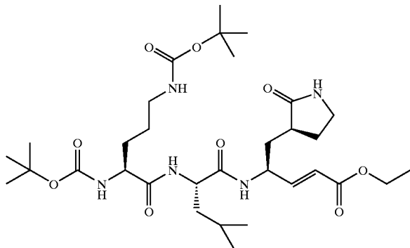
Compound 67
