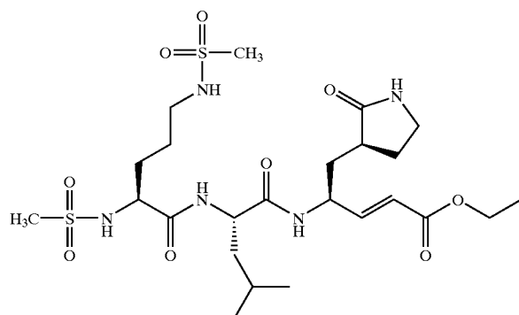
Compound 35
