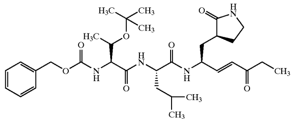
Compound 123
