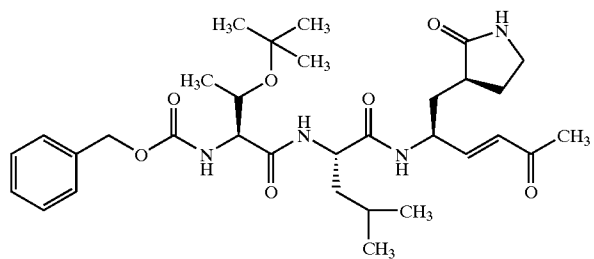
Compound 113
