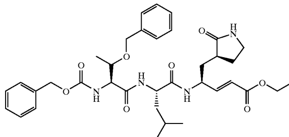
Compound 8
