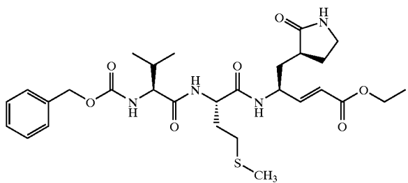
Compound 47
