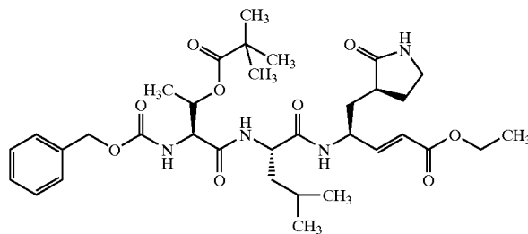
Compound 91
