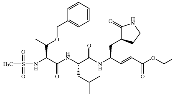
Compound 50
