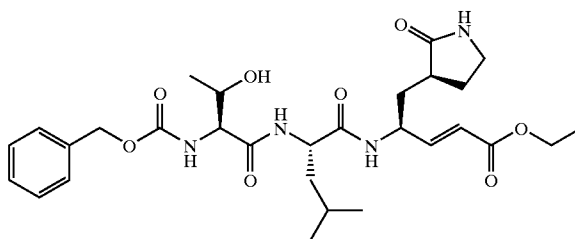
Compound 60
