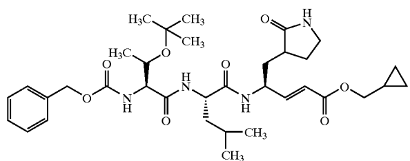
Compound 97
