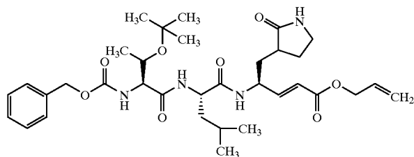
Compound 107
