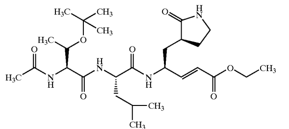
Compound 84
