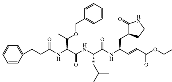
Compound 32
