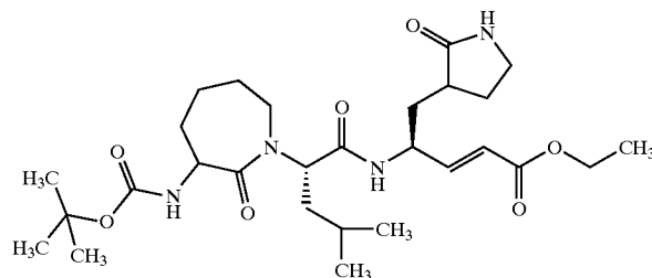
Compound 93
