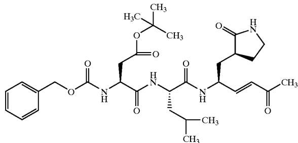
Compound 124
