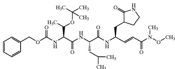
Compound 95
