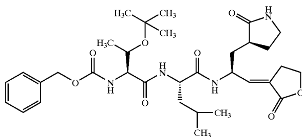
Compound 102
