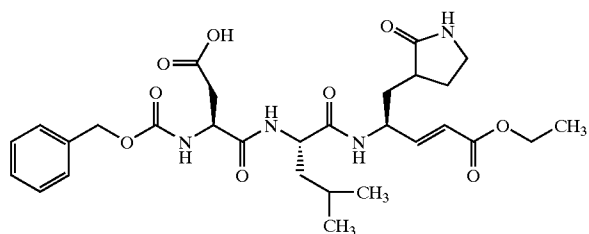
Compound 80
