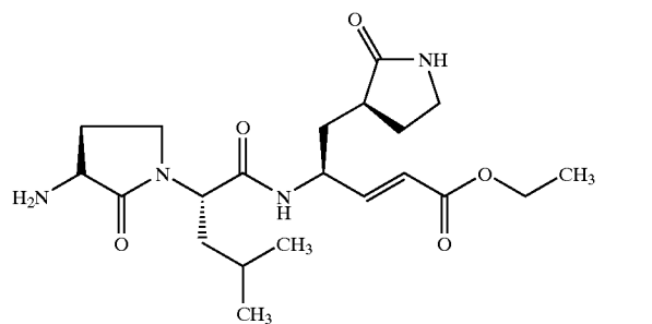
Compound 81
