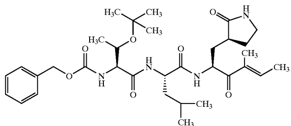
Compound 111
