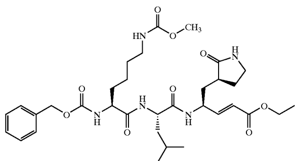
Compound 13
