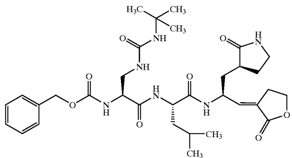
Compound 121
