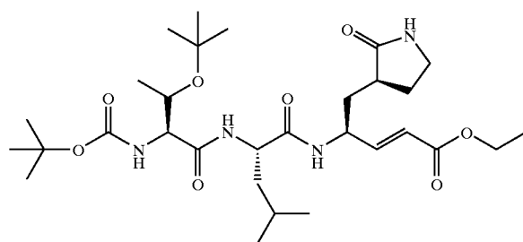
Compound 31
