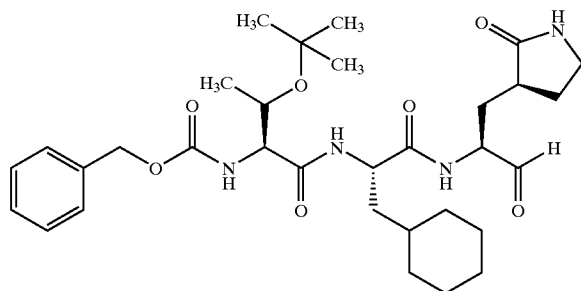
Compound 134
