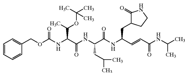
Compound 96
