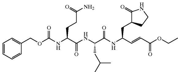
Compound 3
