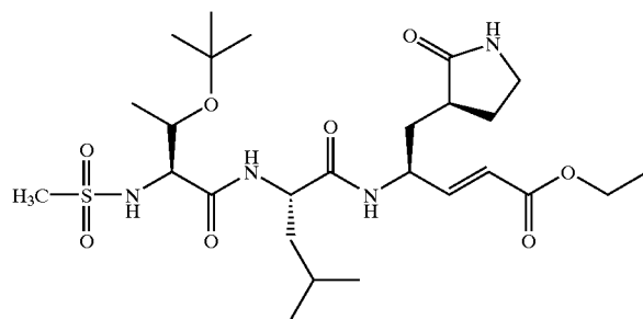
Compound 53
