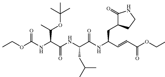
Compound 64
