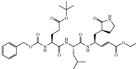
Compound 4
