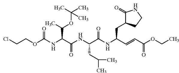
Compound 83
