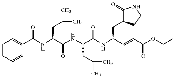
Compound 69
