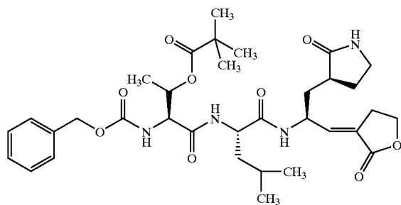
Compound 113
