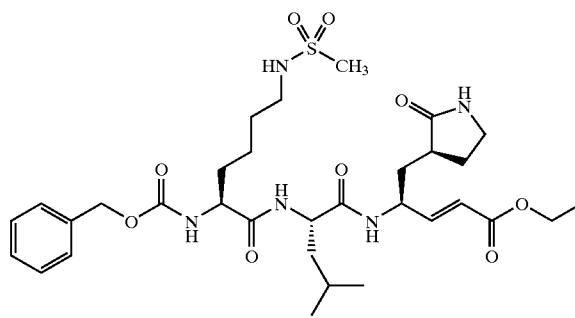
Compound 12
