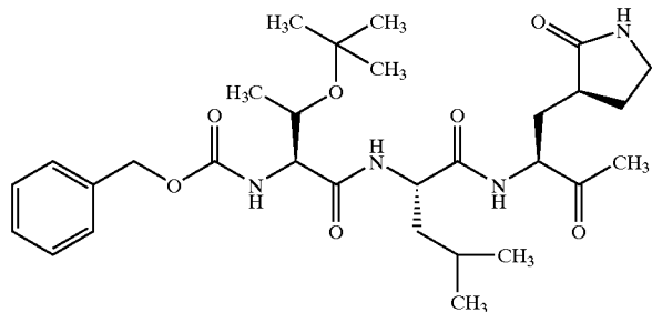
Compound 116
