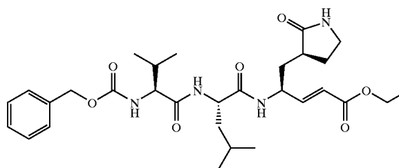
Compound 36
