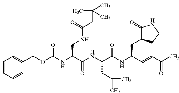
Compound 127
