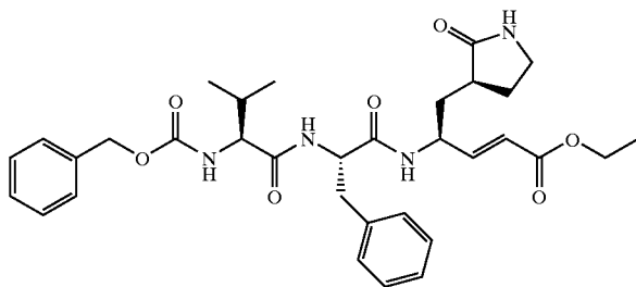
Compound 45
