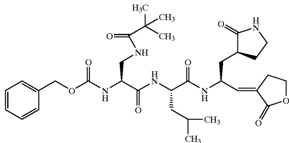
Compound 118
