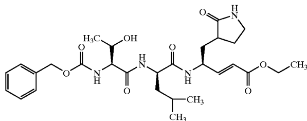
Compound 75
