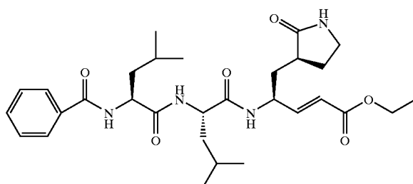
Compound 28
