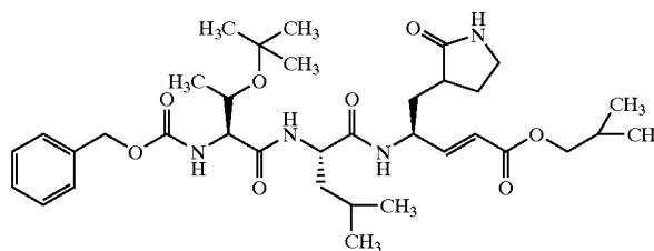
Compound 104
