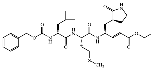
Compound 48
