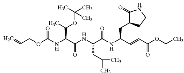
Compound 90
