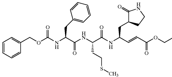
Compound 49
