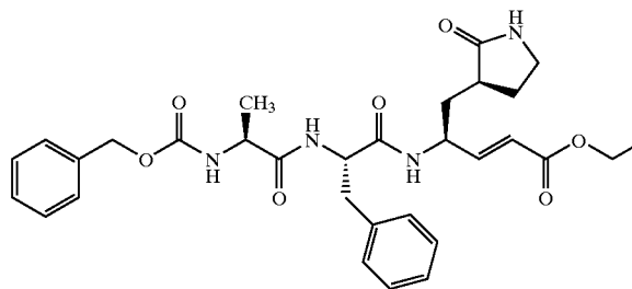
Compound 46
