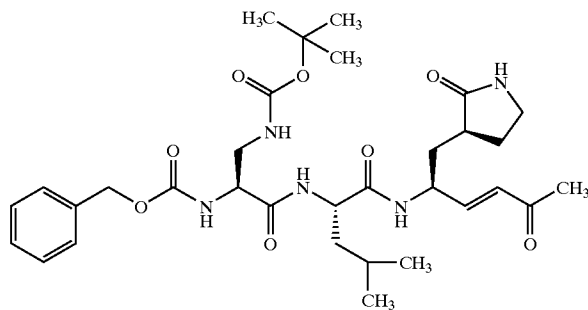
Compound 128
