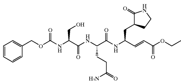
Compound 61
