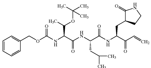
Compound 112
