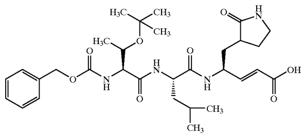
Compound 92
