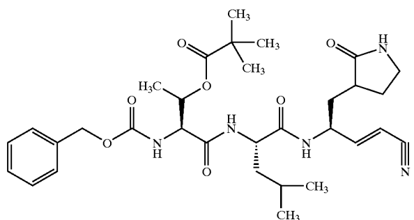
Compound 110
