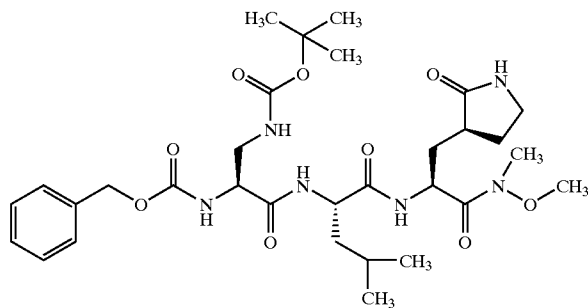
Compound 120
