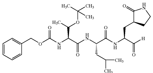
Compound 114
