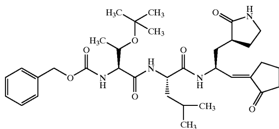
Compound 114
