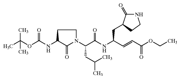
Compound 79
