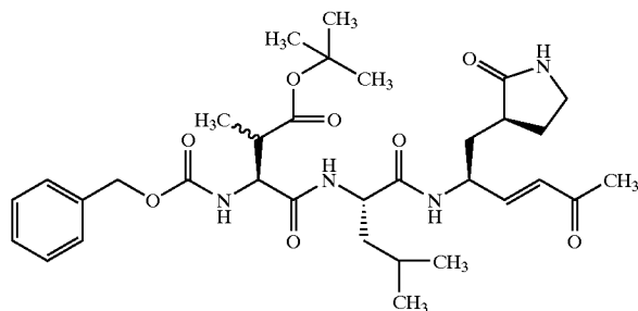
Compound 125
