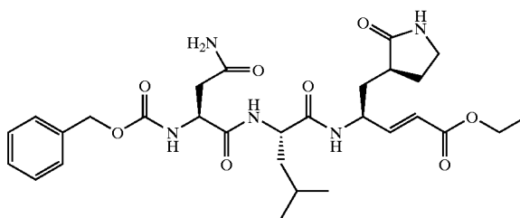
Compound 58
