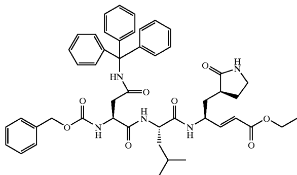
Compound 57
