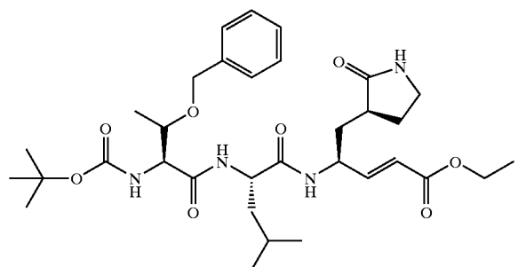
Compound 31
