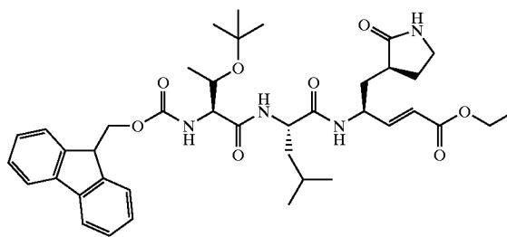
Compound 54
