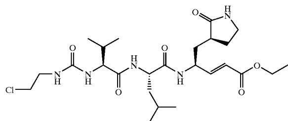
Compound 25
