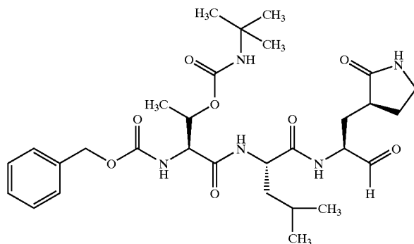
Compound 129
