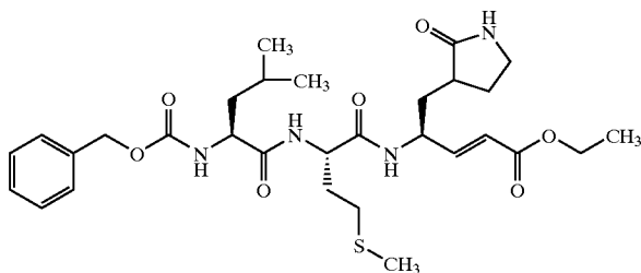
Compound 72
