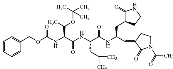
Compound 117
