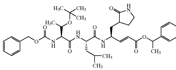
Compound 98
