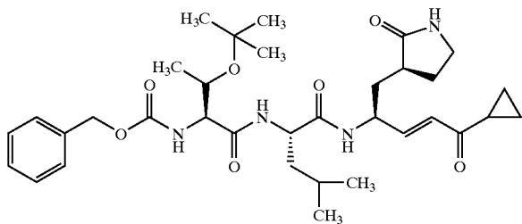
Compound 139
