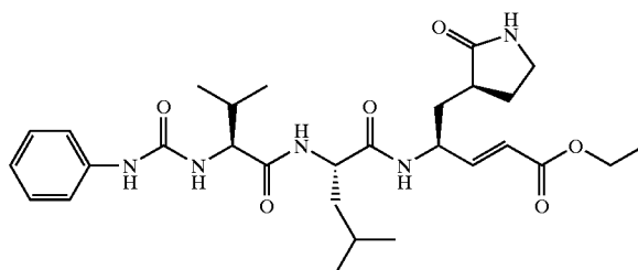
Compound 26
