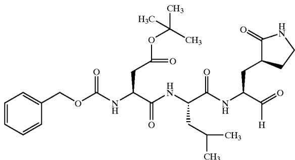
Compound 135
