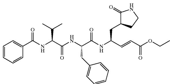
Compound 65
