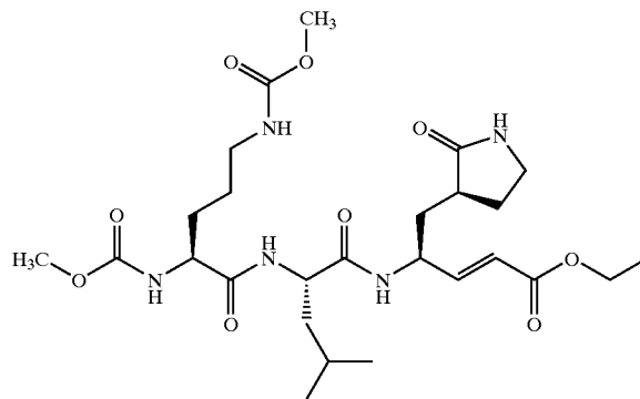
Compound 34
