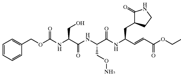
Compound 49
