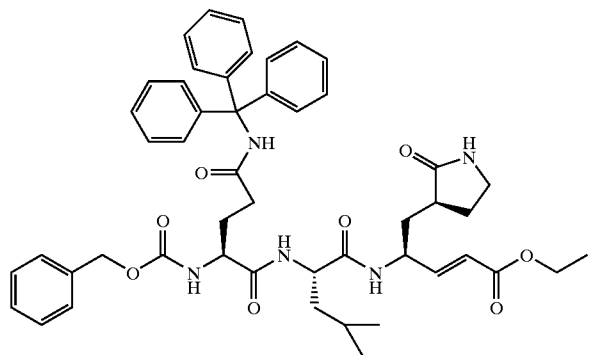
Compound 63
