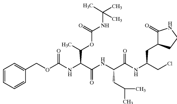
Compound 130
