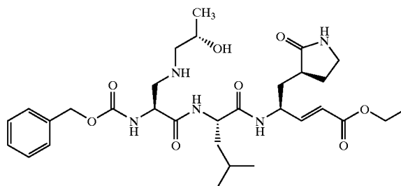
Compound 18
