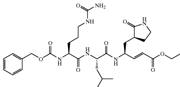
Compound 17
