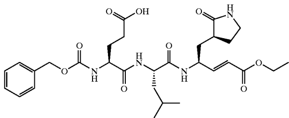
Compound 5
