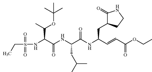
Compound 55
