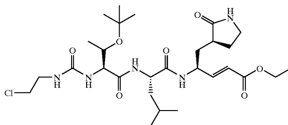
Compound 56
