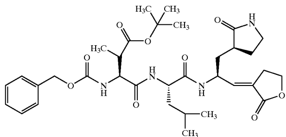
Compound 119
