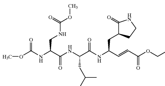
Compound 30
