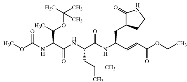
Compound 83
