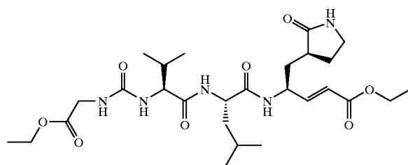
Compound 27
