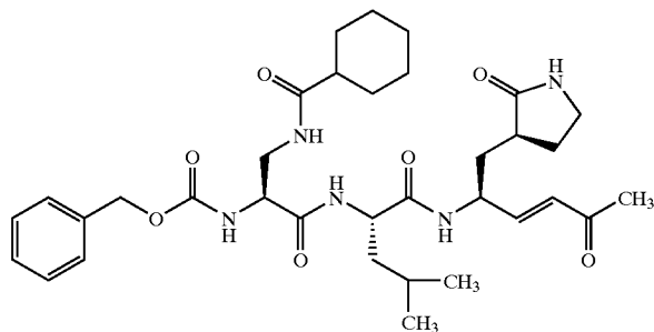
Compound 126
