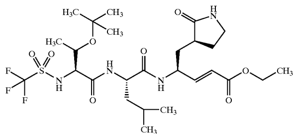
Compound 84
