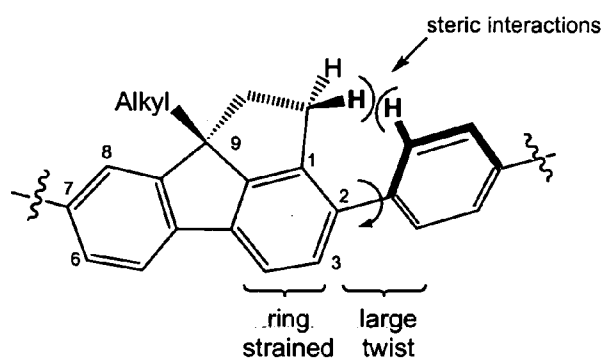
Figure 4. A Copolymer of Phenylene and Doubly-Bridged Biphenylene Showing the Decrease In Conjugation (Increases In Energy) of a Polymer Unit
