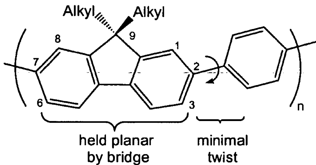
Figure 2. Polyfluorene Copolymer Showing the Polymer Conjugation
