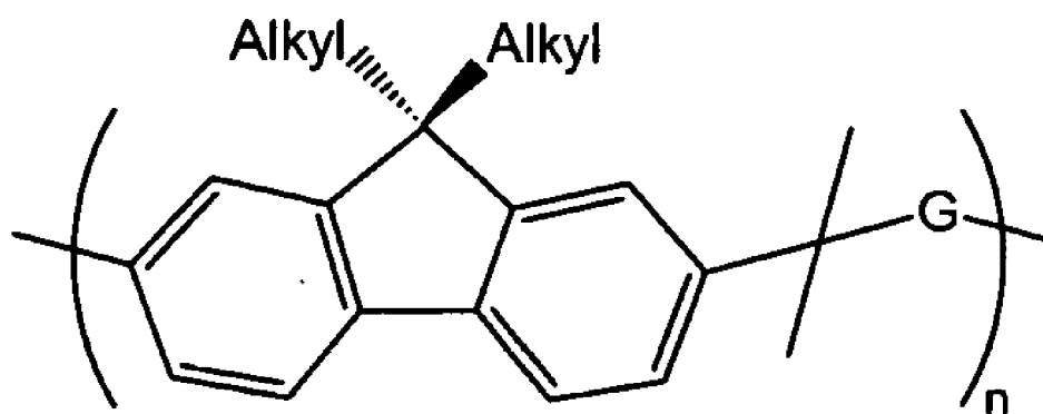
Figure 1. Generalized Structure of a Bridged-Polyphenylene Copolymer
