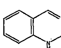
1,2-Dihydroquinazoline (1,2-dihydroquinazolinyl)
