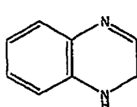
1,2-Dihydroquinoxaline (1,2-dihydroquinoxalinyl)
