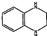
1,2,3,4-Tetrahydroquinoxaline (1,2,3,4-tetrahydroquinoxalinyl)
