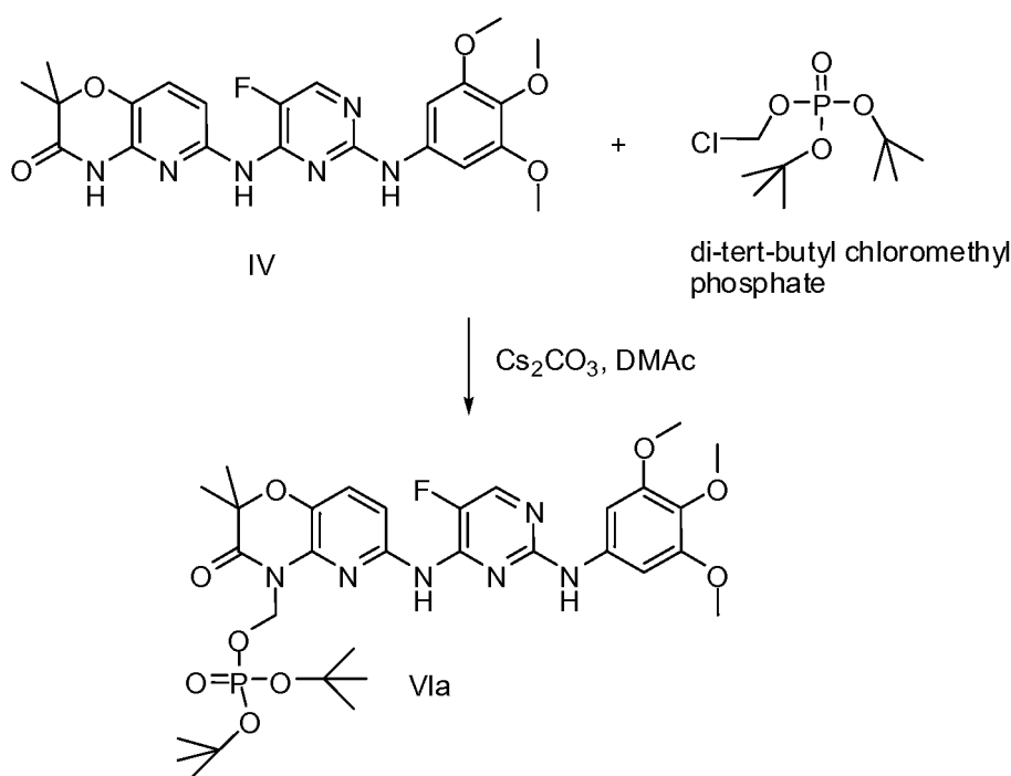
Scheme II
