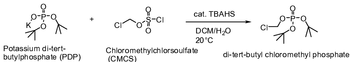
Scheme Ia
