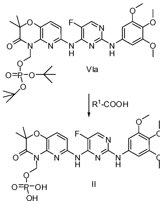
Scheme III
