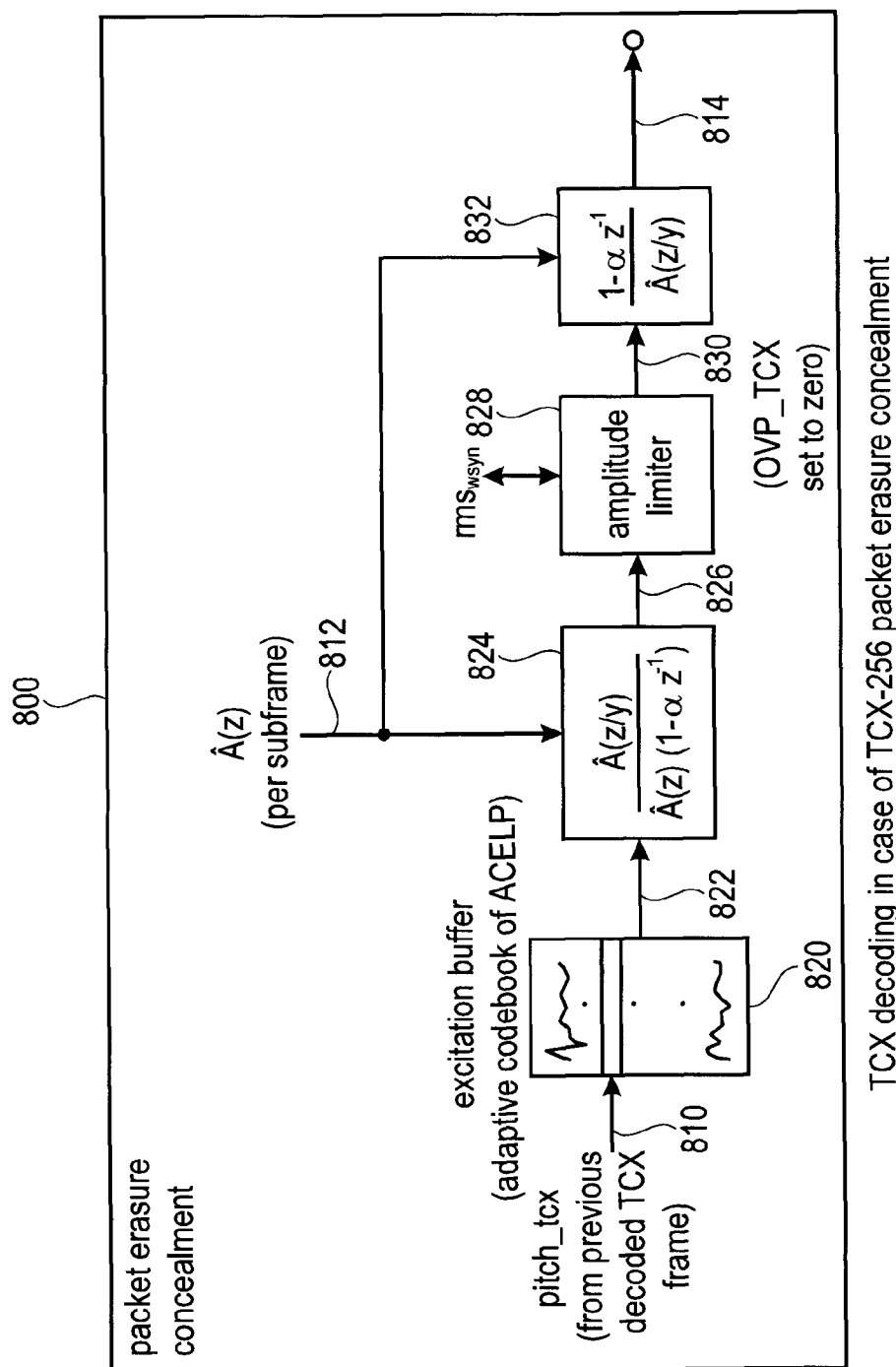
Block diagram of the TCX decoder
