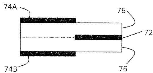
Middle Cross-Section FIG. 7B
