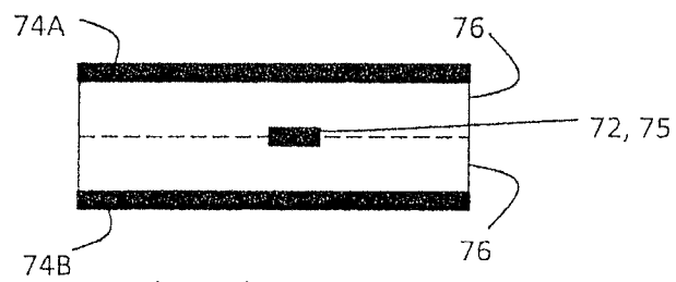
Right End Cross-Section FIG. 7C
