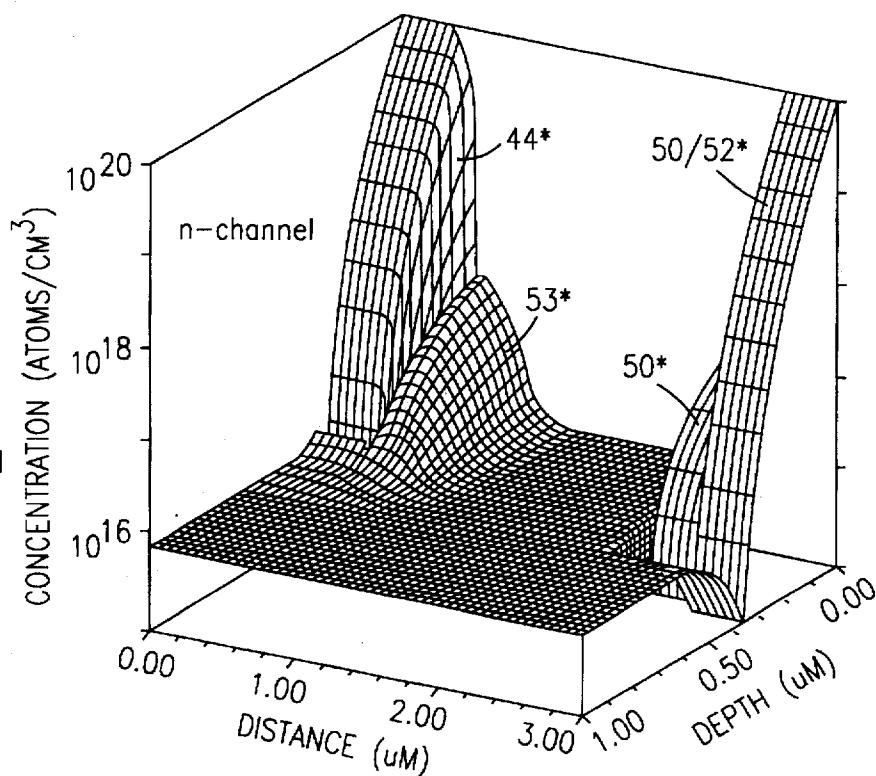
FIG. 14.1 Surface-peaked FET 40
