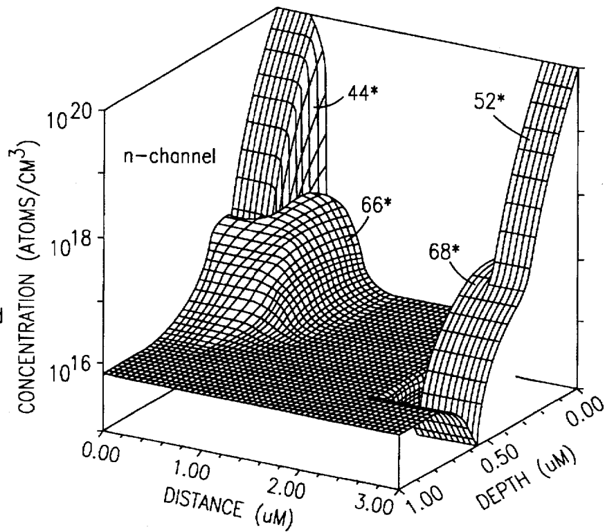
FIG. 20.1 Surface-peaked FET 60
