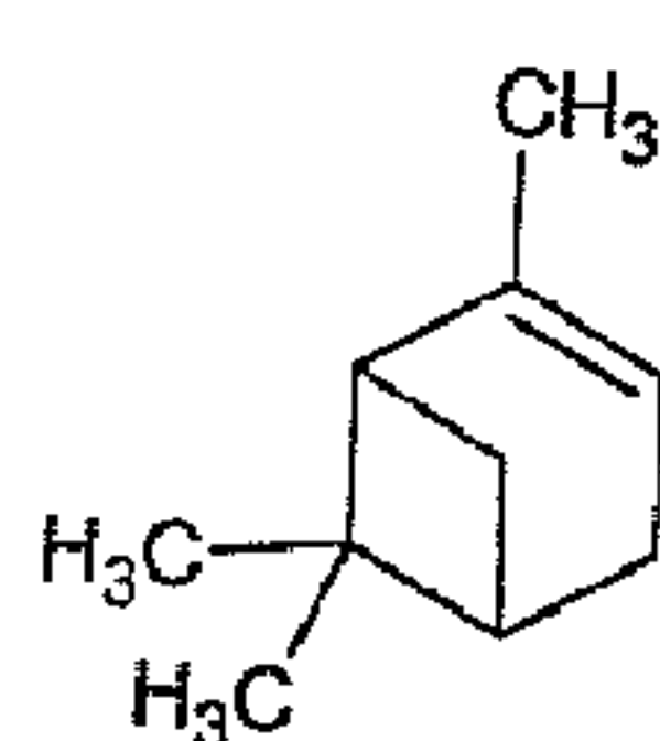
\alpha -pinene
