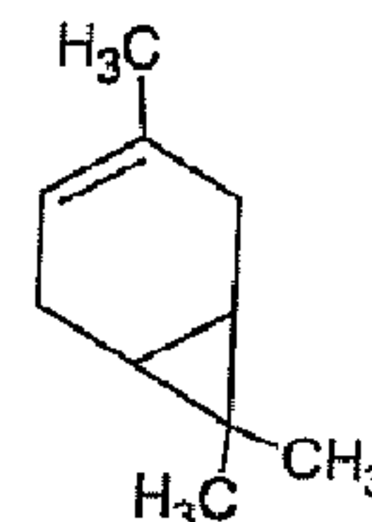
\Delta -3-carene
