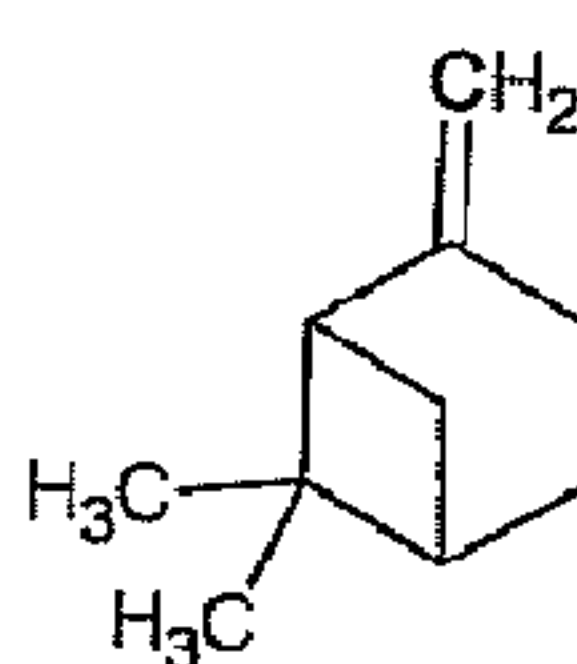
\beta -pinene
