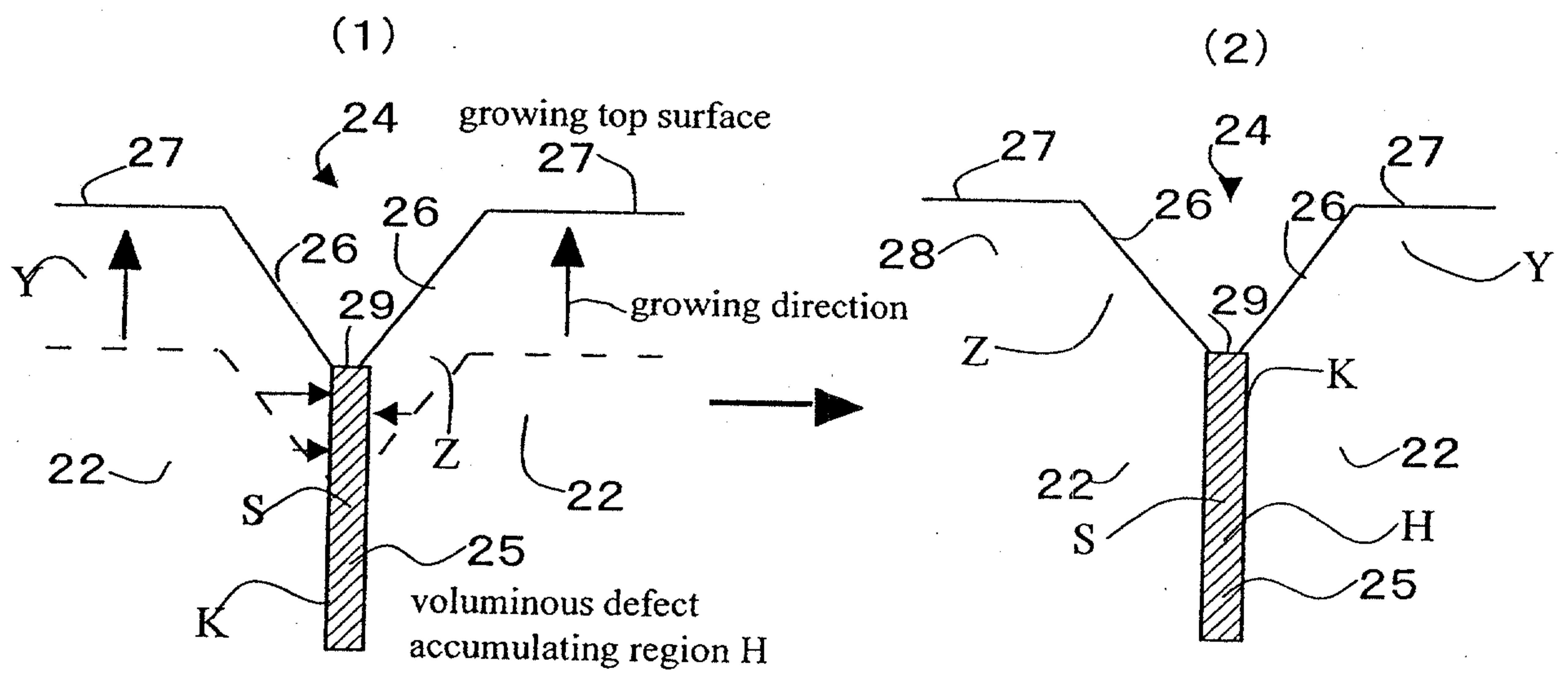
Fig.4 Growing method of the present invention
