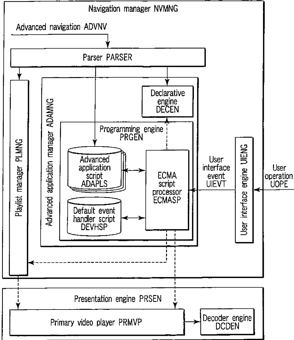
Explanatory view of user input handling model
