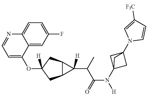
2-((1R,3S,5S,6R)-3-((6-fluoroquinolin-4-yl)oxy)bicyclo[3.1.0]hexan-6-yl)-N-(3-(3-(trifluoromethyl)-1H-pyrrol-1-yl)bicyclo[1.1.1]pentan-1-yl)propanamide
