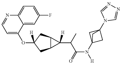
N-(3-(4H-1,2,4-triazol-4-yl)bicyclo[1.1.1]pentan-1-yl)-2-((1R,3S,5S,6R)-3-((6-fluoroquinolin-4-yl)oxy)bicyclo[3.1.0]hexan-6-yl)propanamide
