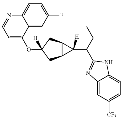
6-fluoro-4-(((1R,3s,5S,6r)-6-(1-(5-(trifluoromethyl)-1H-benzo[d]imidazol-2-yl)-propyl)bicyclo[3.1.0]hexan-3-yl)oxy)quinoline
