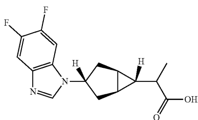
2-((1R,3R5S,6r)-3-(5,6-difluoro-1H-benzo[d]imidazol-1-yl)bicyclo[3.1.0]hexan-6-yl)propanoic acid
