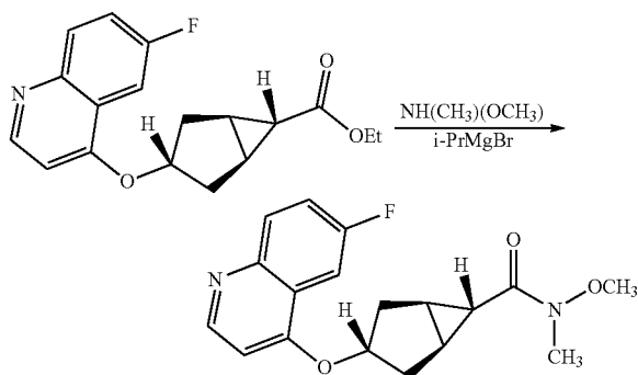
(1R,3s,5S,6r)-3-((6-Fluoroquinolin-4-yl)oxy)-N-methoxy-N-methylbicyclo[3.1.0]hexane-6-carboxamide
