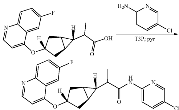
N-(5-Chloropyridin-2-yl)-2-((1R,3s,5S,6r)-3-((6-fluoroquinolin-4-yl)oxy)-bicyclo[3.1.0]hexan-6-yl)propanamide
