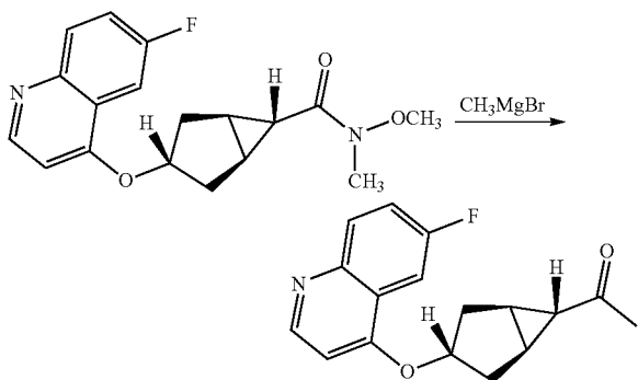
1-((1R,3s,5S,6r)-3-((6-fluoroquinolin-4-yl)oxy)bicyclo[3.1.0]hexan-6-yl)ethan-1-one
