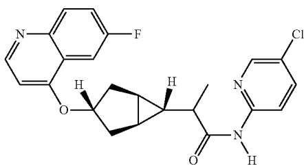
N-(5-chloropyridin-2-yl)-2-((1R,3s,5S,6r)-3-((6-fluoroquinolin-4-yl)oxy)-bicyclo[3.1.0]hexan-6-yl)propanamide
