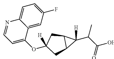
2-((1R,3s,5S,6r)-3-((6-fluoroquinolin-4-yl)oxy)bicyclo[3.1.0]hexan-6-yl)propanoic acid
