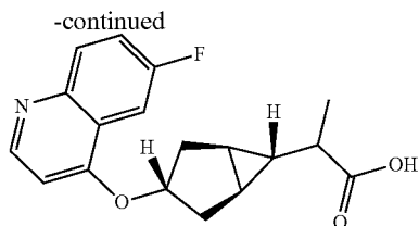
2-((1R,3S,5S,6r)-3-((6-Fluoroquinolin-4-yl)oxy)bicyclo[3.1.0]hexan-6-yl)propanoic acid
