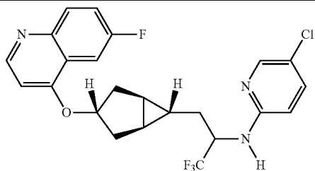
5-Chloro-N-((1,1,1-trifluoro-3-((1R,3R,5S,6S)-3-((6-fluoroquinolin-4-yl)oxy)bicyclo[3.1.0]hexan-6-yl)propan-2-yl)pyridin-2-amine
