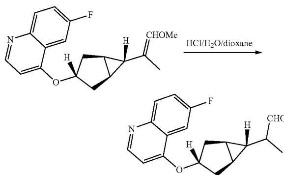
2-((1R,3s,5S,6r)-3-((6-fluoroquinolin-4-yl)oxy)bicyclo[3.1.0]hexan-6-yl)propanal
