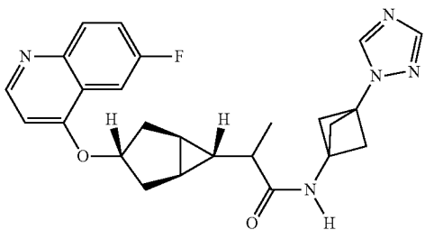
N-(3-(1H-1,2,4-triazol-1-yl)bicyclo[1.1.1]pentan-1-yl)-2-((1R,3S,5S,6R)-3-((6-fluoroquinolin-4-yl)oxy)bicyclo[3.1.0]hexan-6-yl)propanamide
