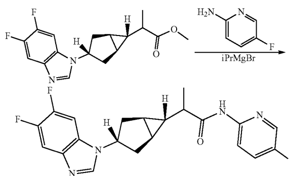
2-((1R,3s,5S,6r)-3-(5,6-difluoro-1H-benzo[d]imidazol-1-yl)bicyclo[3.1.0]hexan-6-yl)-N-(5-fluoropyridin-2-yl)propanamide
