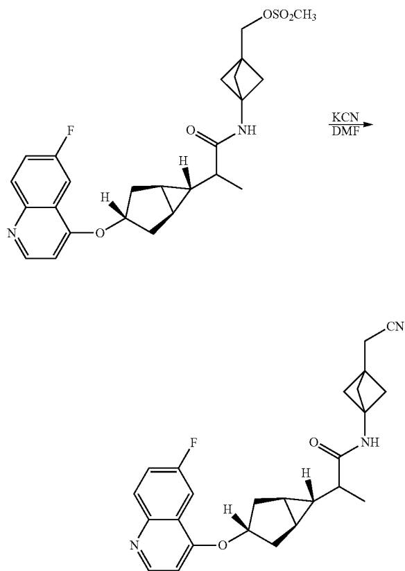
N-(3-(cyanomethyl)bicyclo[1.1.1]pentan-1-yl)-2-((1R,3s,5S,6r)-3-((6-fluoroquinolin-4-yl)oxy)bicyclo[3.1.0]hexan-6-yl)propanamide
