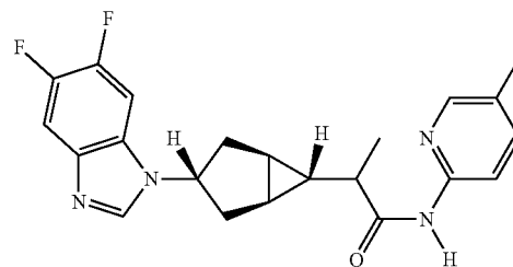
2-((1R,3s,5S,6r)-3-(5,6-difluoro-1H-benzo[d]imidazol-1-yl)bicyclo[3.1.0]hexan-6-yl)-N-(5-fluoropyridin-2-yl)propanamide
