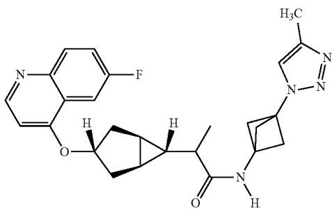
2-((1R,3S,5S,6R)-3-((6-fluoroquinolin-4-yl)oxy)bicyclo[3.1.0]hexan-6-yl)-N-(3-(4-methyl-1H-1,2,3-triazol-1-yl)bicyclo[1.1.1]pentan-1-yl)propanamide
