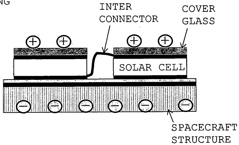
FIG. 1 DISCHARGE MECHANISM
