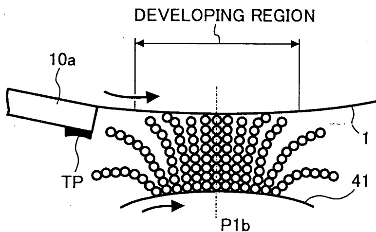
FIG. 6 BACKGROUND ART
