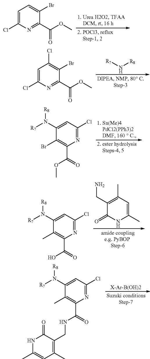
Scheme 5
