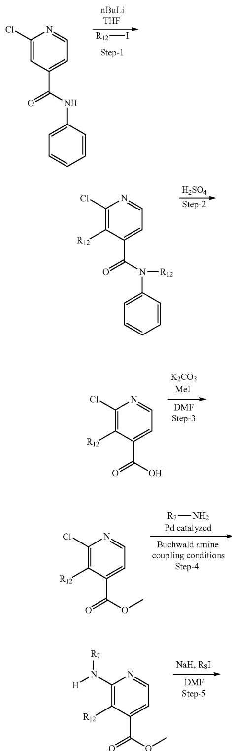
Scheme 8
