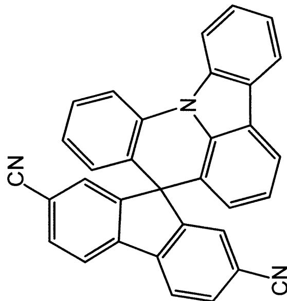
Chemical Formula 2-3
