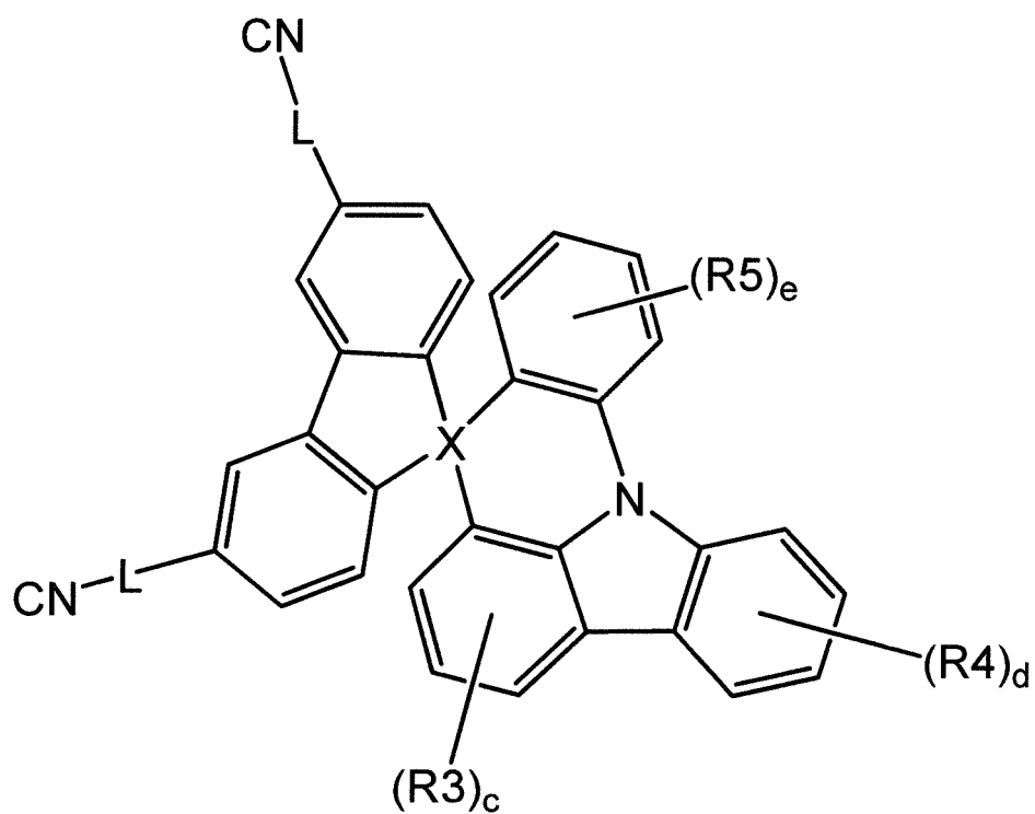
[Chemical Formula 1-5]
