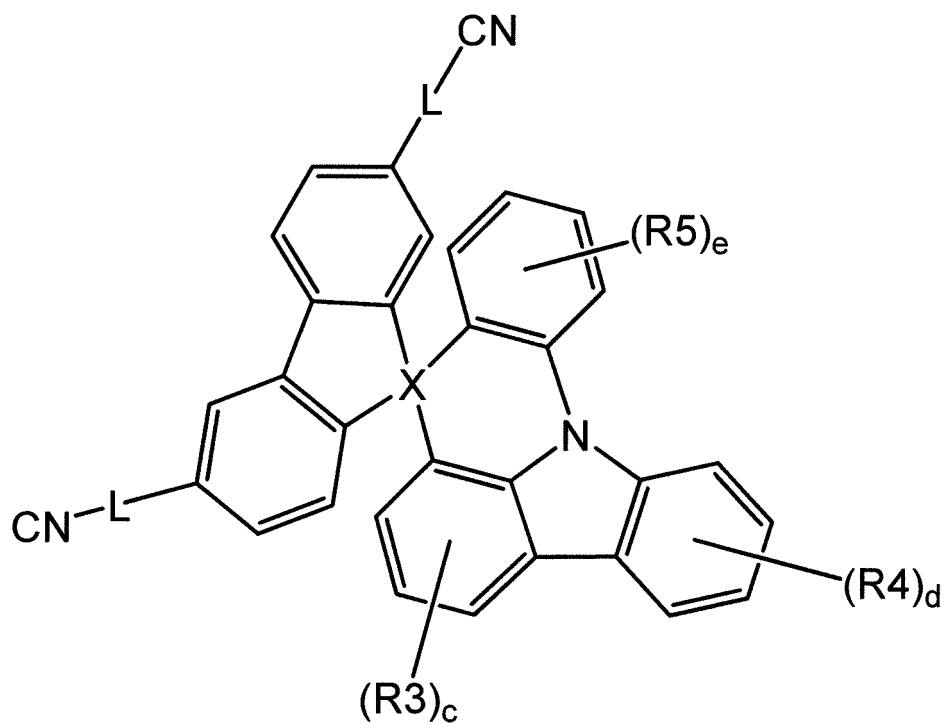
[Chemical Formula 1-5]
