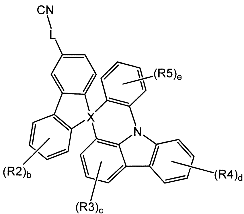
[Chemical Formula 1-3]
