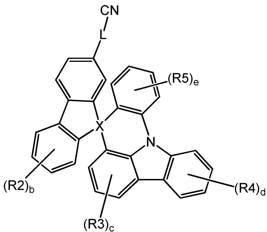
[Chemical Formula 1-2]
