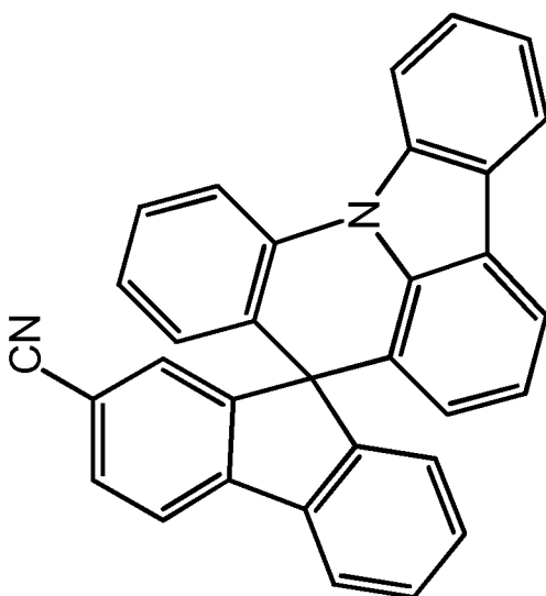
Chemical Formula 2-1
