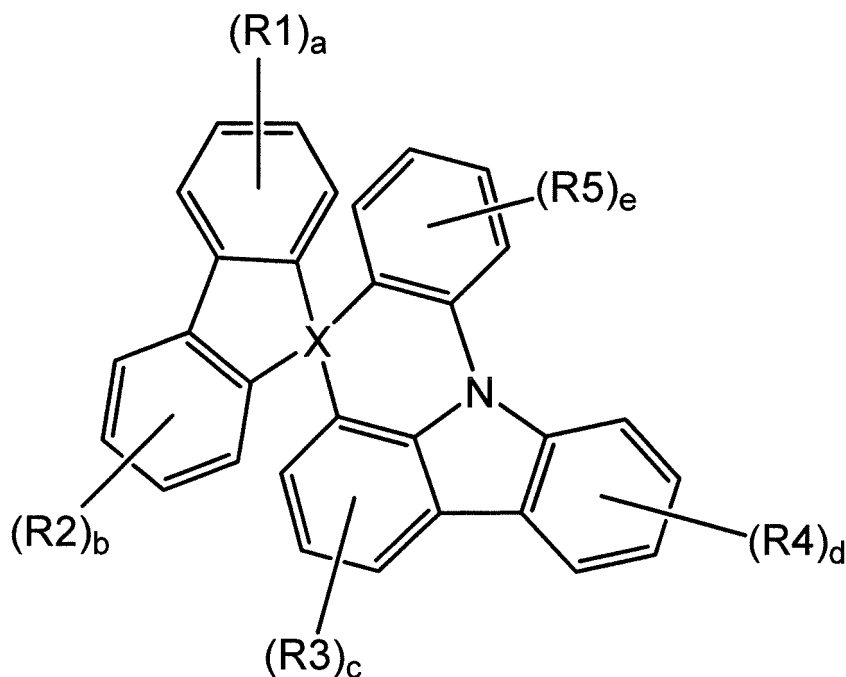
[Chemical Formula 1]
