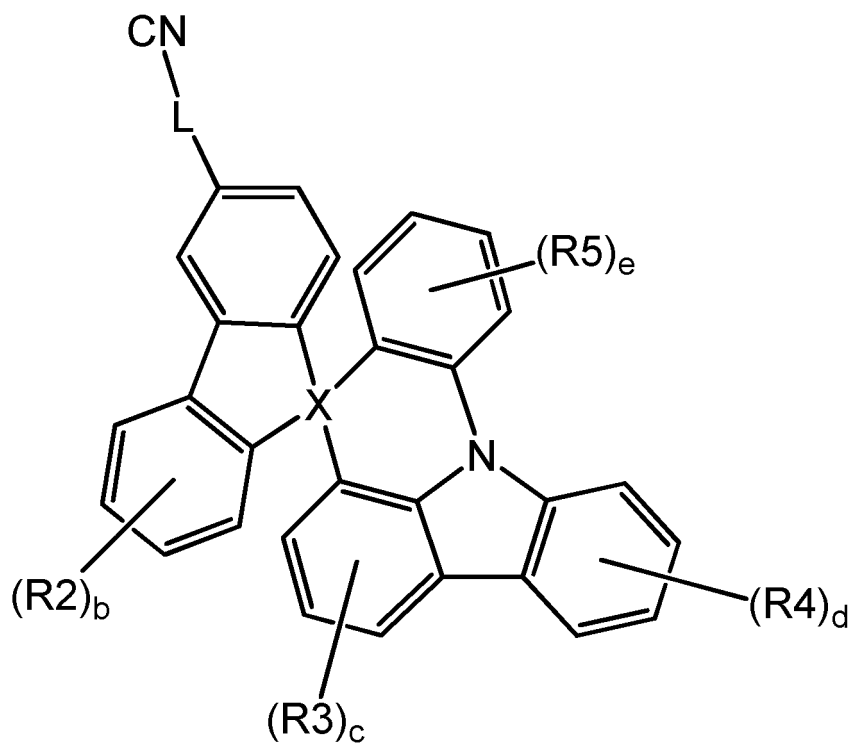
[Chemical Formula 1-3]
