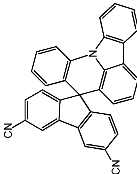
Chemical Formula 2-4
