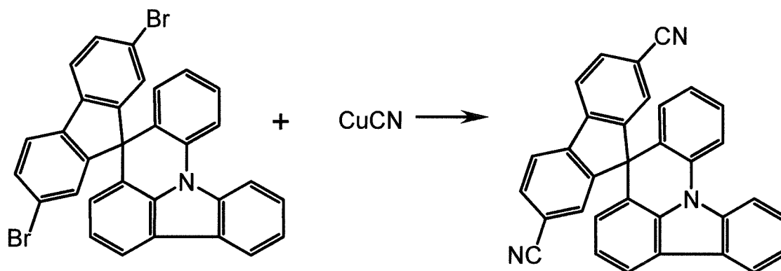
[Compound A]
