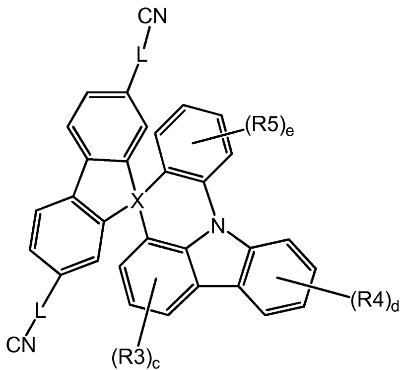
[Chemical Formula 1-4]
