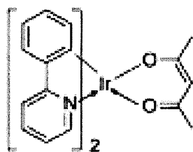
[(PPy) 2 Ir(acac)]
