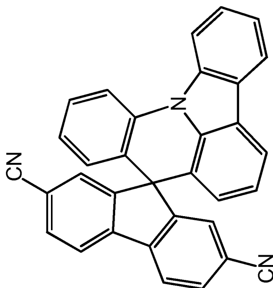
Chemical Formula 2-3
