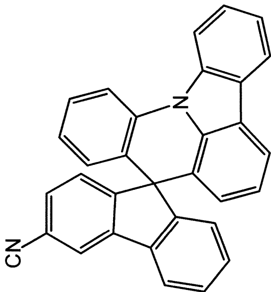
Chemical Formula 2-2
