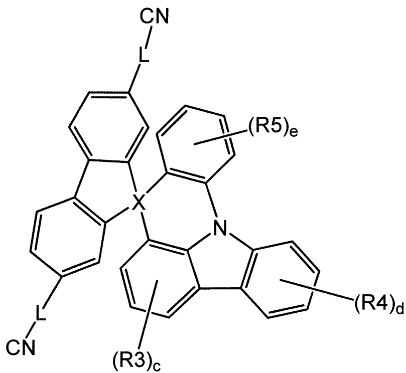
[Chemical Formula 1-3]
