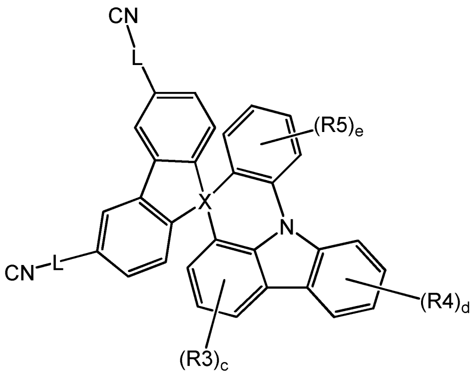
[Chemical Formula 1-5]
