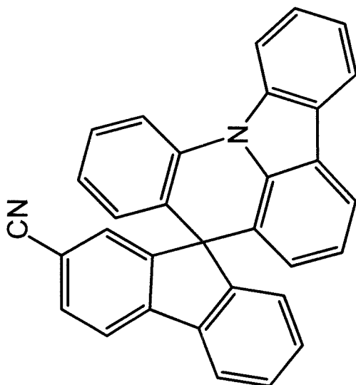
Chemical Formula 2-1
