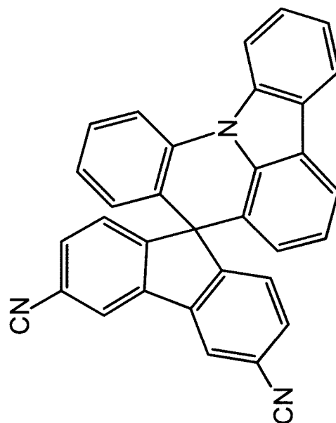
Chemical Formula 2-4
