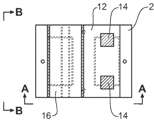
Figure 3 Plan View
