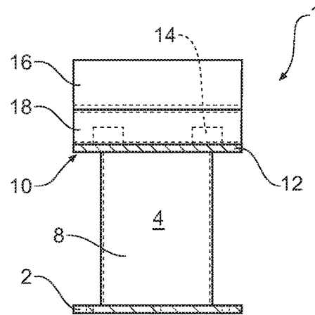
Figure 2 Section B-B
