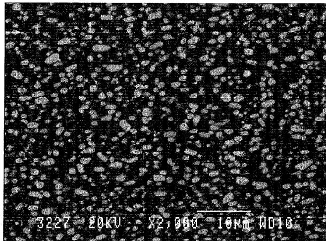
Microstructure of the inventive alloy. The white phase is \text{Mo}_2\text{FeB}_2 . The length of the bar is 10 \mu\text{m} .
