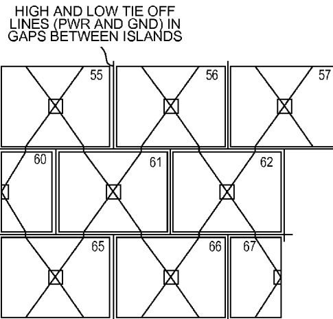
CONFIGURABLE MESH CONTROL BUS FIG. 27
