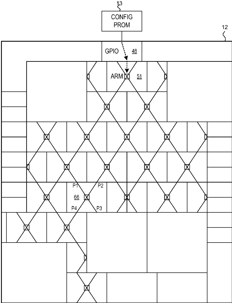
CONFIGURABLE MESH CONTROL BUS STRUCTURE
