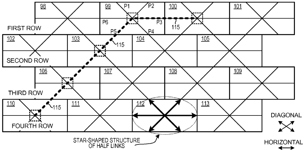
STAGGERED-PATTERN ISLANDS WITH STAR-SHAPED HALF-LINK STRUCTURE
