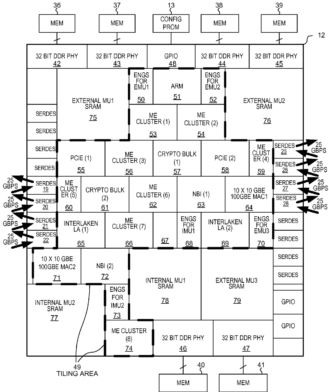
IBNFP INTEGRATED CIRCUIT
