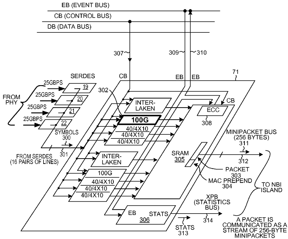
MAC ISLAND (INGRESS)
