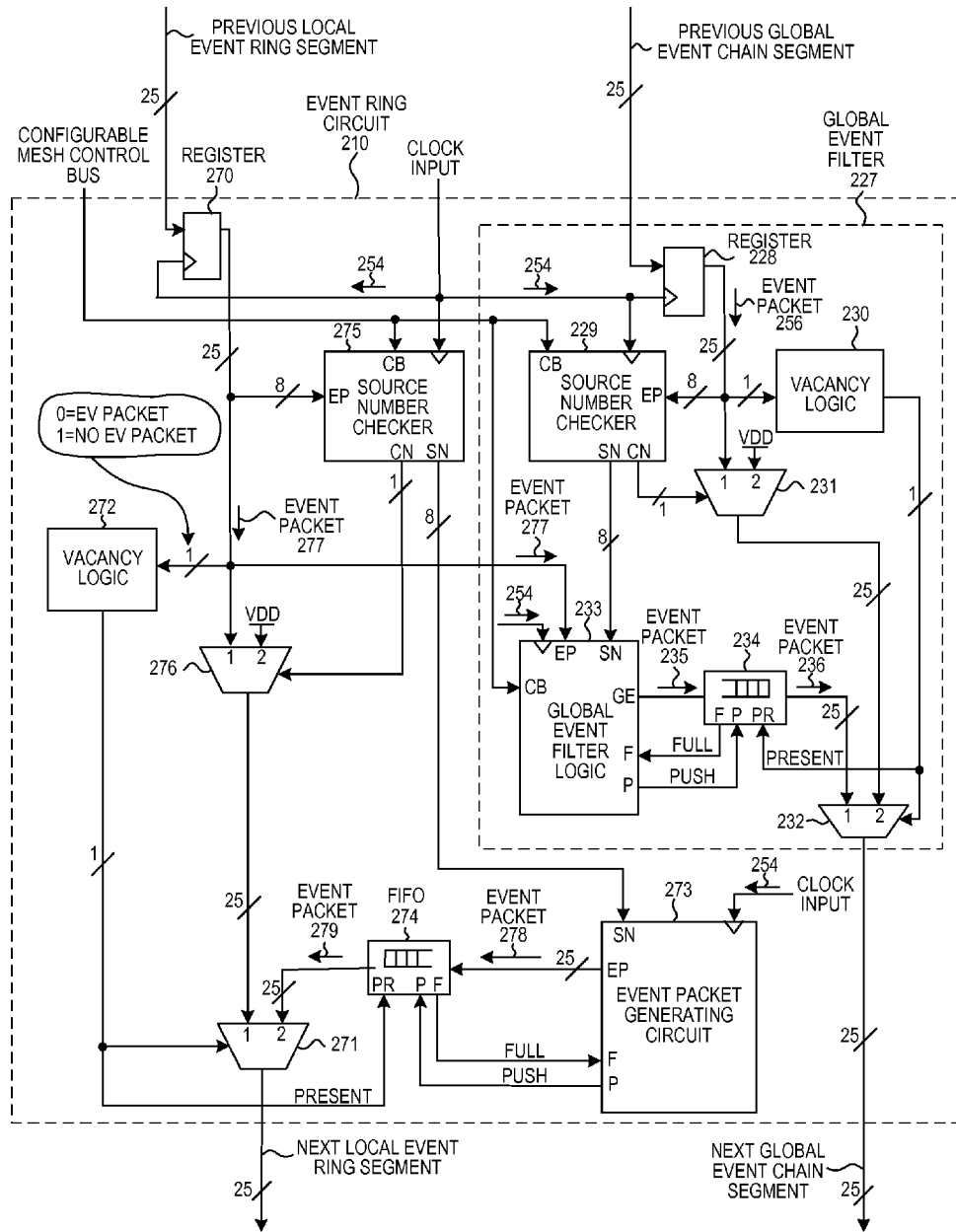
EVENT RING CIRCUIT WITH GLOBAL EVENT FILTER
