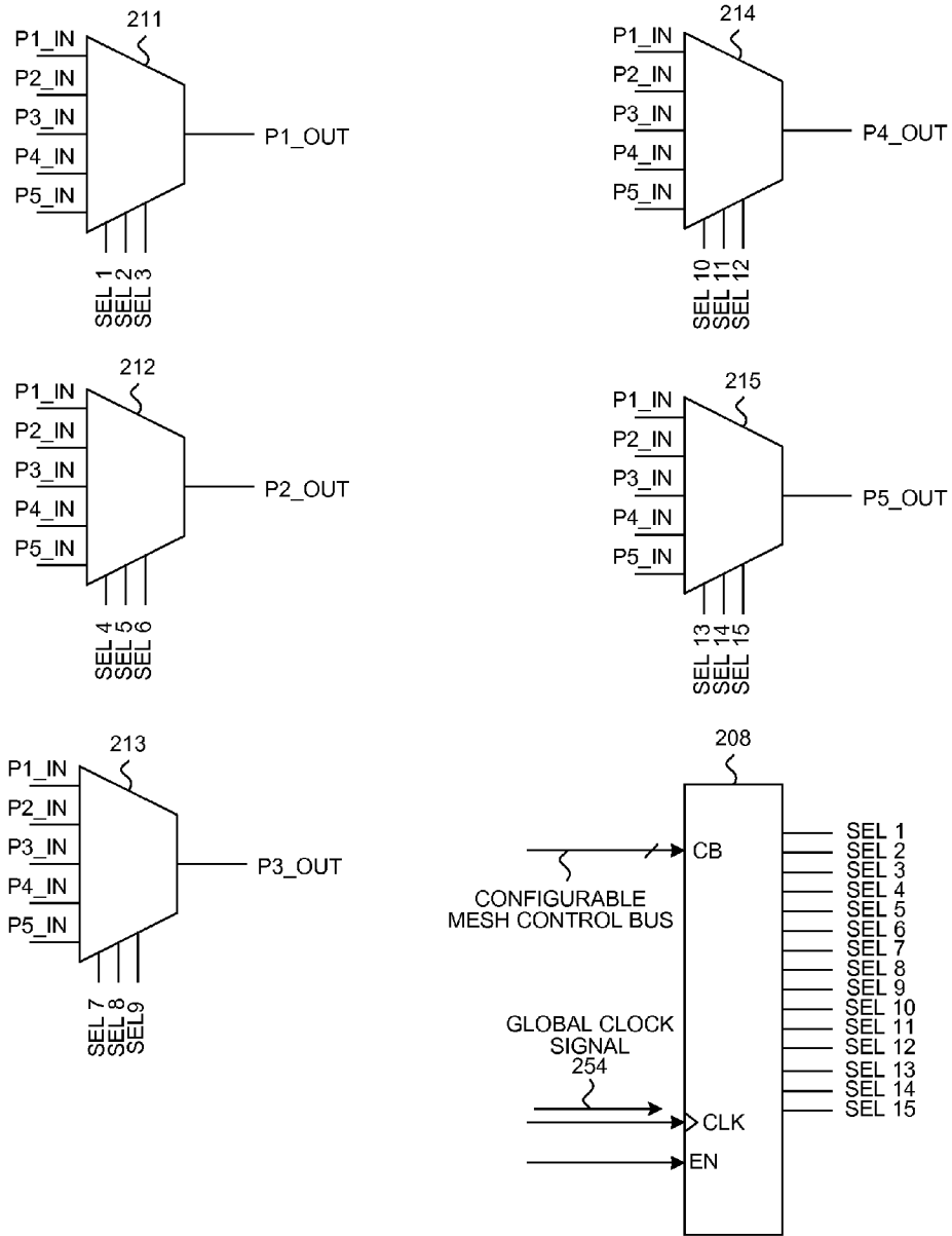
RUN TIME CONFIGURABLE SWITCH CIRCUIT
