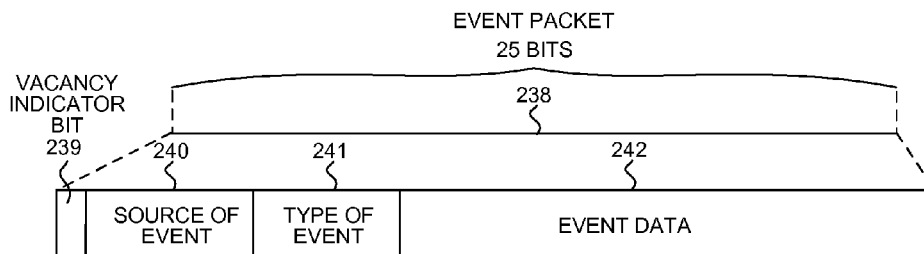
EVENT PACKET BIT SEQUENCE FIG. 38A
