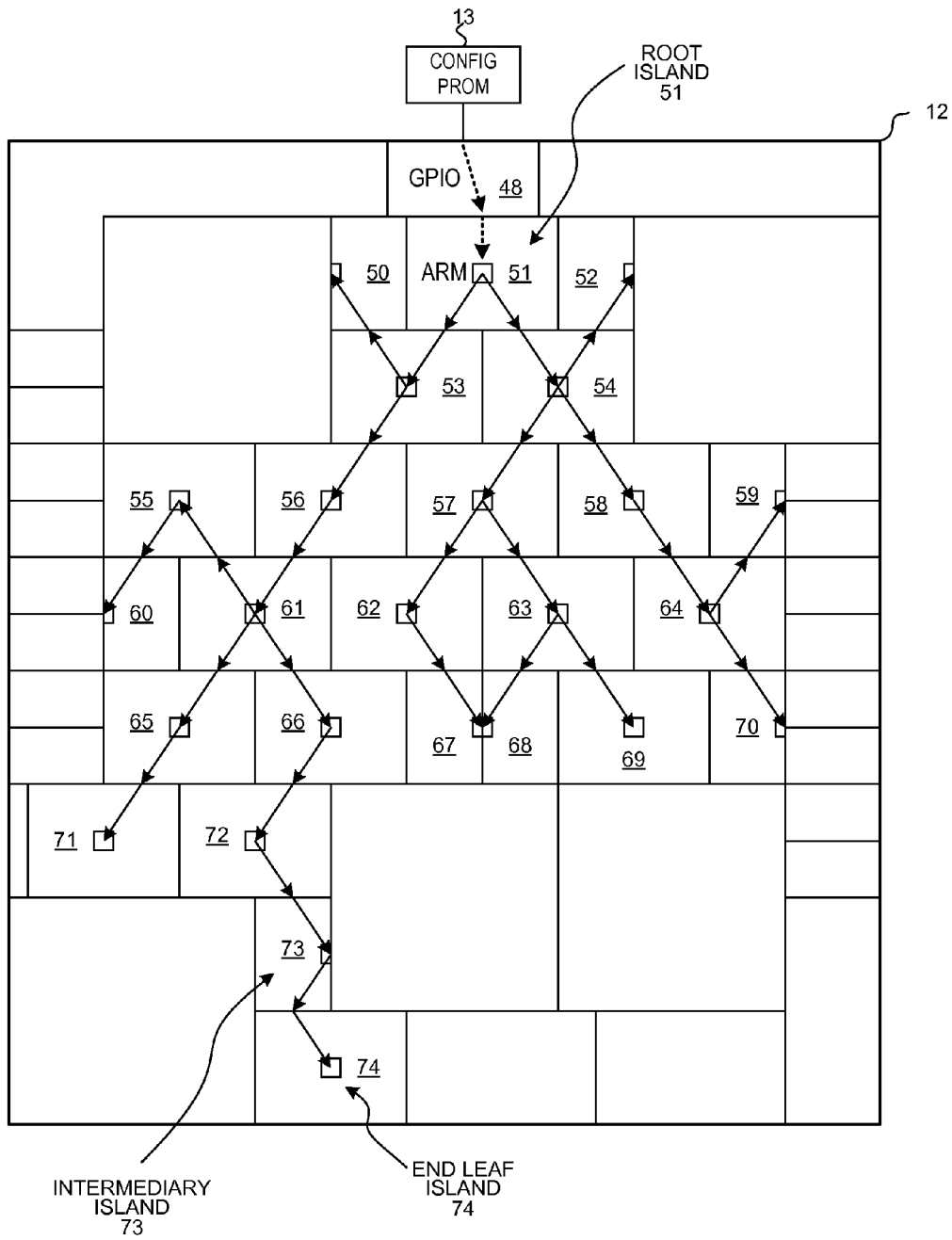
CONFIGURED CONFIGURABLE MESH CONTROL BUS
