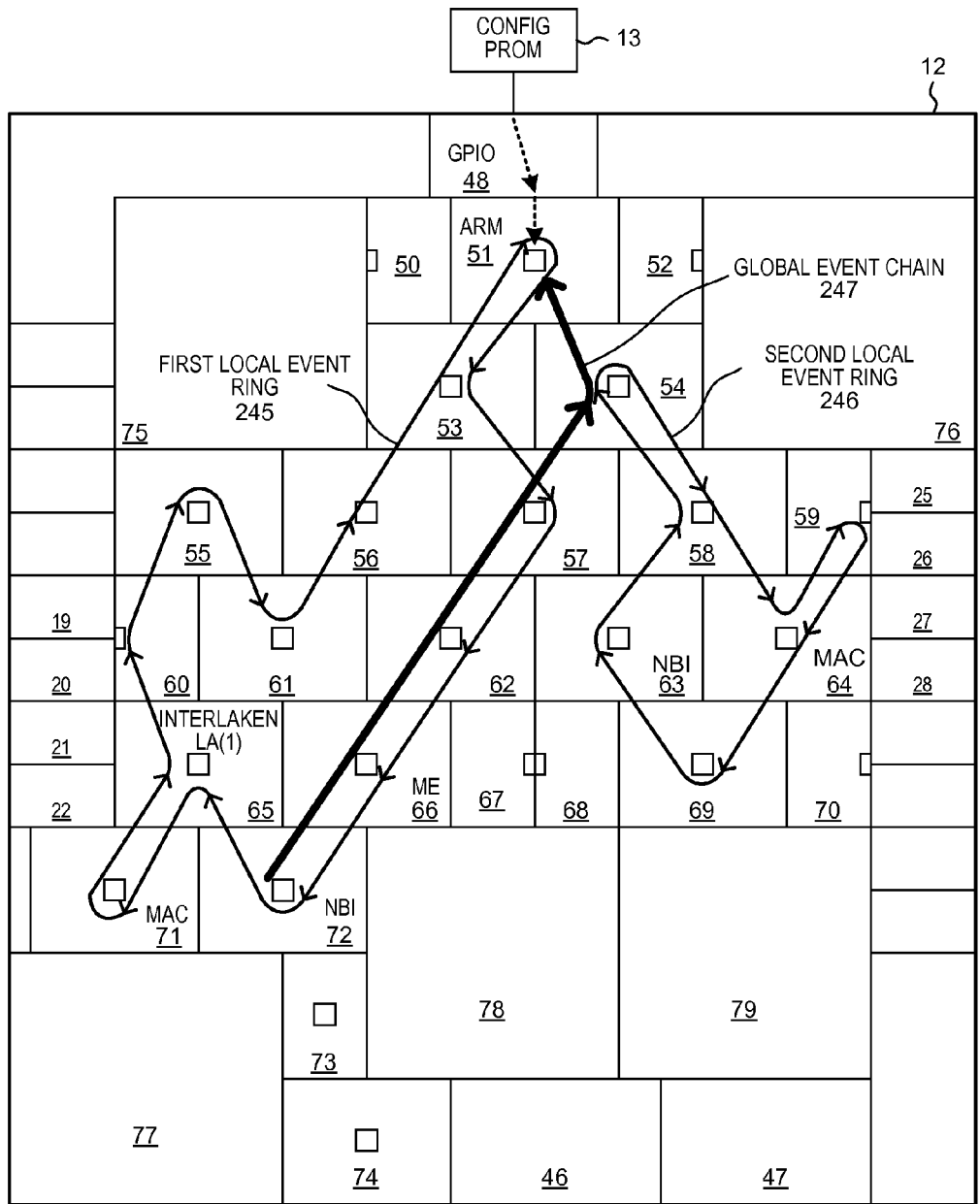
CONFIGURED CONFIGURABLE MESH EVENT BUS
