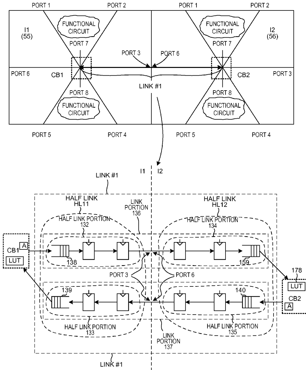
LINK BETWEEN TWO CROSSBAR SWITCHES
