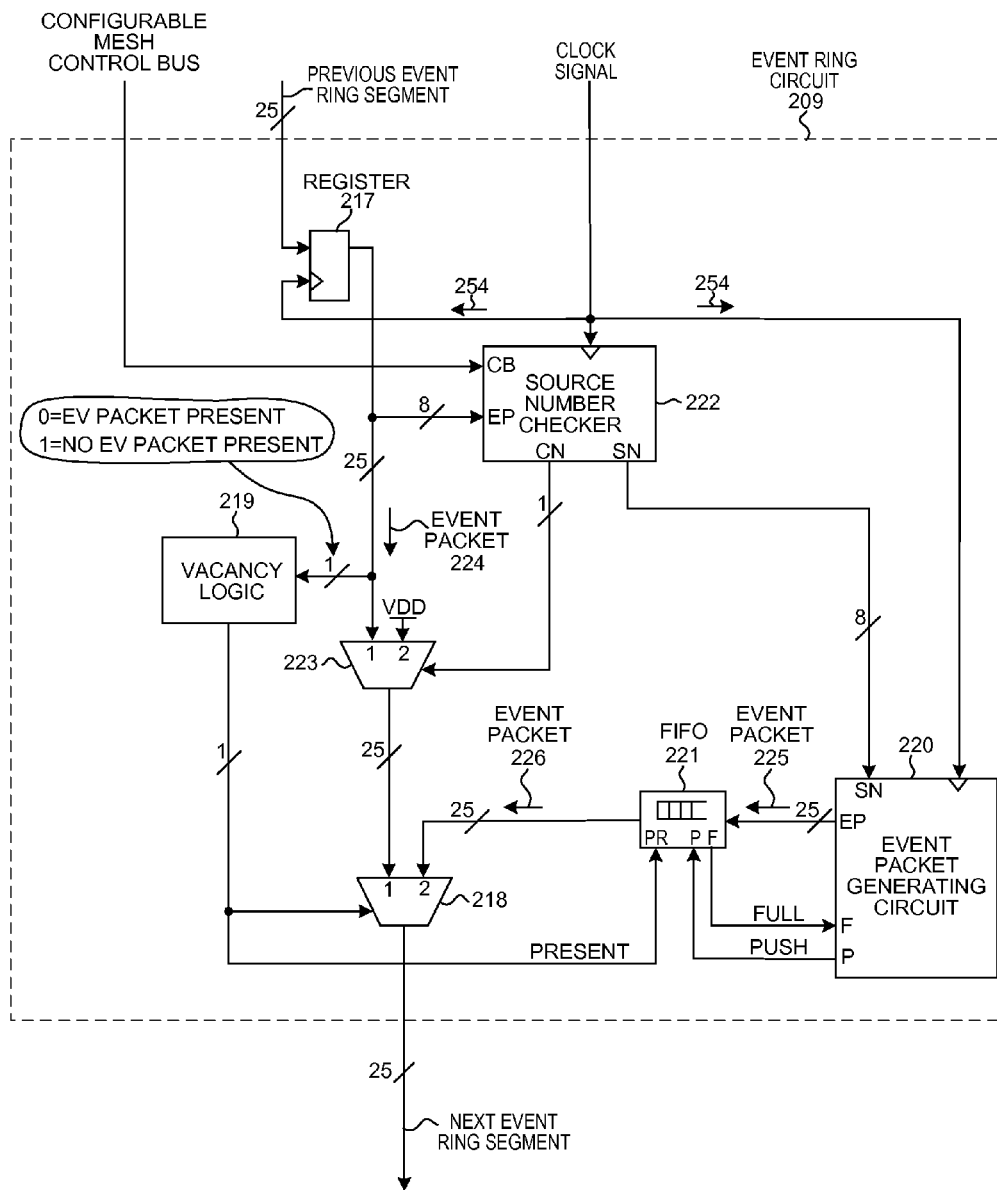
EVENT RING CIRCUIT FIG. 36
