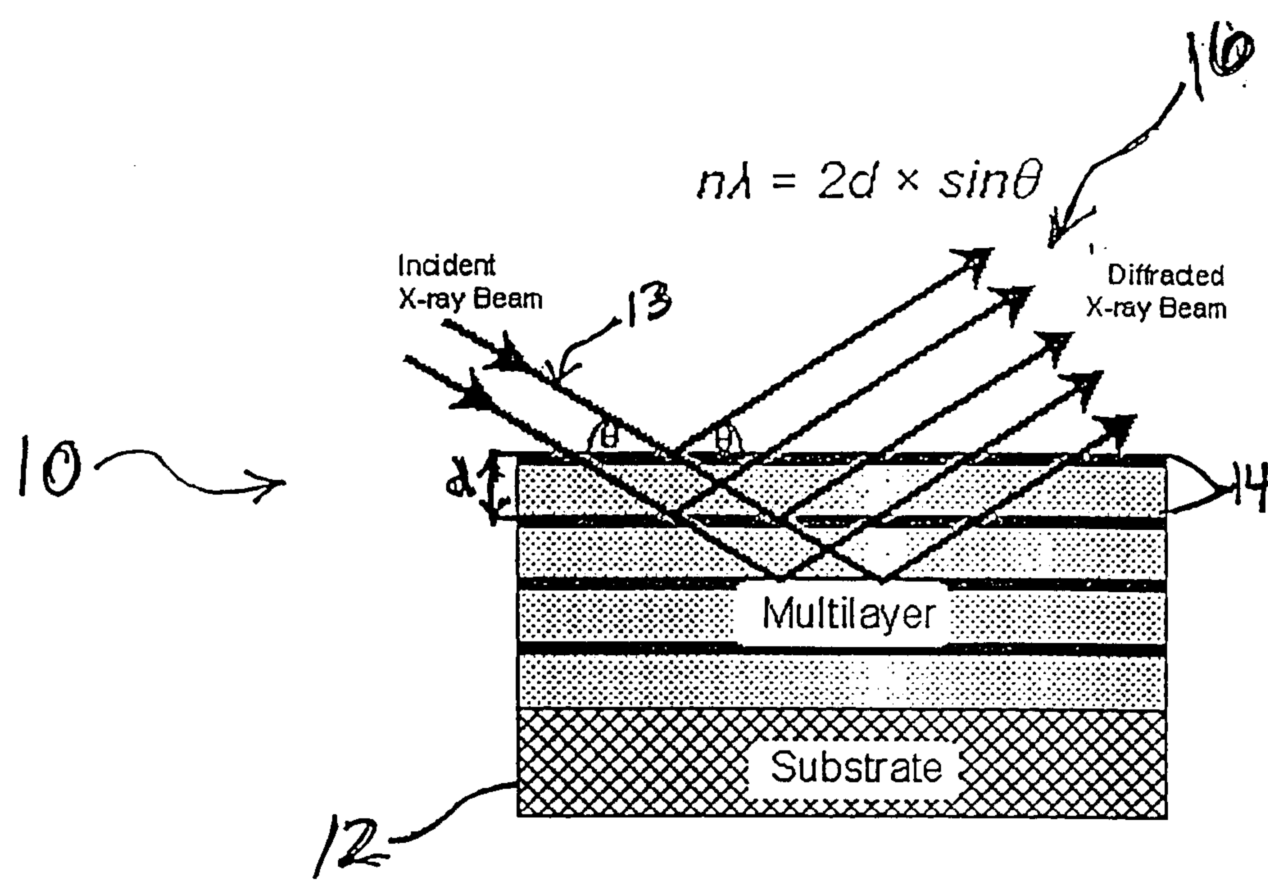
Figure 1. Bragg's reflection of multilayer
