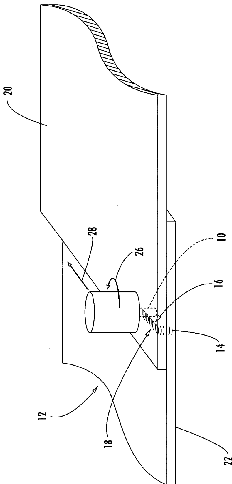
FIG. 1 (PRIOR ART)
