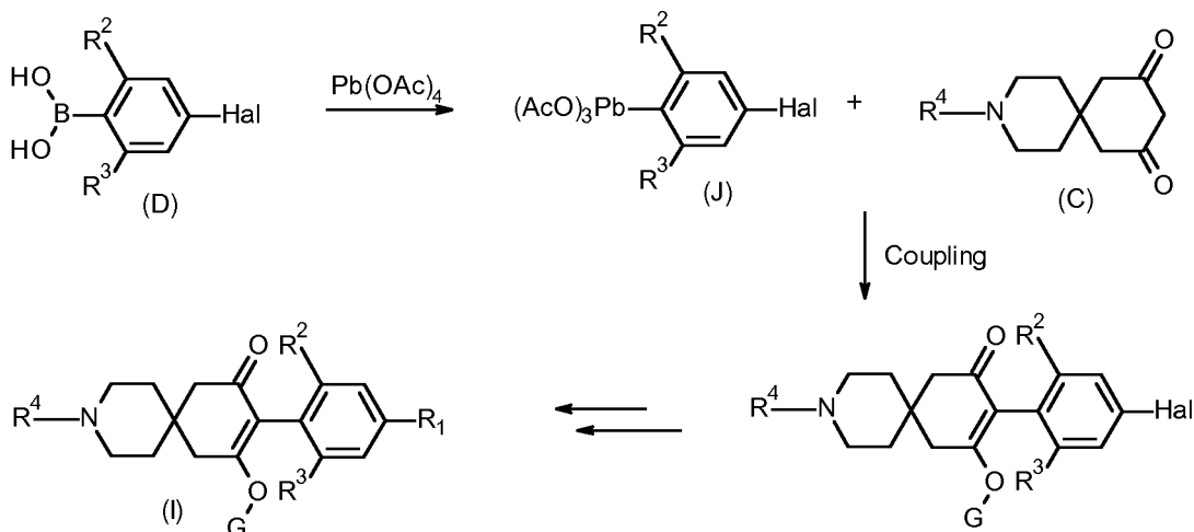
Scheme 6
