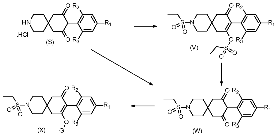
Scheme 11
