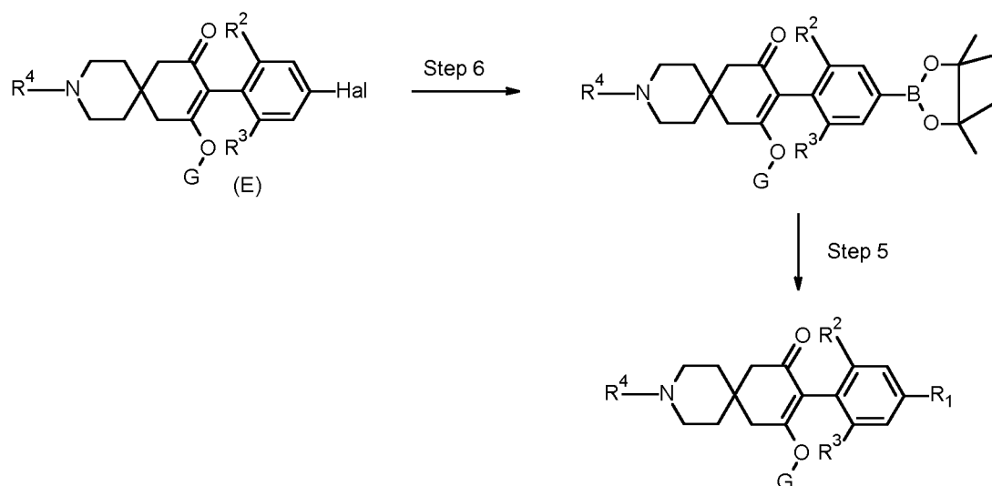
Scheme 4c
