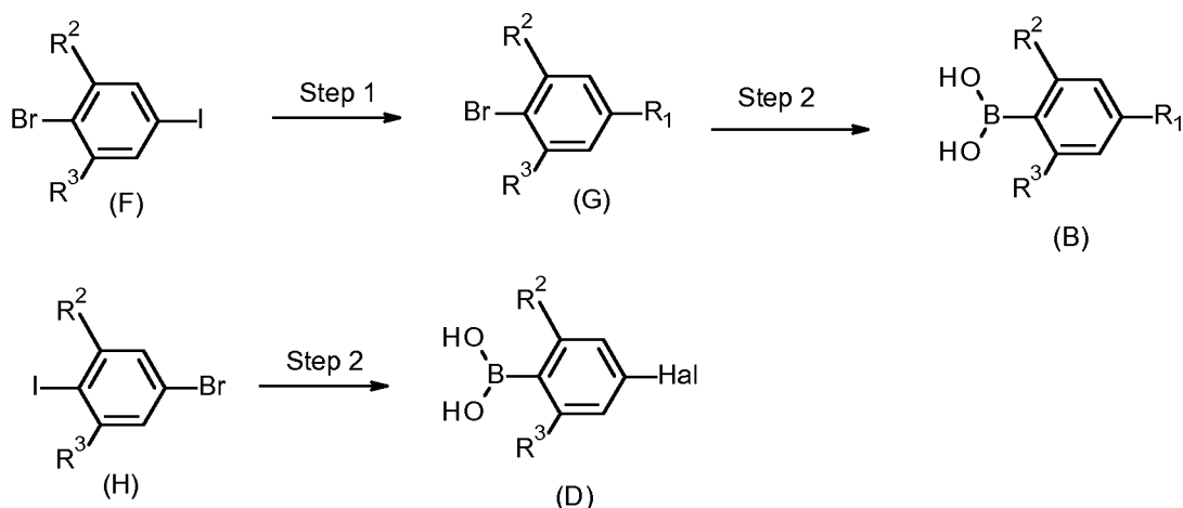
Scheme 5
