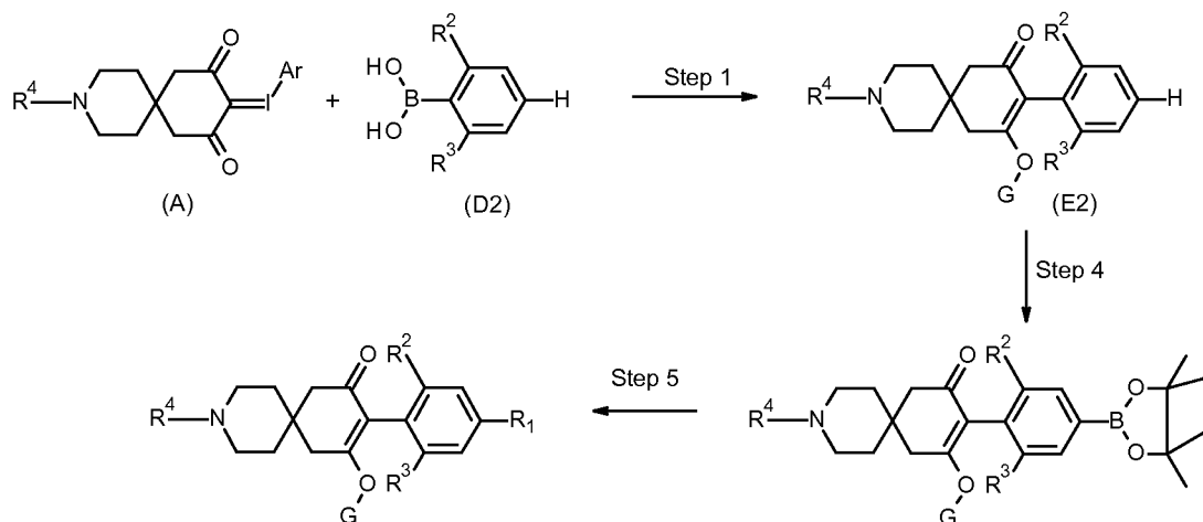
Scheme 4b
