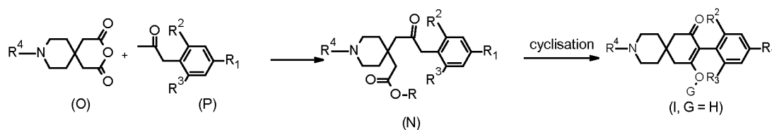
Scheme 9
