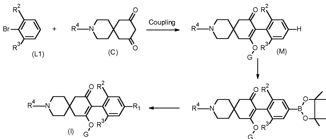
Scheme 8b
