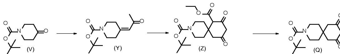
Scheme 13
