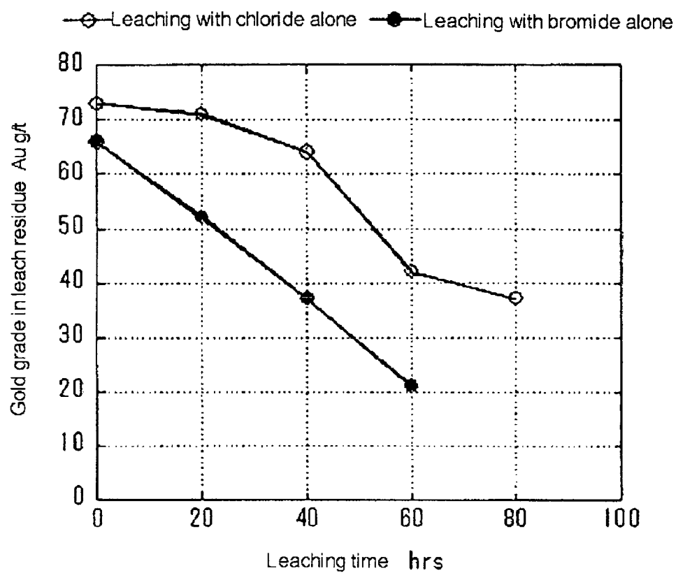
Effects of bromide ions on gold leaching
