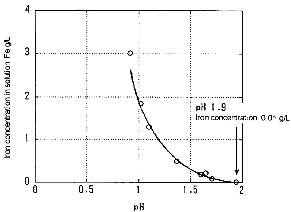
Effects of pH on iron concentration
