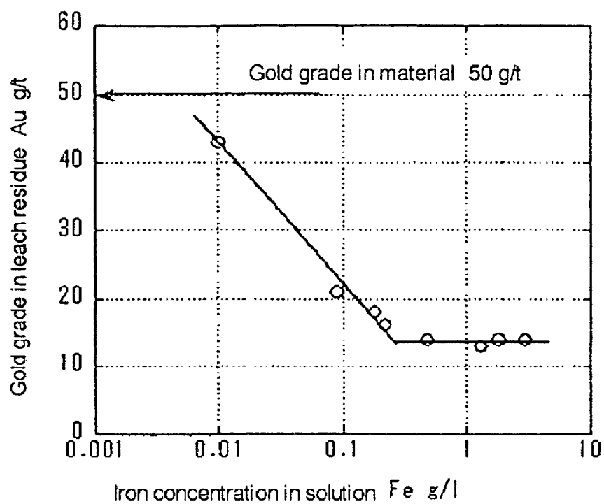
Effects of iron concentration on gold leaching
