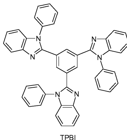
2,2',2''-(1,3,5-benzenetriyl)tris(1-phenyl-1H-benzimidazole) formula ET-2
