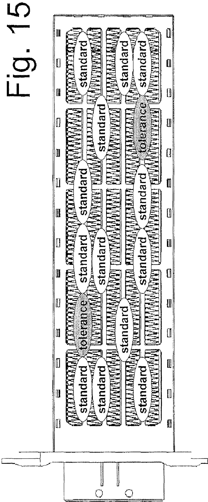
Use of standard PTCs with an R_{25} of 2,61 - 2,90 Ohm
