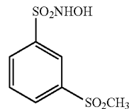
(2) N-Hydroxy-3-methanesulfonylbenzene-1-sulfonamide
